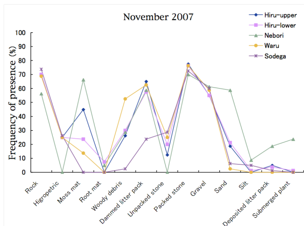
Fig.6 Presence frequency of microhabitat in each stream in June 2006 and November 2007.
