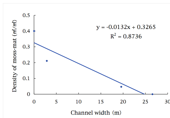
Fig.5 Upper: Relations of the moss-mat density to freeze-thaw index values. Lower: Relations of the moss-mat density to channel width.
