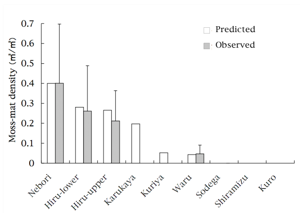
Fig.11 Comparison of predicted and observed values of moss-mat density in the selected streams in the Gamata River basin.
