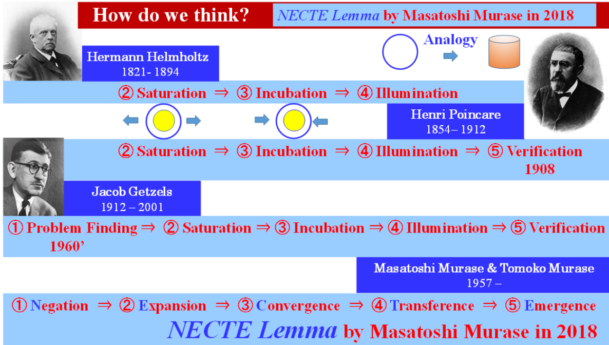
Figure 4: The 5-NECTE principle
