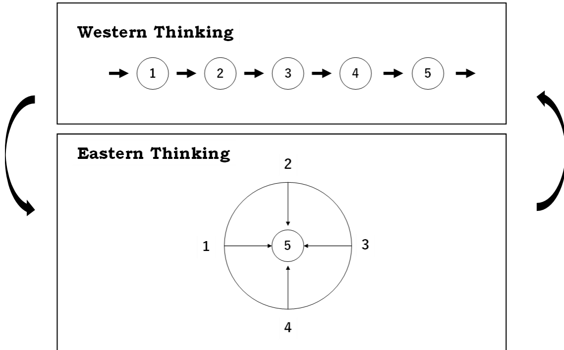
Figure 1: Western thinking and Eastern Thinking
