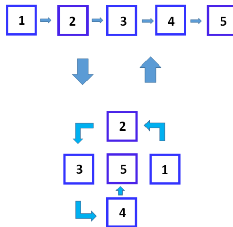
Figure 7: Chain-like relationship and field-like conformation
