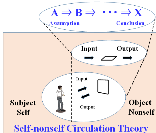
Figure 2: The upper panel shows cause-and-effect relationships at the level of an object. The lower panel indicates the presence of an observer.
