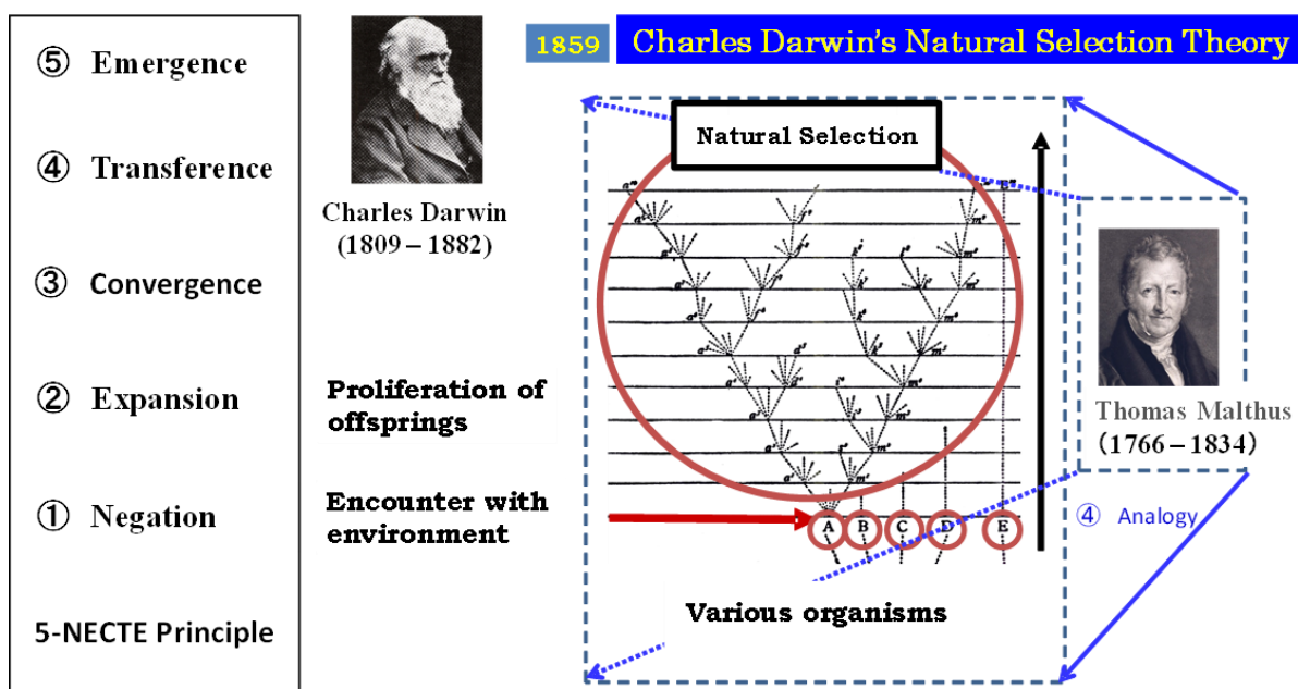
Figure 5: Evolution conducted through NECTE Principle
