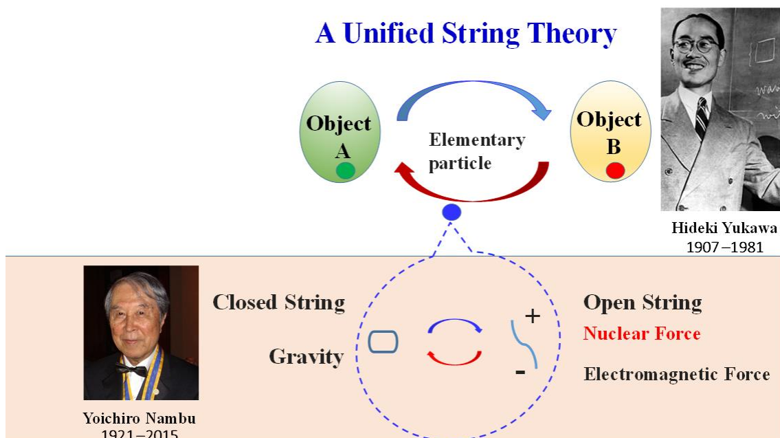
Figure 8: A unified string theory
