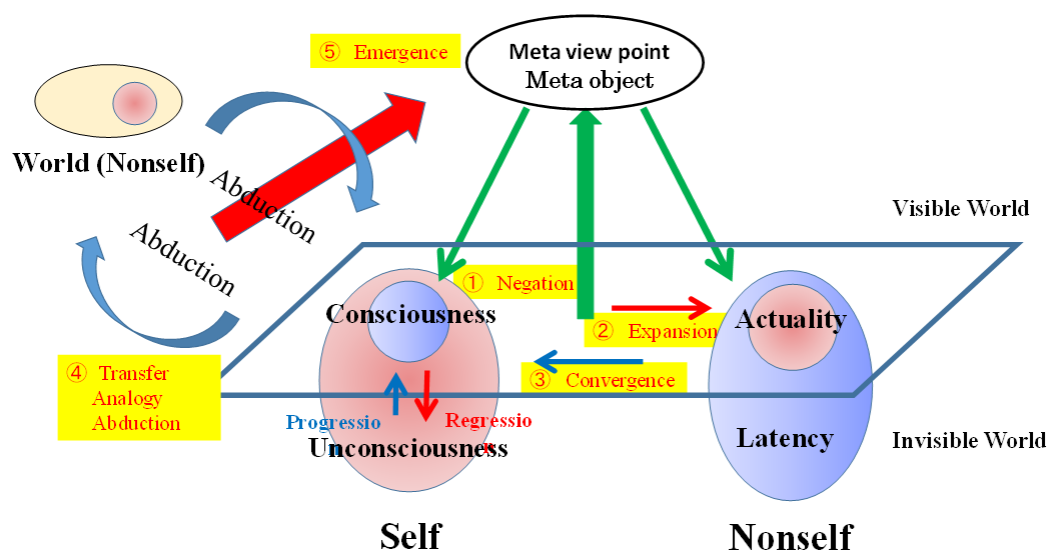
Figure 3: Dynamics of the Self-nonself Circulation Theory
