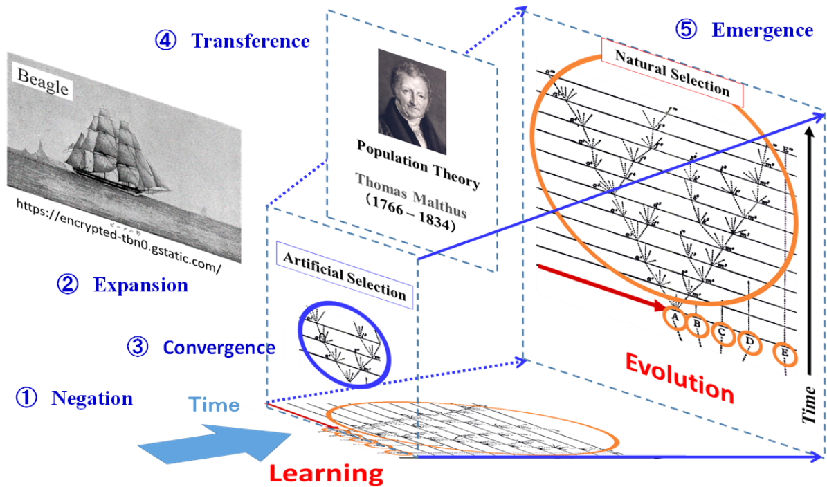
Figure 6: Learning and Evolution conducted through NECTE Principle
