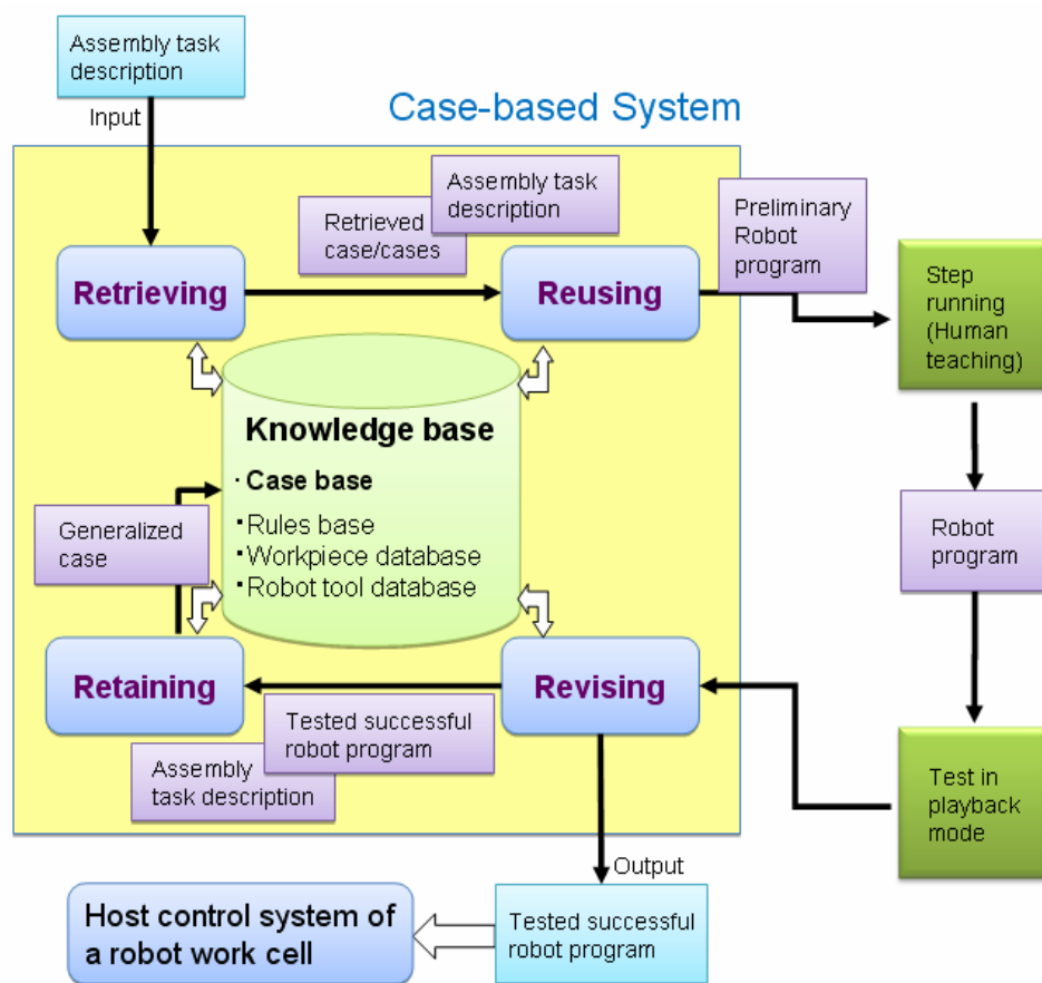
Figure 5.1 The structure of the case-based system.
