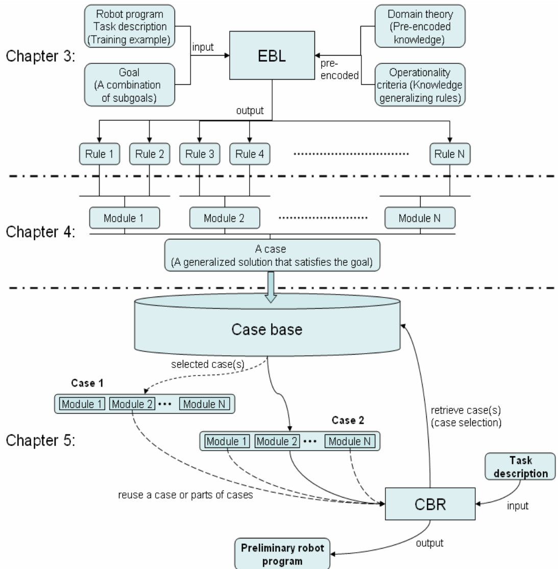
Figure 2.7 The knowledge acquisition and reuse method by integrating EBL and CBR.
