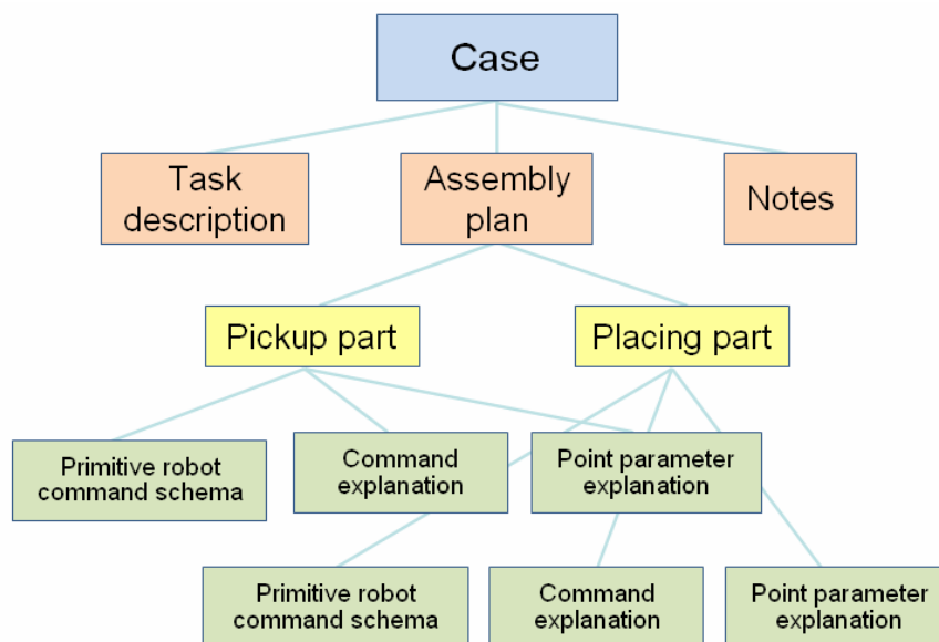
Figure 5.2 The case representation form.
