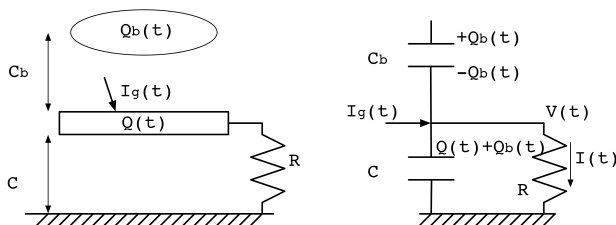
Figure 3: Equivalent circuit.
