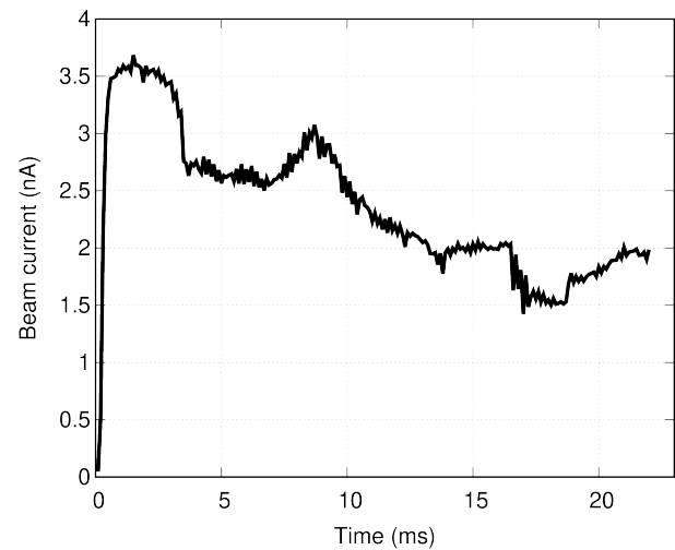
Figure 7: Normalized FAB output waveform, showing the circulating beam current.
