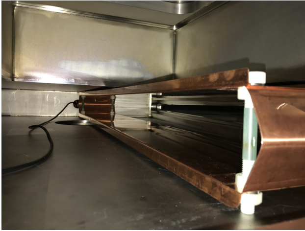
Figure 1: Photo of full-aperture bunch monitor. 100 mm(W)×75 mm(H)×158 mm(L).
