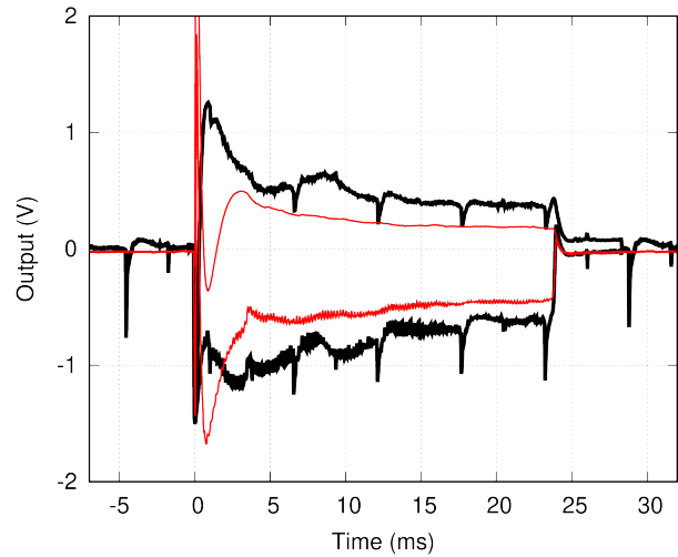
Figure 6: Envelope of the FAB output (black) and normal BMON (red).
