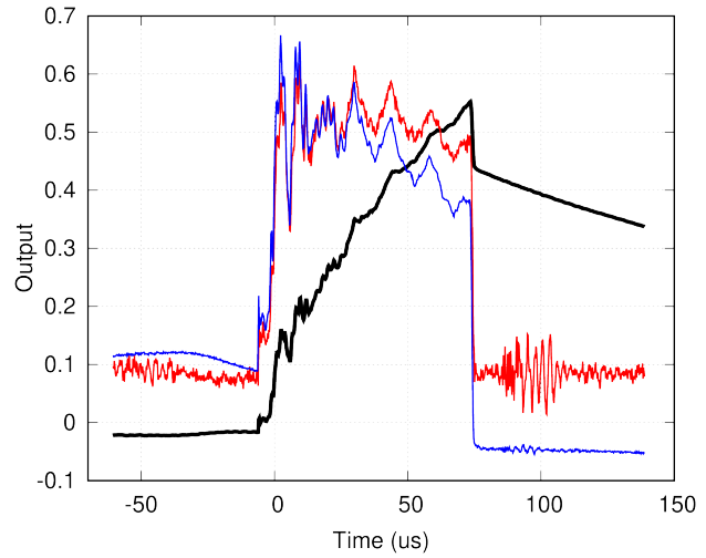
Figure 4: Output from full-aperture bunch monitor (black, in 0.1 V/div), destructive beam current monitor (red, -0.5 mV/div), and current transformer (blue, -5 mV/div).
