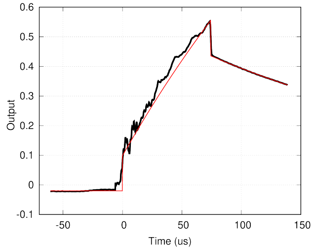
Figure 5: Best fit function (red) for full-aperture bunch monitor output waveform (black) in Fig. 4, based on the assumption of rectangular input.
