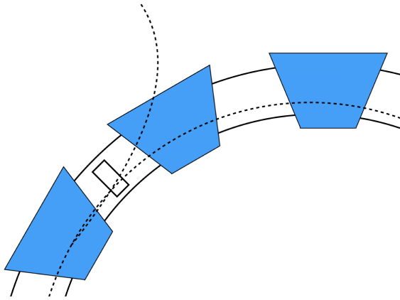
Figure 2: Location to install a new bunch monitor (rectangle symbol). Dashed lines show the trajectory of injected H^- beam and circulating orbit at injection energy.
