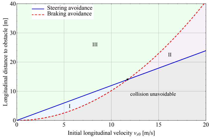
Figure 1.3: Longitudinal distance to obstacle.
