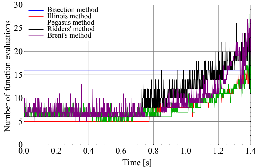
Figure 2.7: Number of function evaluations along the lane change maneuver with \epsilon = 10^{-6} for different root finding methods.
