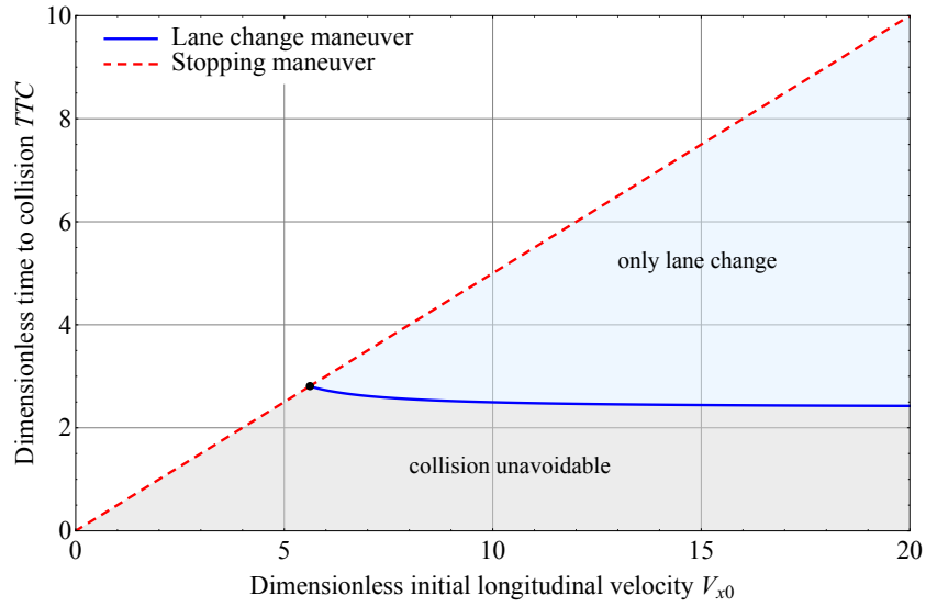
Figure 4.5: Decision-making diagram based on the dimensionless time to collision.
