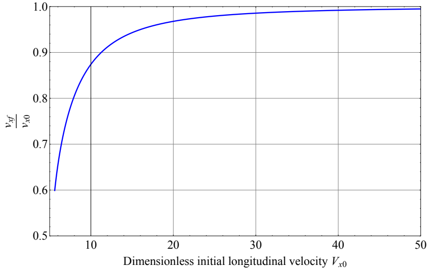
Figure 4.6: Final-to-initial longitudinal vehicle velocity ratio.
