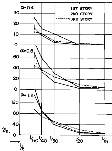
Fig. 11. Basic Response Diagram of Total Dissipated Hysteretic Energy Factor-El Centro N-S, Structural Model B_I .
