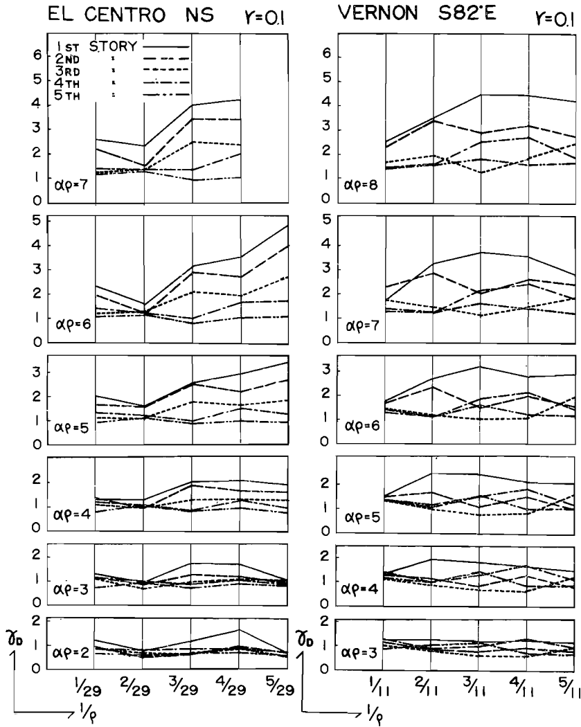
Fig. 17. Basic Response Diagrams of Maximum Ductility Factor-El Centro N-S and Vernon S82°E, Structural Model C_{II} , Rigidity Ratio r=0.1 .
