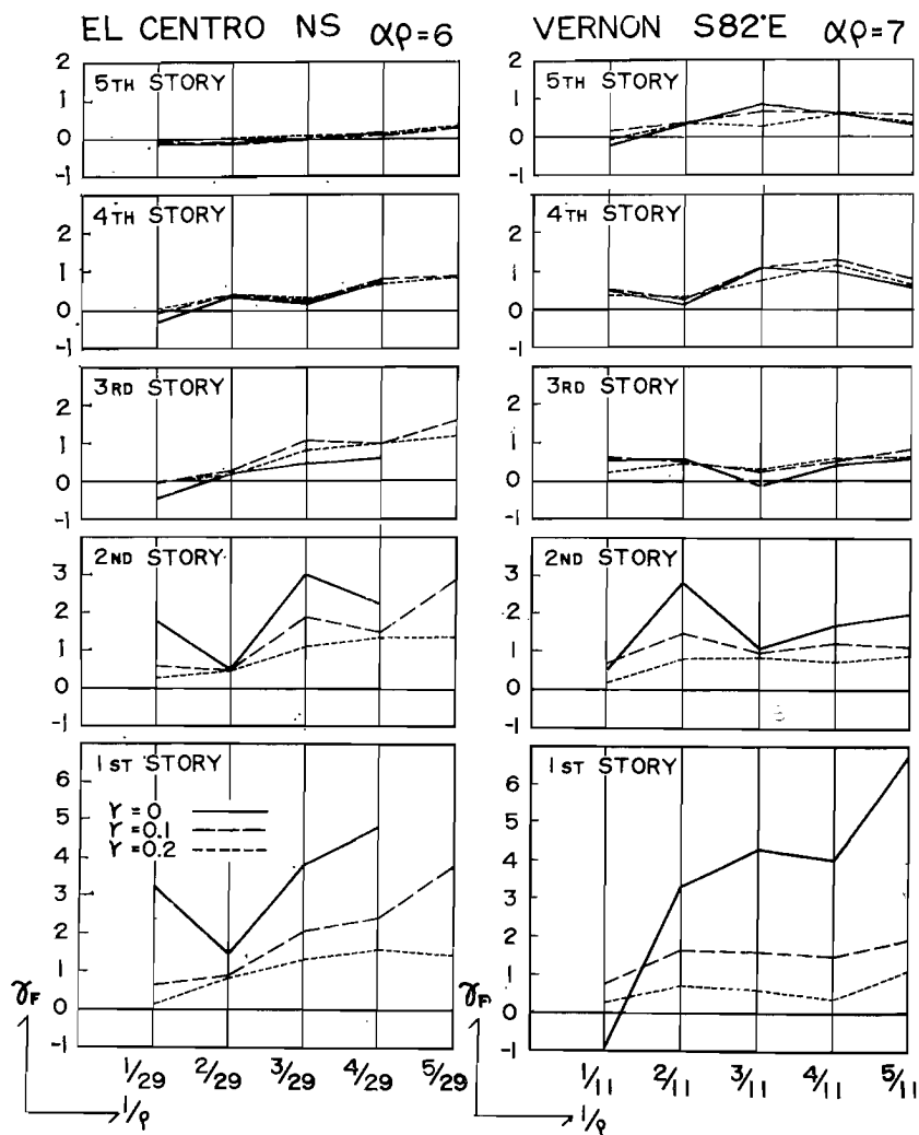
Fig. 20. Response Diagrams of Offset Factor-El Centro N-S and Vernon S82°E, Structural Model C_{II} .
