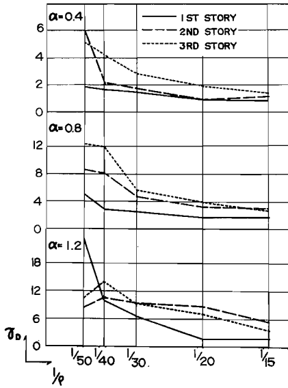
Fig. 9. Basic Response Diagram of Maximum Ductility Factor-El Centro N-S, Structural Model C_I .
