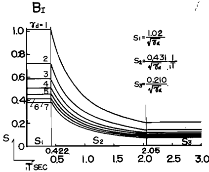
Fig. 36. Simplified Base Shear Coefficient-El Centro N-S, Structural Model B_I .
