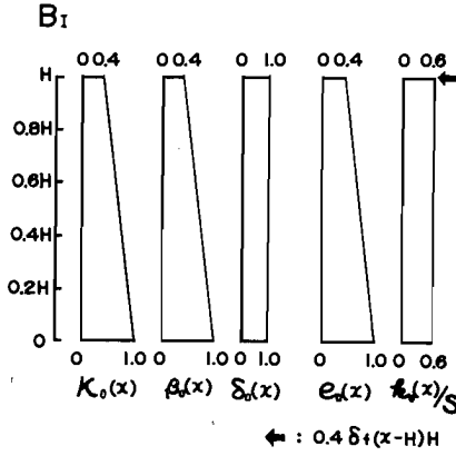
Fig. 30. Optimum Distributions of Dynamic Characteristics and Lateral Force Coefficients-Structural Model B_I .
