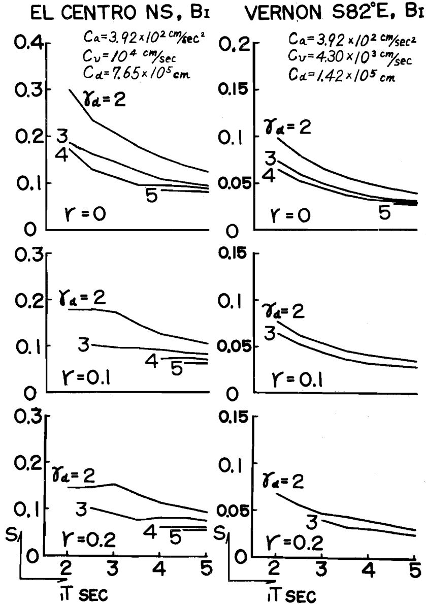
Fig. 28. Base Shear Coefficients for Hypothetical Earthquake Excitation Groups- El Centro N-S and Vernon S82°E, Structural Model B I .
