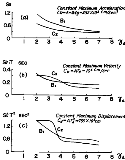
Fig. 22. Base Shear Coefficients s_{\bar{a}} , s_{\bar{v}} and s_{\bar{d}} Based on Maximum Ductility Factor in 15 \leq \rho \leq 50 —El Centro N-S, Structural Models B_I and C_{II} .
