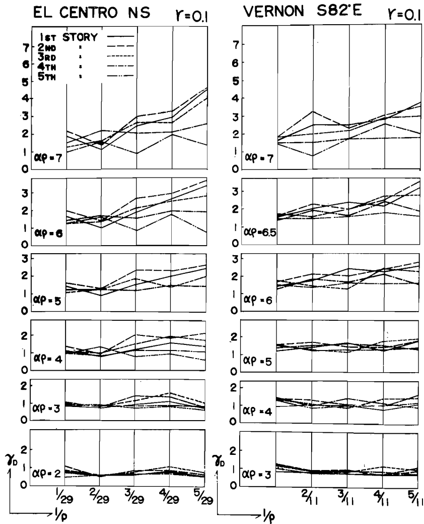
Fig. 14. Basic Response Diagrams of Maximum Ductility Fatcor-El Centro N-S and Vernon S82°E, Structural Model B_1 , Rigidity Ratio r=0.1 .
