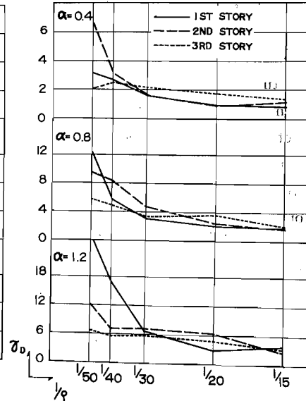
Fig. 8. Basic Response Diagram of Maximum Ductility Factor-El Centro N-S, Structural Model B_I .
