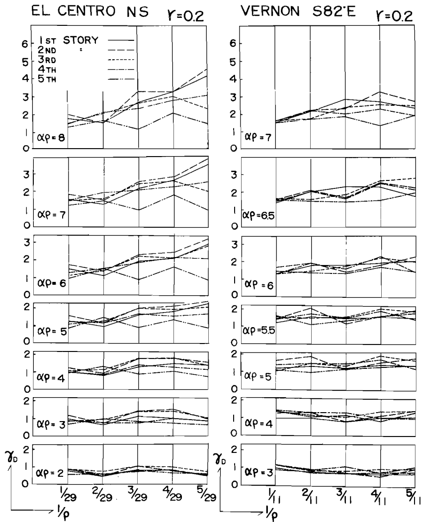
Fig. 15. Basic Response Diagrams of Maximum Ductility Factor-El Centro N-S and Vernon S82°E, Structural Model B_7 , Rigidity Ratio \gamma=0.2 .
