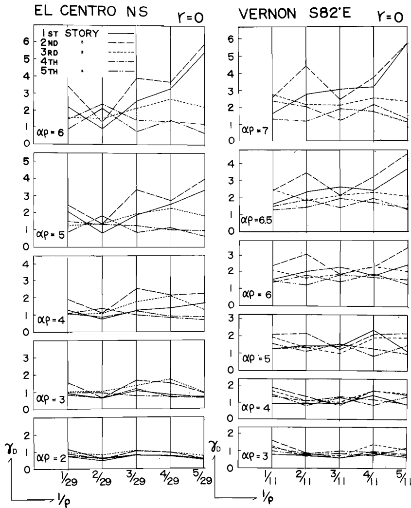
Fig. 13. Basic Response Diagrams of Maximum Ductility Factor-El Centro N-S and Vernon S82°E, Structural Model B_I , Rigidity Ratio r=0 .
