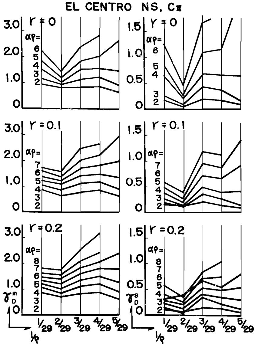
Fig. 27. Mean and Standard Deviation of Standardized Maximum Ductility Factor-El Centro N-S, Structural Model C_{II} .
