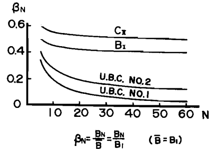
Fig. 33. Distribution Coefficient of Strength at Top Story.
