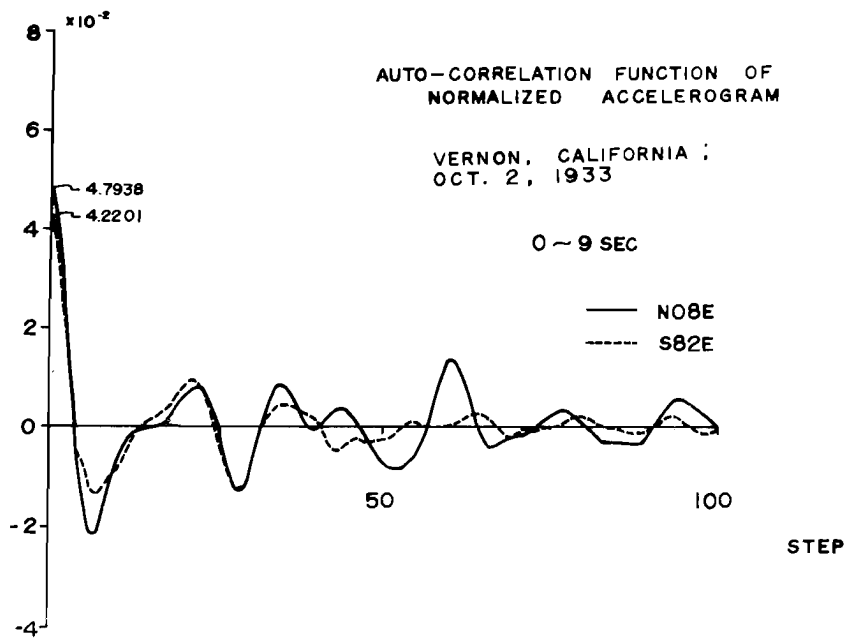
Fig. 5. (a) Autocorrelation Functions of Normalized Accelerograms of Vernon Earthquake, 0~9 sec.
