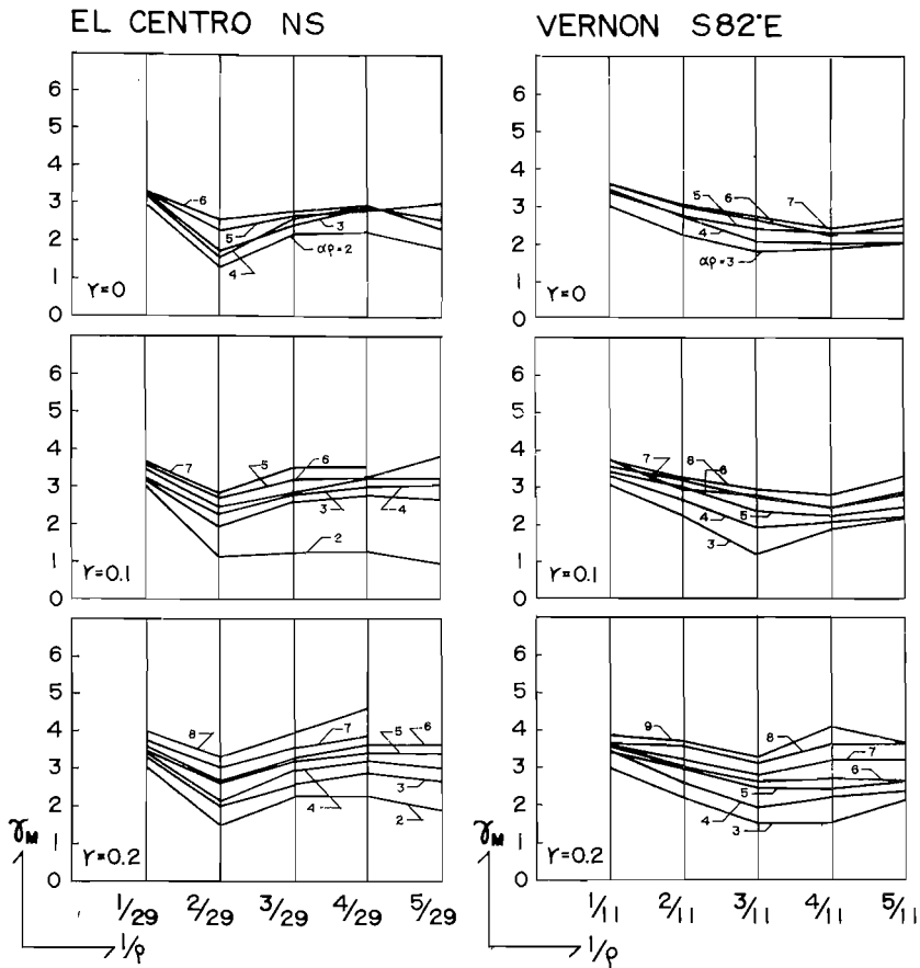
Fig. 21. Response Diagrams of Maximum Overturing Moment Factor-El Centro N-S and Vernon S82°E, Structural Model C_{II} .
