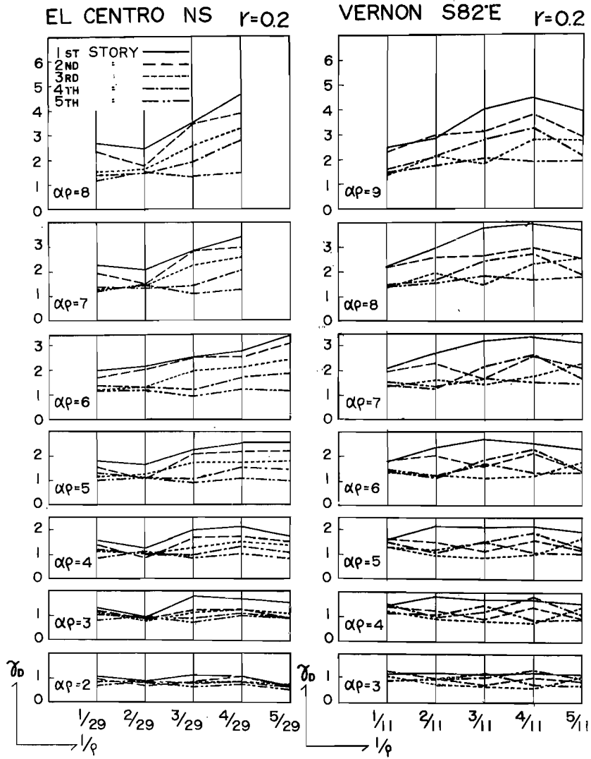
Fig. 18. Basic Response Diagrams of Maximum Ductility Factor-El Centro N-S and Vernon S82°E, Structural Model C_{II} , Rigidity Ratio r=0.2 .
