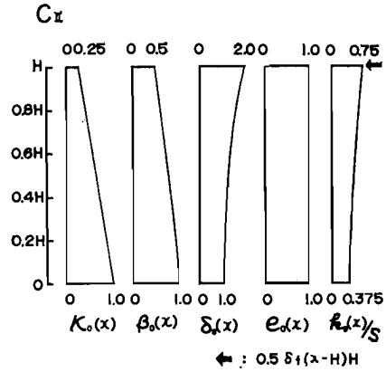
Fig. 31. Optimum Distributions of Dynamic Characteristics and Lateral Force Coefficients-Structural Model C_{II} .
