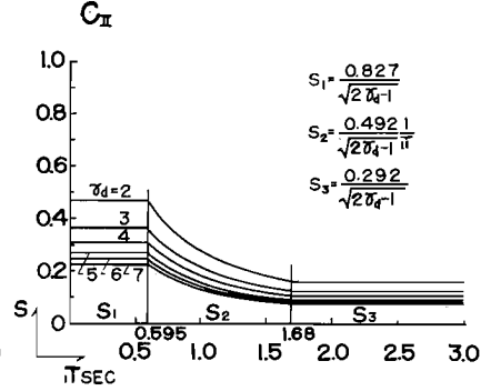
Fig. 35. Simplified Base Shear Coefficient-El Centro N-S, Structural Model C_{II} .
