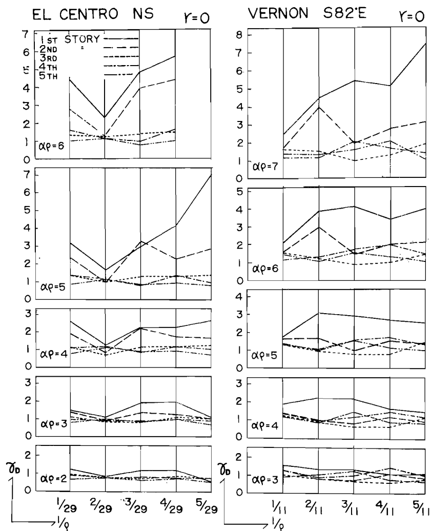
Fig. 16. Basic Response Diagrams of Maximum Ductility Factor-El Centro N-S and Vernon S82°E, Structural Model C_{11} , Rigidity Ratio r=0 .
