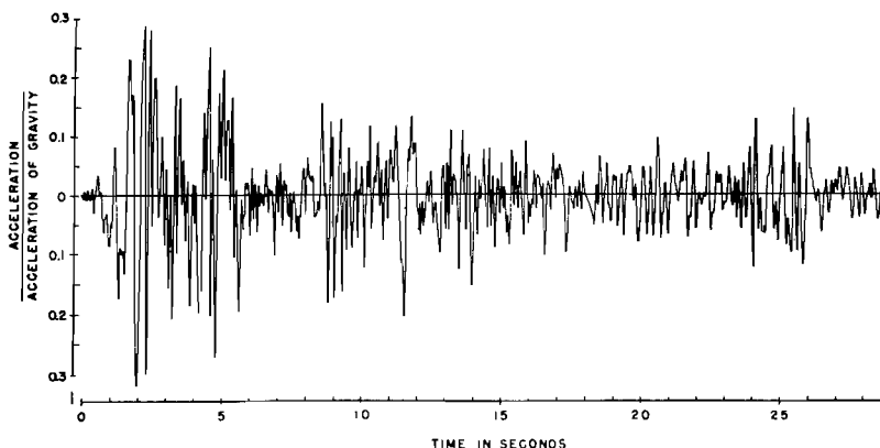
Fig. 1. (a) Accelerogram for El Centro, California, May 18, 1940, N-S Component.
