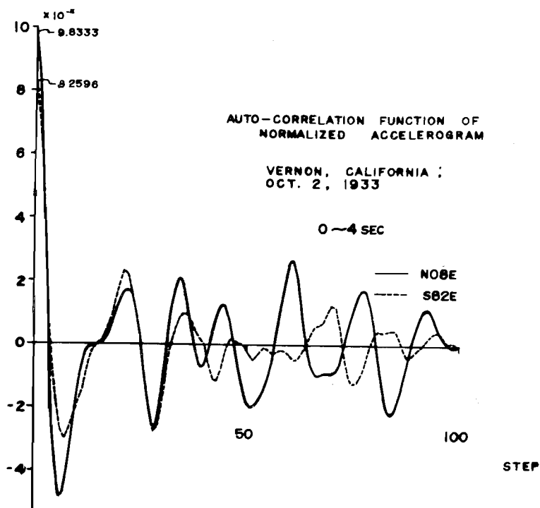
Fig. 5. (b) Autocorrelation Functions of Normalized Accelerograms of Vernon Earthquake, 0~4 sec.
