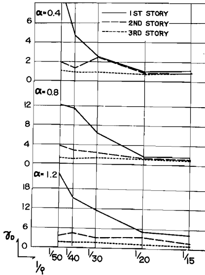
Fig. 7. Basic Response Diagram of Maximum Ductility Factor-El Centro N-S, Structural Model A_I = A_{II} .
