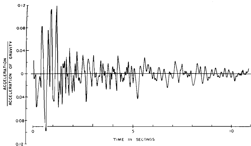
Fig. 4. (a) Accelerogram for Vernon, California, Oct. 2, 1933, S82°E Component.
