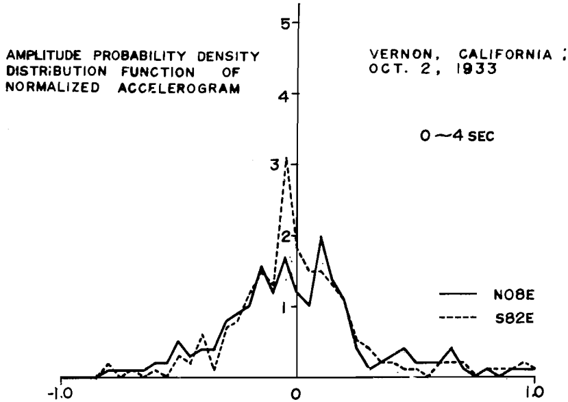
Fig. 6. (b) Amplitude Probability Density Distribution Functions of Vernon Earthquake, 0~4 sec.
