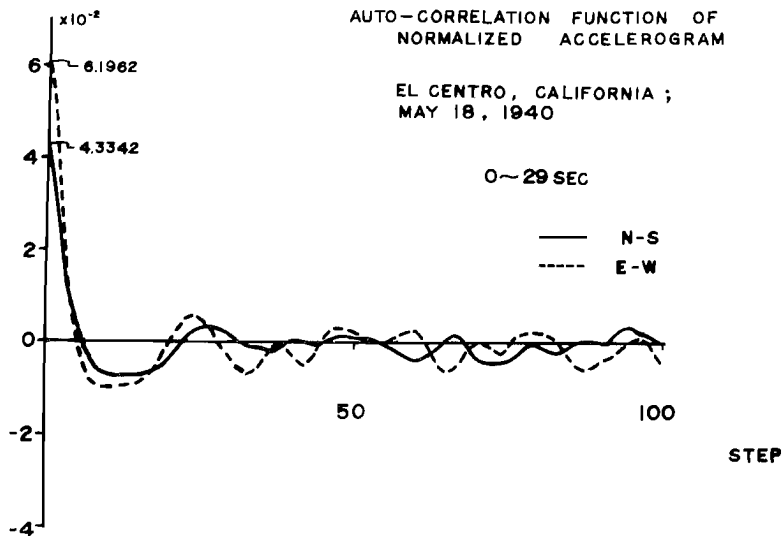
Fig. 2. Autocorrelation Functions of Normalized Accelerograms of El Centro Earthquake.
