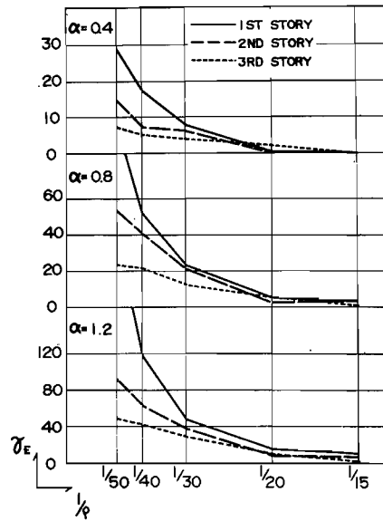
Fig. 12. Basic Response Diagram of Total Dissipated Hysteretic Energy Factor-El Centro N-S, Structural Model C_{II} .
