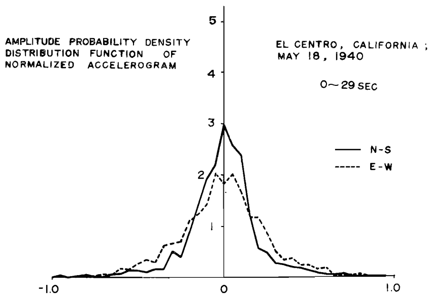
Fig. 3. Amplitude Probability Density Distribution Functions of Normalized Accelerograms of El Centro Earthquake.
