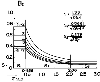
Fig. 34. Simplified Base Shear Coefficient-El Centro N-S, Structural Model B_I .
