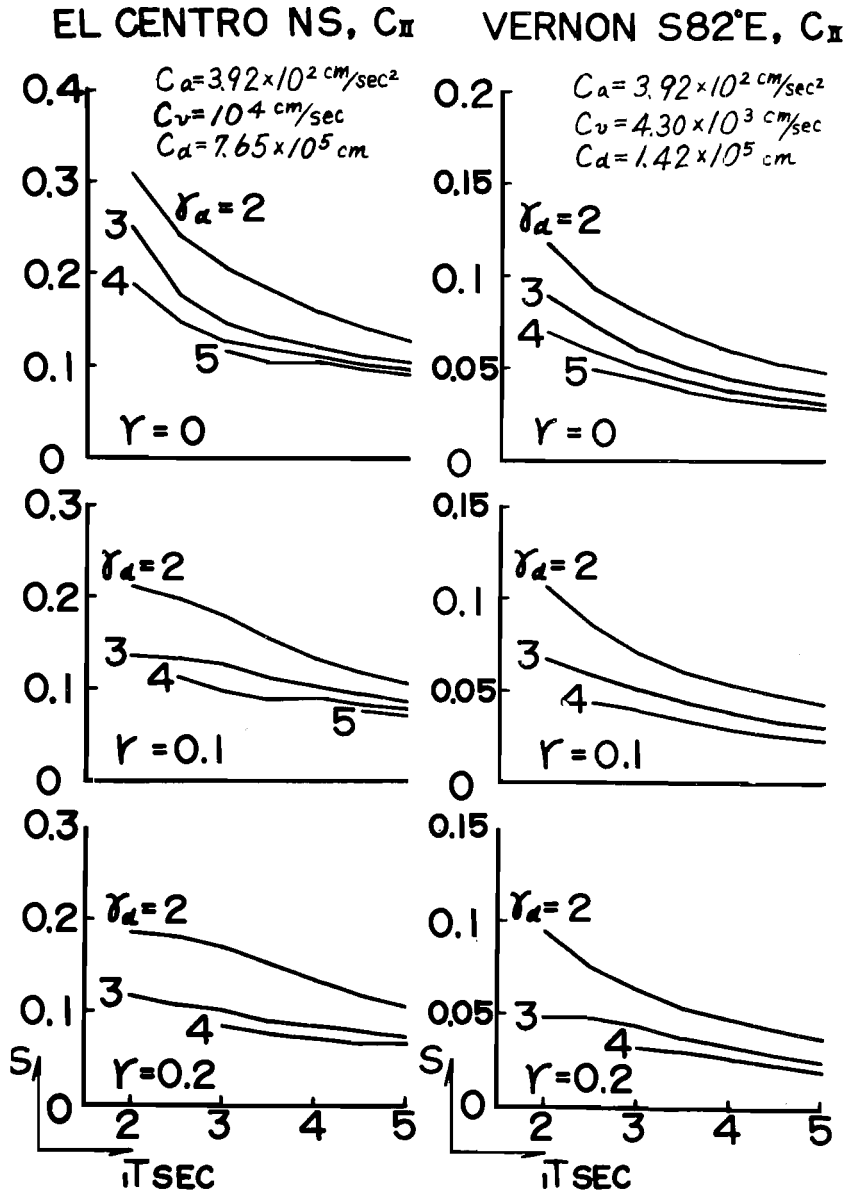
Fig. 29. Base Shear Coefficients for Hypothetical Earthquake Excitation Groups- El Centro N-S and Vernon S82°E, Structural Model C_{II} .
