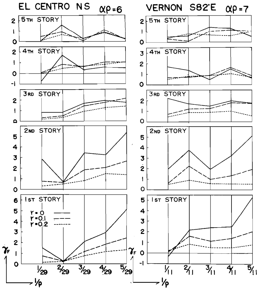
Fig. 19. Response Diagrams of Offset Factor-El Centro N-S and Vernon S82°E, Structural Model B_1 .
