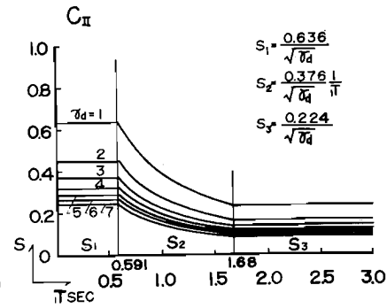
Fig. 37. Simplified Base Shear Coefficient-El Centro N-S, Structural Model C_{II} .
