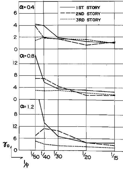
Fig. 10. Basic Response Diagram of Maximum Ductility Factor-El Centro N-S, Structural Model C_{II} .
