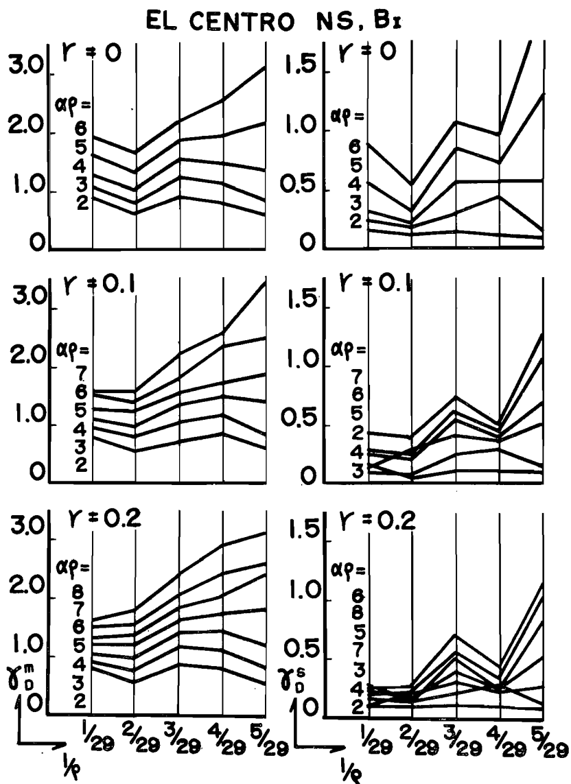
Fig. 26. Mean and Standard Deviation of Standardized Maximum Ductility Factor-El Centro N-S, Structural Model B 1 .
