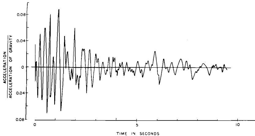
Fig. 4. (b) Accelerogram for Vernon, California, Oct. 2, 1933, N08°E Component.
