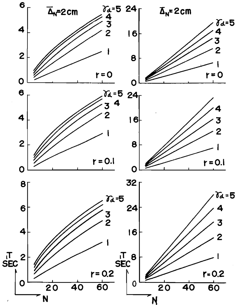
Fig. 39. Fundamental Natural Period for \bar{A}_N=2 cm-El Centro N-S and Vernon S82°E, Structural Model C_{II} .
