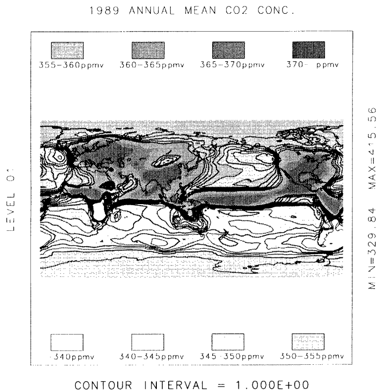
Fig. 2 Annual mean simulated CO 2 distribution in the lowest layer
