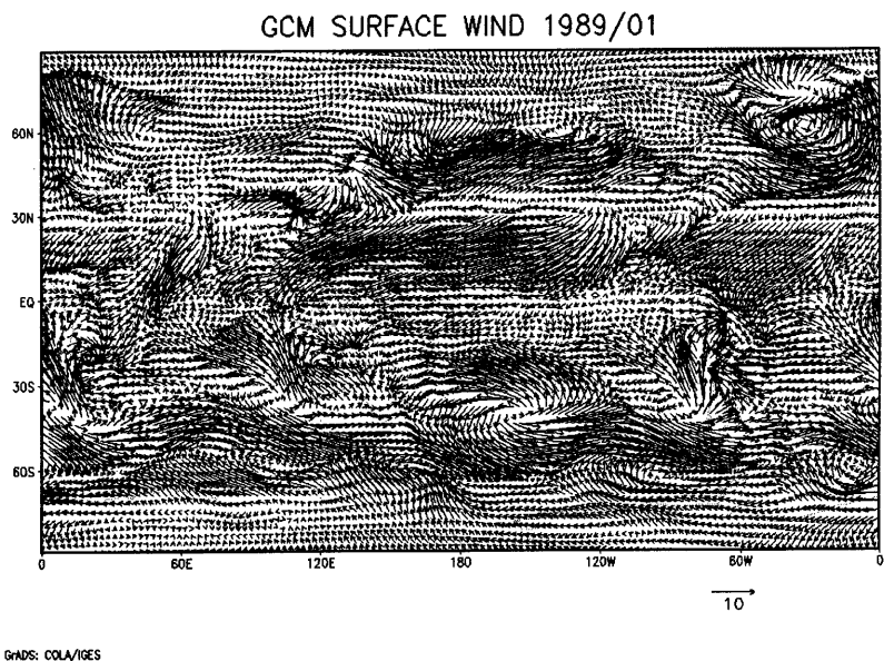
Fig. 9 1989/01 monthly wind of ECMWF/TOGA and GCM
