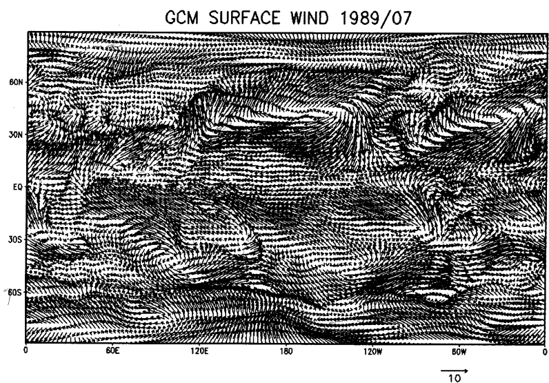
Fig. 10 1989/07 monthly wind of ECMWF/TOGA and GCM
