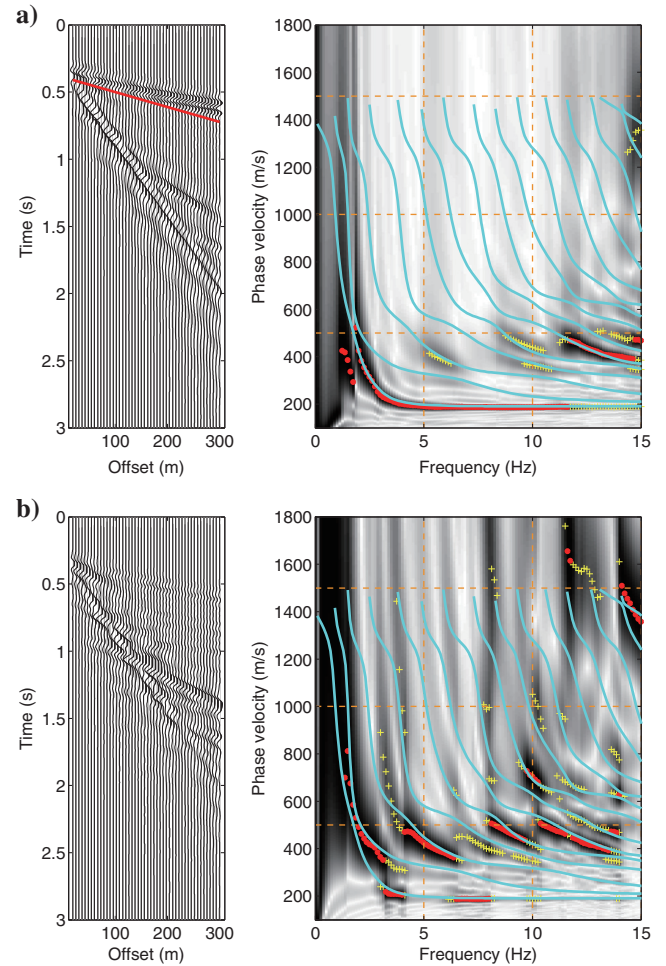
Figure 4. The 30-Hz low-pass-filtered synthesized waveforms and dispersion images for (a) vertical and (b) horizontal component data when the explosive source is located at an 8-m depth in model A. The body waves of the vertical component data are muted (red line). The red circles and yellow crosses are phase velocities with absolute maxima and relative maxima for each frequency, respectively. The cyan lines are theoretical dispersion curves.
