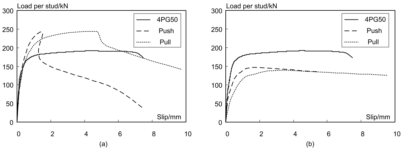
Fig. 6.20 Comparison of load-slip curves of stud: (a) Specimen ‘C-4PG50’; (b) Specimen ‘C-9PG50’
