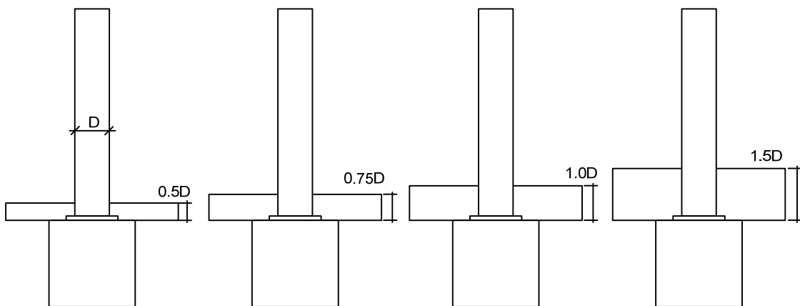
Fig. 3. 26 Shallowly embedded column base with different thickness of slab
