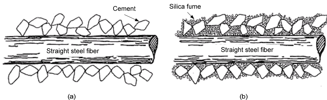
Fig. 4. 6 Straight fibers embedded in different paste:
