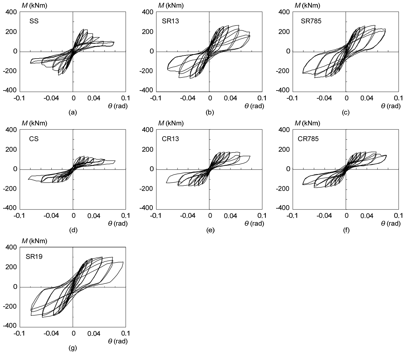
Fig. 4. 15 Moment versus rotation relationships: (a) SS; (b) SR13; (c) SR785; (d) CS; (e) CR13; (f) CR785; and (g) SR19
