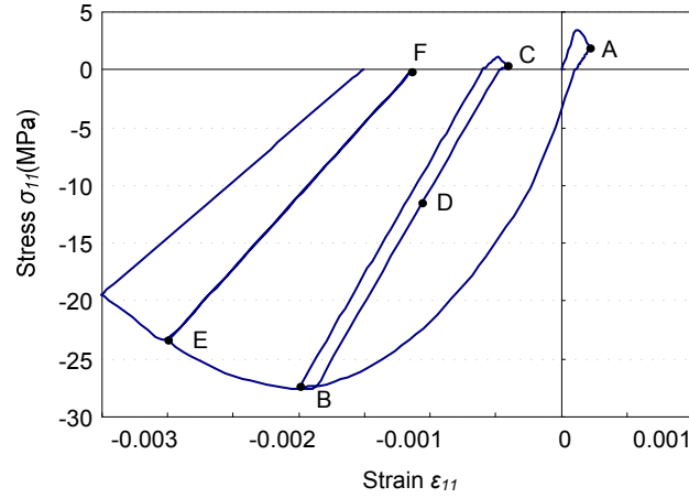
Fig. 3. 15 Numerical solution for full cyclic loading (path: O-A-B-C-D-E-F)
