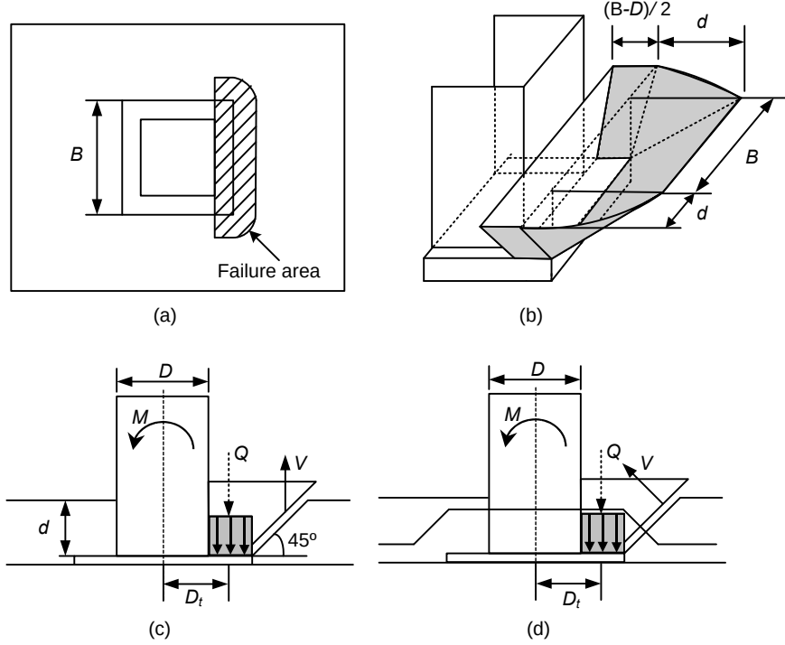
Fig. 2. 9 Model of punching shear mechanism in concrete slab: (a) plan view; (b) punching-shear surface; (c) evaluation model for floor slab; and (d) evaluation model for strengthened floor slab
