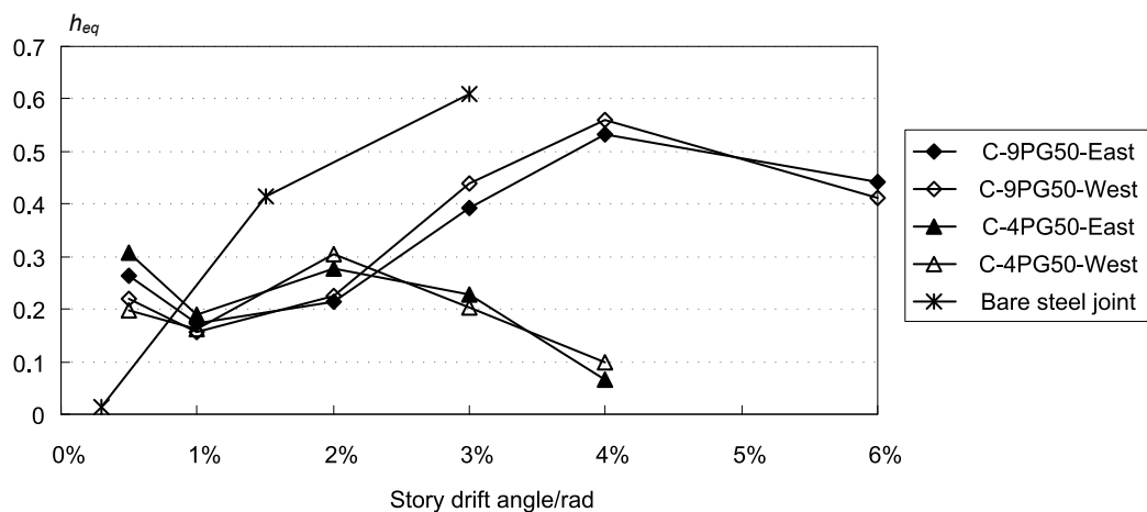
Fig. 6. 16 Equivalent viscous damping coefficient
