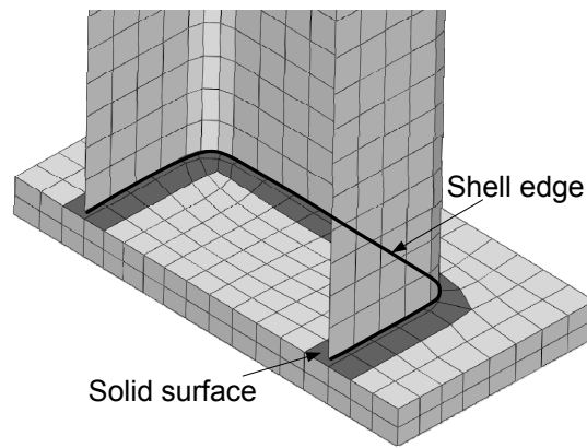
Fig. 3. 8 Shell-to-solid coupling between the column and baseplate
