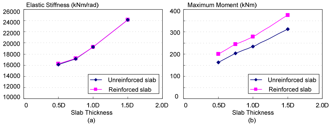
Fig. 3. 27 Influence of axial force ratio: (a) elastic stiffness; (b) maximum moment
