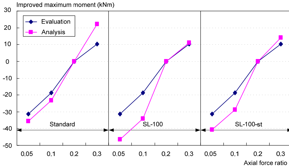
Fig. 3. 39 Comparisons of increased maximum moment with respect to axial force ratio
