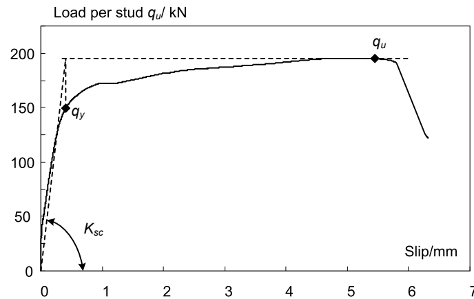
Fig. 5. 9 Definition of slip stiffness, yield load and ultimate load
