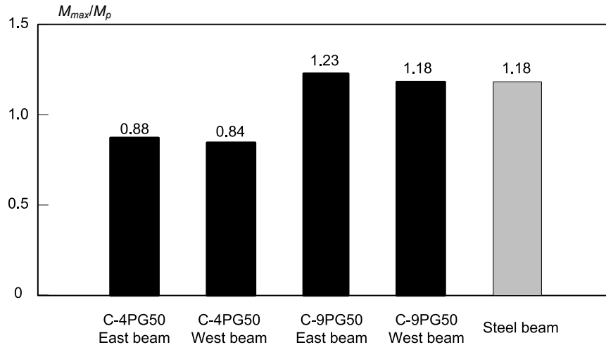
Fig. 6. 15 Normalized maximum moment
