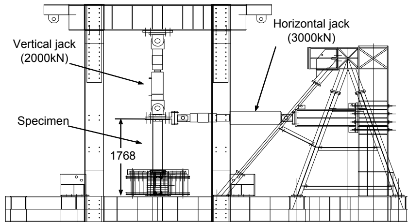
Fig. 4. 14 Elevation of the loading system (unit: mm)
