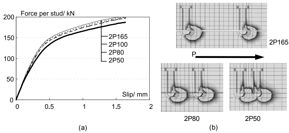
Fig. 5. 25 Effects of the longitudinal spacing: (a) Load –slip curves; (b) compressive strain contour of the slabs
