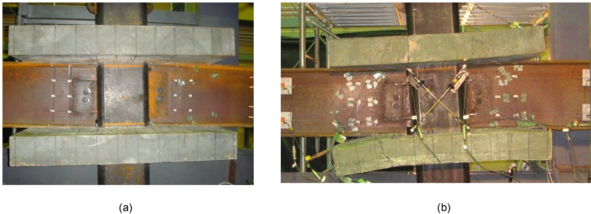
Fig. 6. 17 Failure of specimens: (a) stud fracture (Specimen ‘C-4PG50’); (b) combination of slab fracture and beam yield (Specimen ‘C-9PG50’)
