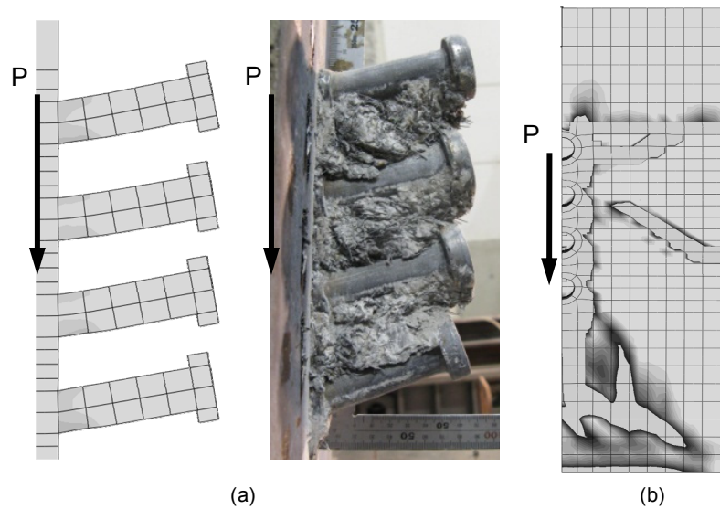
Fig. 5. 24 Comparison of numerical and experimental behavior of specimen failed in the slab: (a) deformation of studs; (b) splitting of the slab
