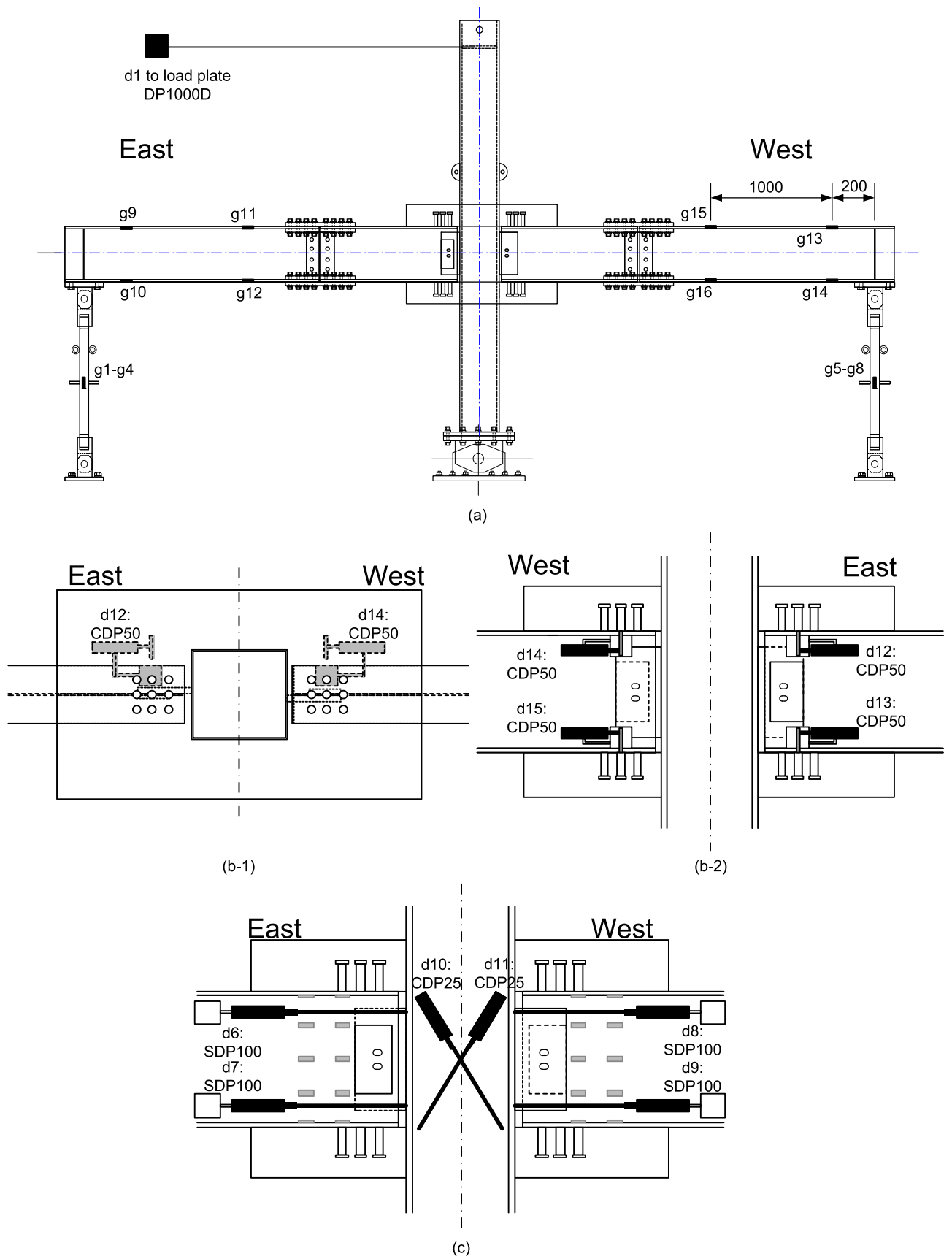
Fig. 6.9 Layout of LVDT: (a) globe view; (b-1) plane view for slip measure; (b-2) side view for slip measurement; and (c) side view for the rotation of beam and panel zone (unit:mm)
