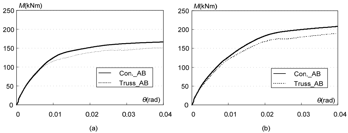
Fig. 3. 22 Comparisons between different models of anchor bolts: (a) SL-100; (b) SL-100-st
