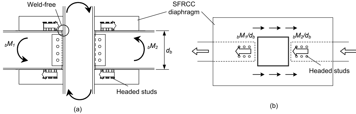
Fig. 6. 4 Proposed beam-column connection: (a) elevation view; (b) plane-view
