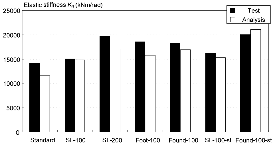
Fig. 3. 18 Comparison of elastic stiffness between test and analysis
