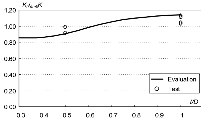
Fig. 2. 21 The ratio of elastic stiffness between shallowly embedded and embedded column base
