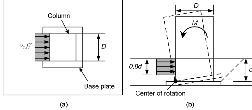
Fig. 2. 8 Model of compressive mechanism in concrete slab: (a) plan view; (b) elevation view
