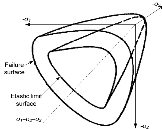
Fig. 3. 5 Schematic representation of elastic limit and failure surfaces of concrete in three-dimensional stress space (Chen, 1982)
