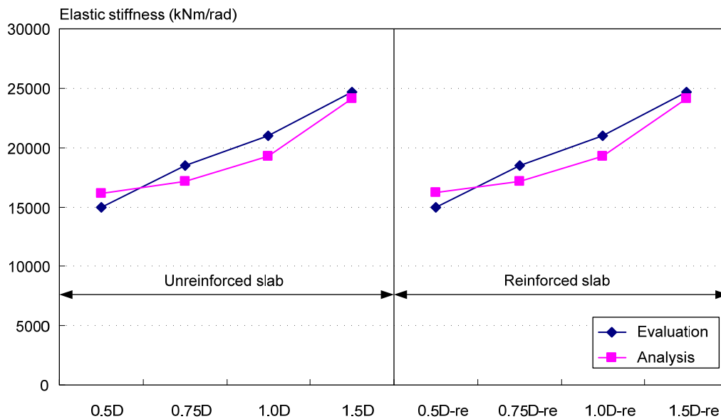
Fig. 3. 32 Comparisons of predicted elastic stiffness with respect to slab thickness
