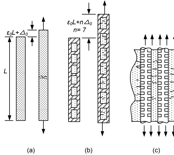
Fig. 4. 8 Tensile deformation of bar of different material:
