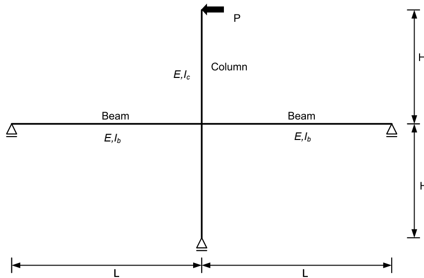
Fig. 6. 14 Cruciform frame model
