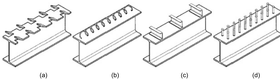
Fig. 5. 1 Historical development of shear connectors:
