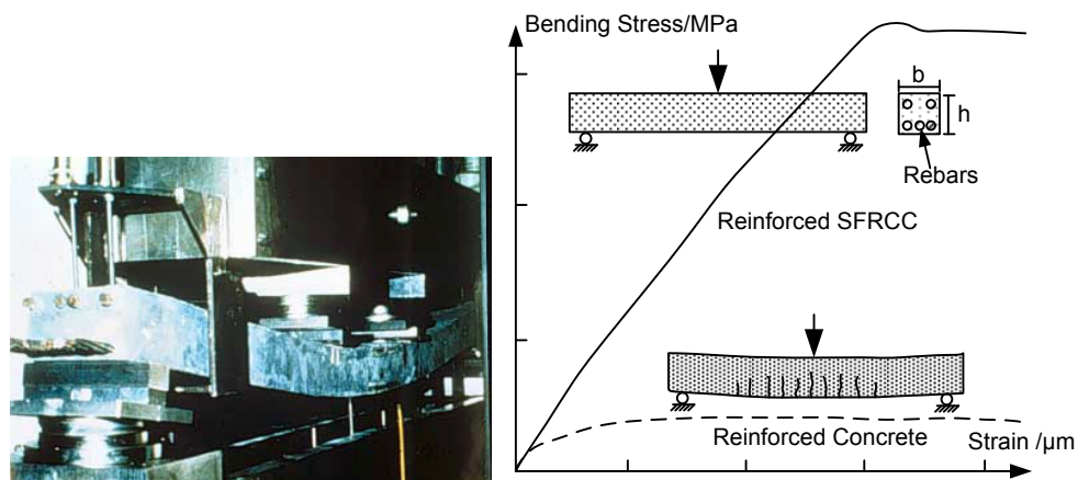
Fig. 4. 2 Behavior of reinforced SFRCC beam and reinforced concrete beam in bending (Cross section 50x50 mm, span 447 mm, bending stress is M/(1/6bh^2) ) (Bache 1987)
