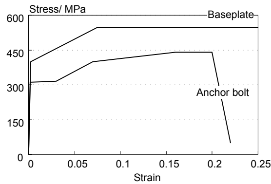
Fig. 3. 11 Material Property for base plates, columns and anchor bolts
