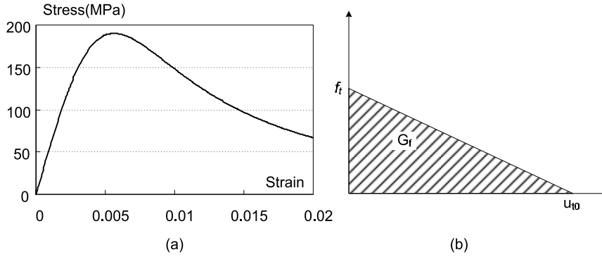
Fig. 5. 20 Material Property: (a) compression; (b) tension
