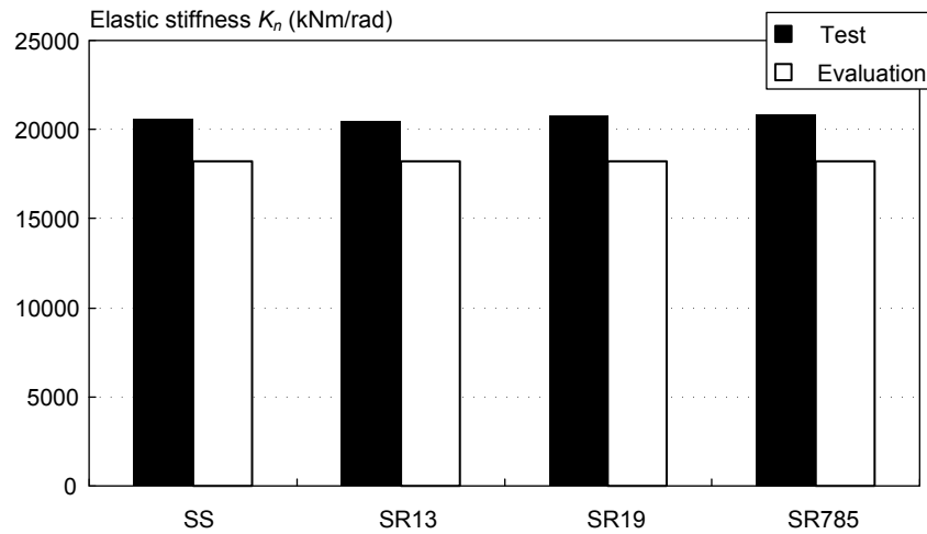
Fig.4.26 Elastic stiffness of specimen
