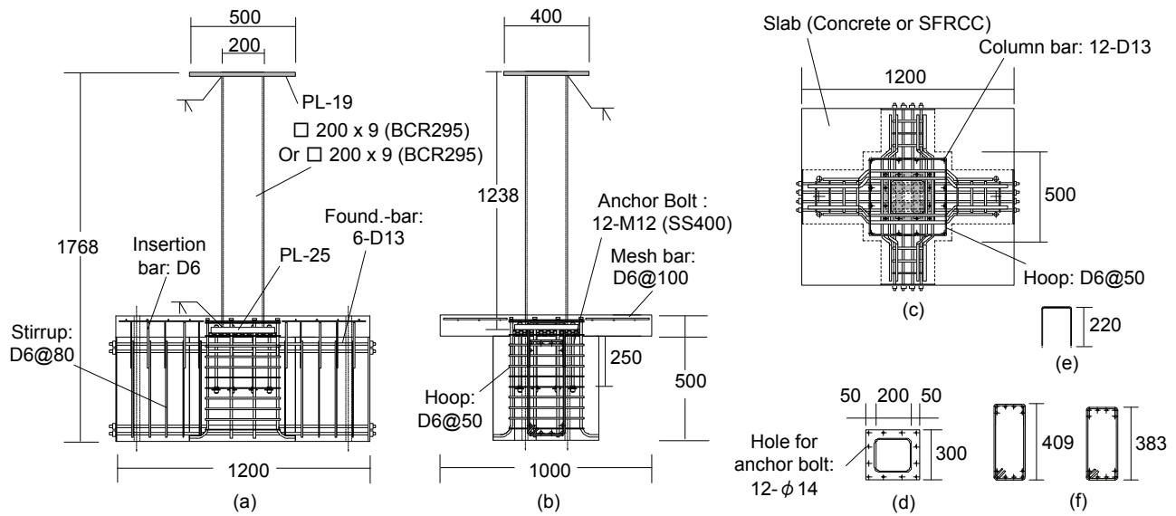
Fig. 4. 12 Test specimen: (a) front elevation; (b) side elevation; (c) plane view; (d) baseplate; (e) insertion bar; and (f) stirrup (unit: mm)
