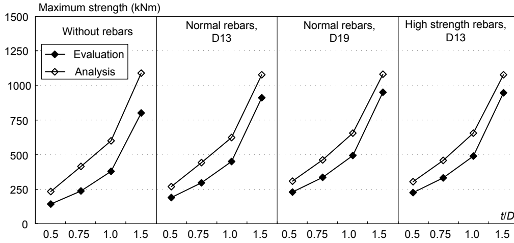
Fig.4.30 Comparisons of predicted maximum strength with respect to slab thickness
