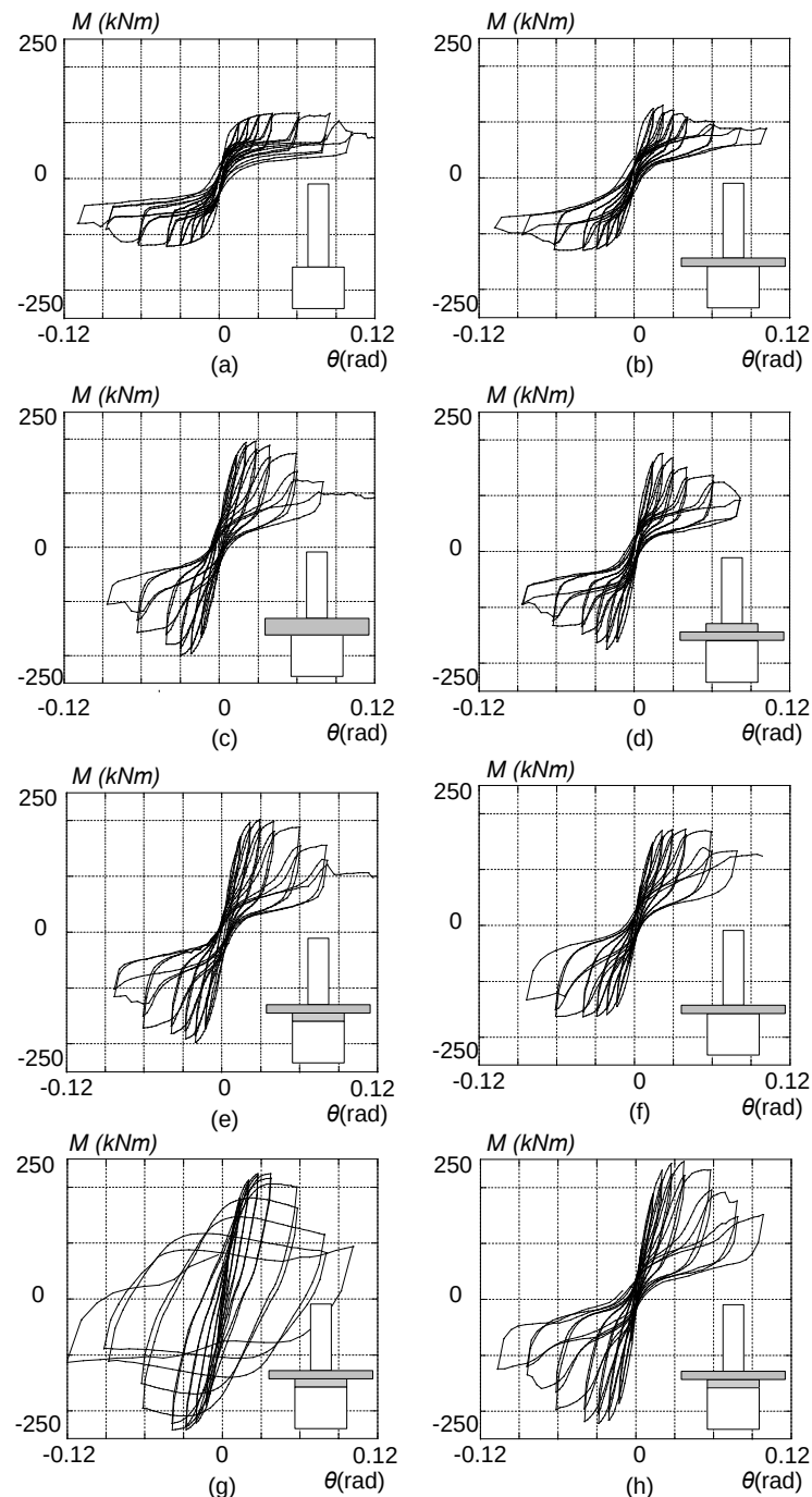
Fig. 2. 5 Moment versus rotation relationships: (a) Standard; (b) ) SL-100; (c) SL-200; (d) Foot-100; (e) Found.-100; (f) SL-100-st; (g) Found.-100-st-t9; and (h) Found.-100-st-t12
