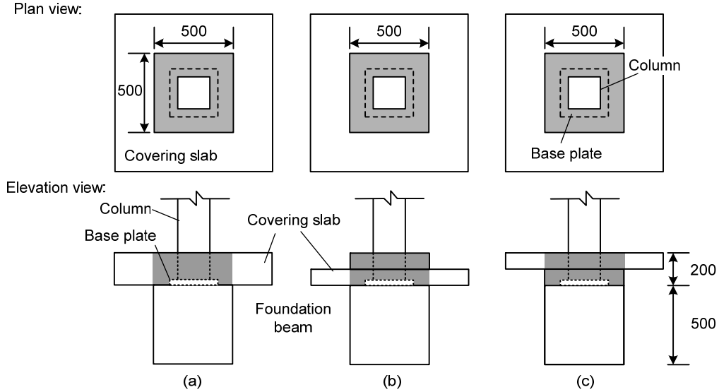
Fig. 2. 14 Effective region in slab for the elastic stiffness evaluation: (a) SL-200; (b) Foot- 100; and (c) Found.-100 (Unit: mm)
