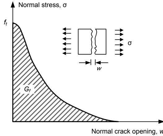
Fig. 4. 3 Tensile stress vs. crack opening displacement diagram (Rots et al., 1985)
