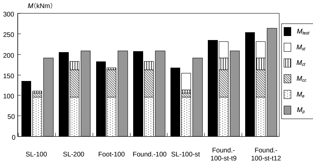
Fig. 2. 11 Maximum strength of specimen
