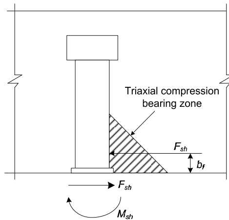
Fig. 5. 15 Dowel action (Johnson and Oehlers 1981)
