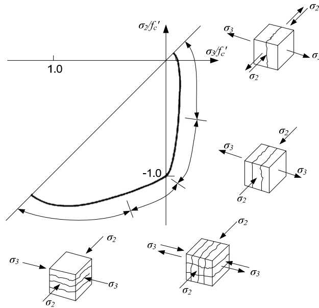
Fig. 3. 4 Failure modes of biaxially loaded concrete (Nelissen, 1972)
