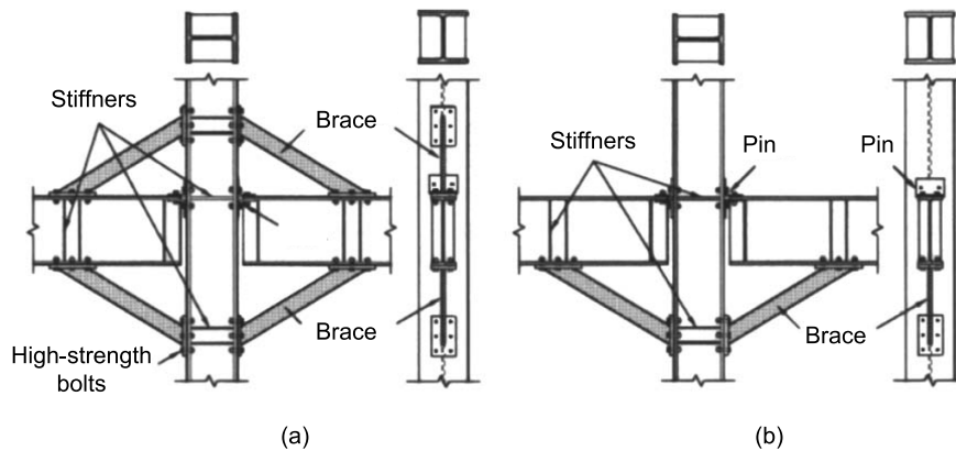
Fig. 6.1 Weld-free beam-column connections: (a) double-side bracing; (b) single-side bracing (Suita et al. 2004 and Inoue et al. 2006)
