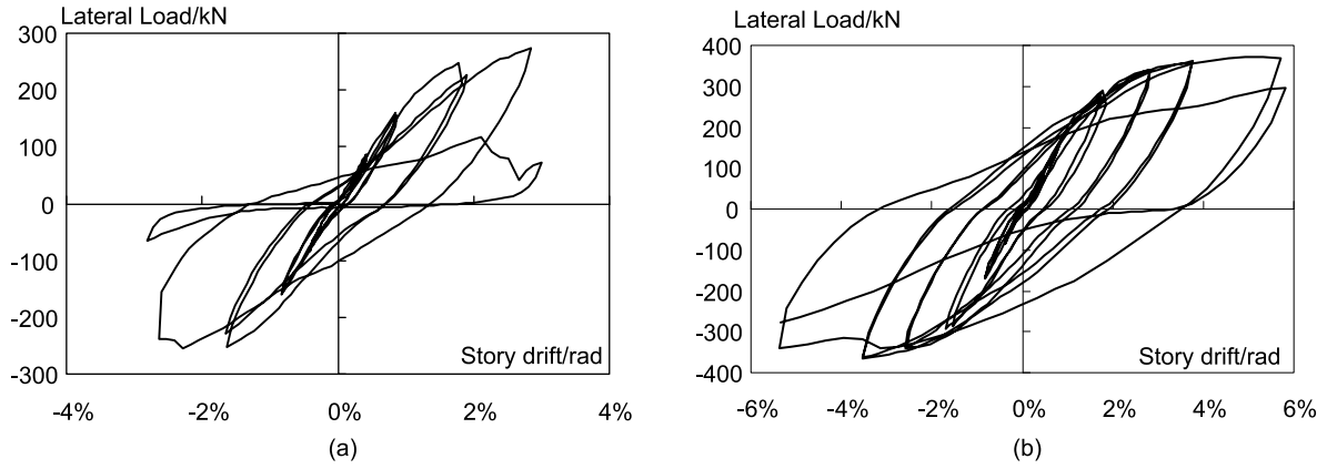
Fig. 6.11 Load versus story drift rotation curves: (a) 'C-4PG50'; (b) 'C-9PG50'
