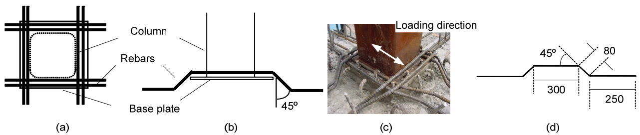
Fig. 4. 13 Configuration of reinforcing bars:
