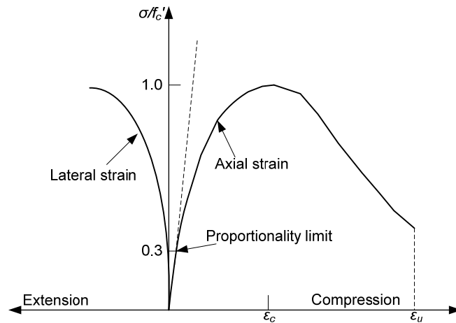
Fig. 3. 1 Typical stress-strain curves for concrete in uniaxial compression test (Chen, 1982)
