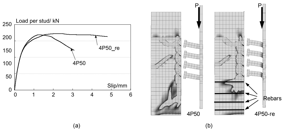
Fig. 5. 27 Effects of the transverse rebars: (a) Load –slip curves; (b) tensile strain contour of the slabs
