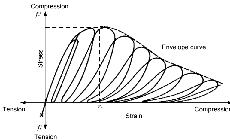
Fig. 3. 2 Cyclic uniaxial compressive stress-strain curve (Karsan and Jirsa, 1969)
