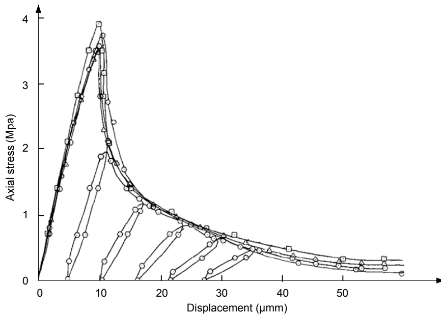
Fig. 3.3 Cyclic uniaxial tensile stress-strain curve (Gopalaratnam and Shah, 1985)
