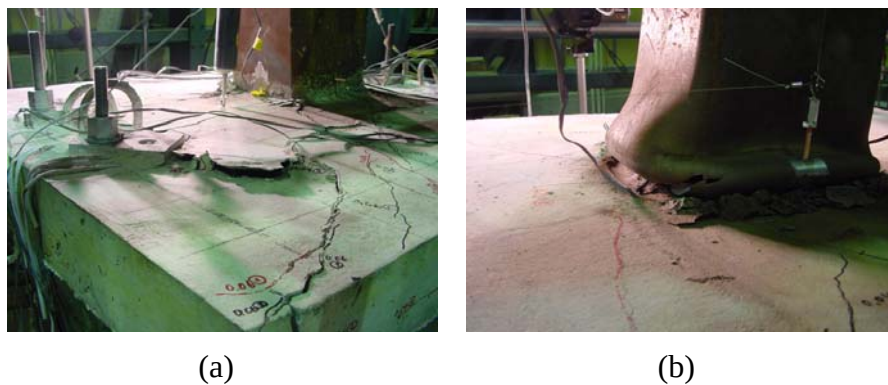
Fig. 2. 6 Failure of reinforced specimens: (a) SL-100-st; (b) Found.-100-st-t9
