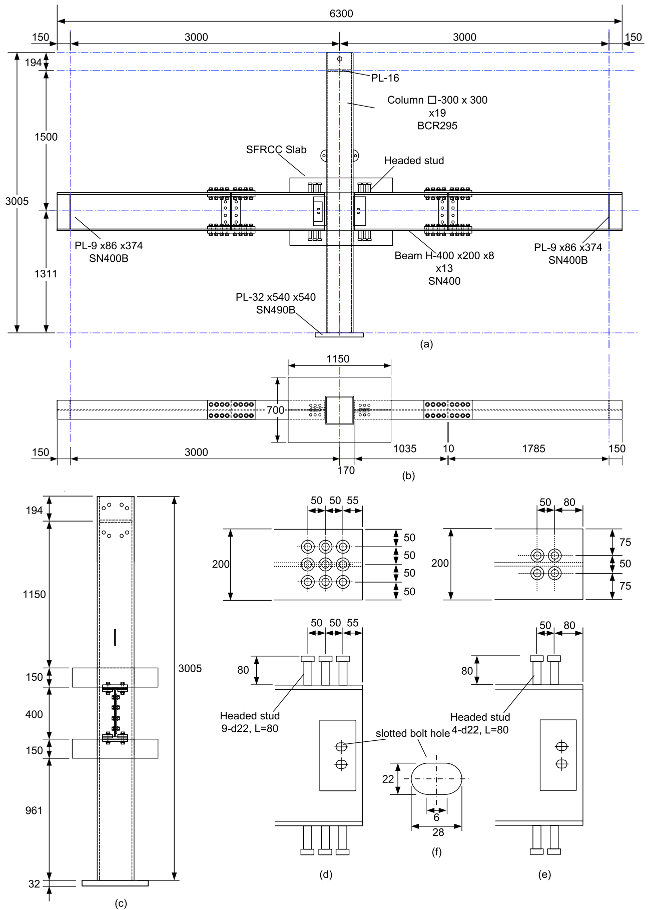
Fig. 6.5 Test specimen: (a) front elevation; (b) plane view; (c) side elevation; (d) studs of Specimen 'C-9PG50'; (e) studs of Specimen 'C-4PG50'; and (f) slotted bolt hole (unit: mm)
