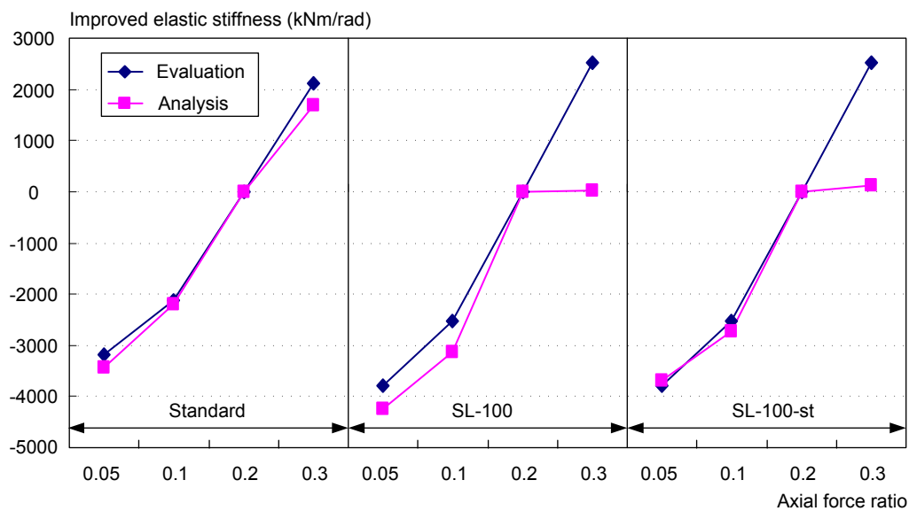
Fig. 3. 31 Comparisons of increased elastic stiffness with respect to axial force ratio
