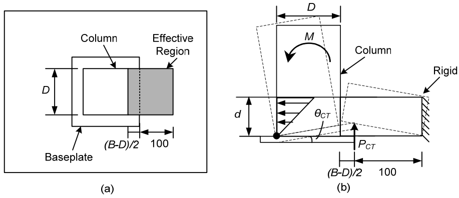
Fig. 2. 16 Model of punching resistance in concrete slab: (a) plan view; (b) elevation view (Unit: mm)
