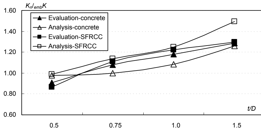
Fig.4.27 Comparisons of predicted elastic stiffness with respect to slab thickness
