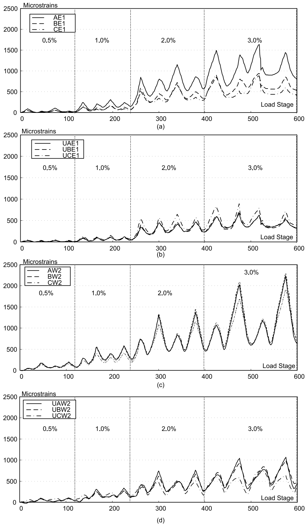
Fig. 6.21 Rebars strains: (a) bottom layer of Specimen 'C-4PG50'; (b) top layer of Specimen 'C-4PG50'; (c) bottom layer of Specimen 'C-9PG50'; and (d) top layer of Specimen 'C-9PG50'
