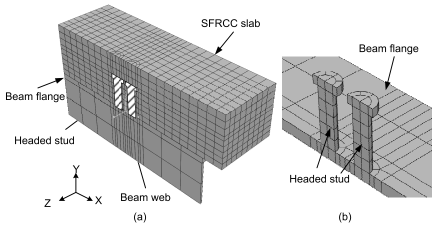
Fig. 5. 19 Model mesh: (a) entire specimen; (b) headed stud connectors
