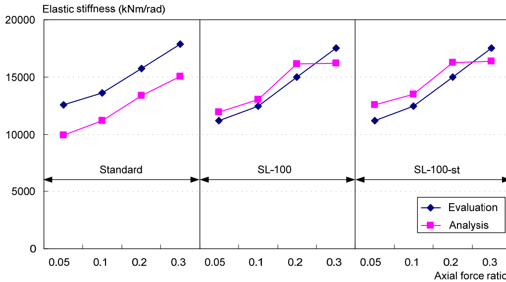
Fig. 3. 30 Comparisons of predicted elastic stiffness with respect to axial force ratio
