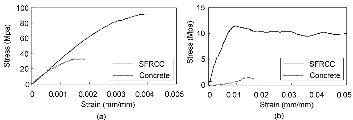
Fig. 4. 11 Stress-strain behavior of concrete and SFRCC: (a) in compression; (b) in tension
