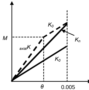
Fig. 2. 18 Definition of the initial stiffness with axial force
