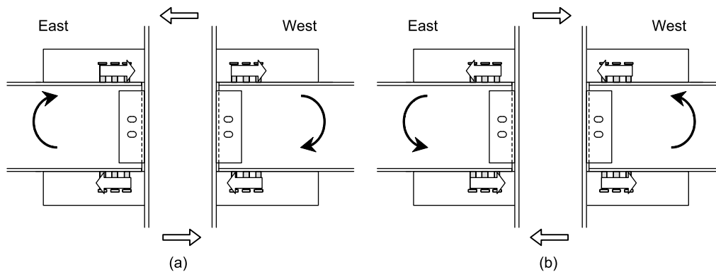
Fig. 6.13 Definition of loading direction: (a) positive loading; (b) negative loading
