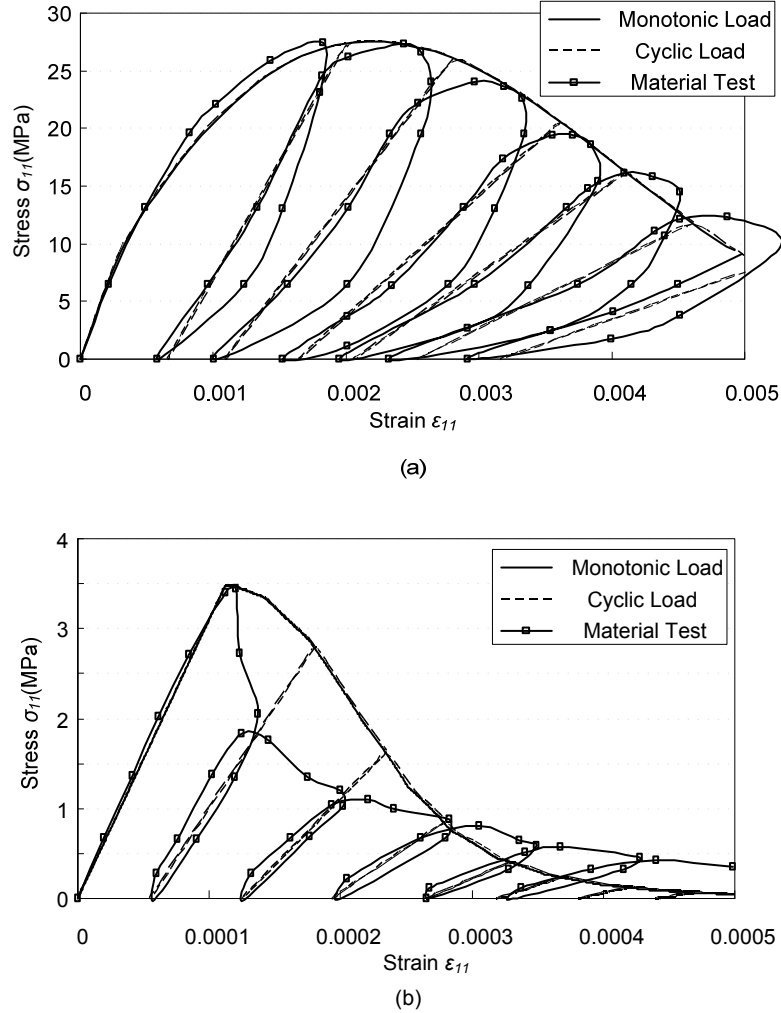
Fig. 3. 14 Numerical solutions of cyclic uniaxial loading compared with experimental results: (a) compressive case (Karsan and Jirsa 1969); (b) tensile case (Gopalaratnam and Shah 1985)
