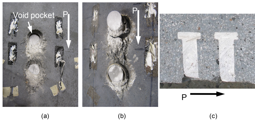
Fig. 5. 11 Detail of specimen failed in the stud: (a) slab side; (b) beam side; and (c) sawed section
