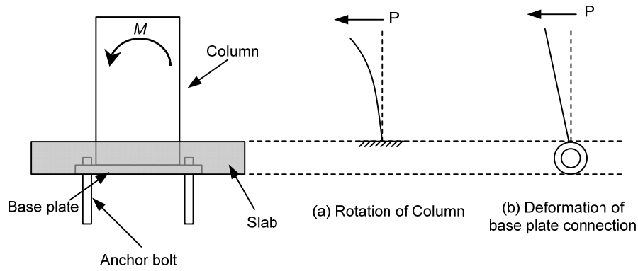
Fig. 2. 12 Mechanism model for stiffness evaluation
