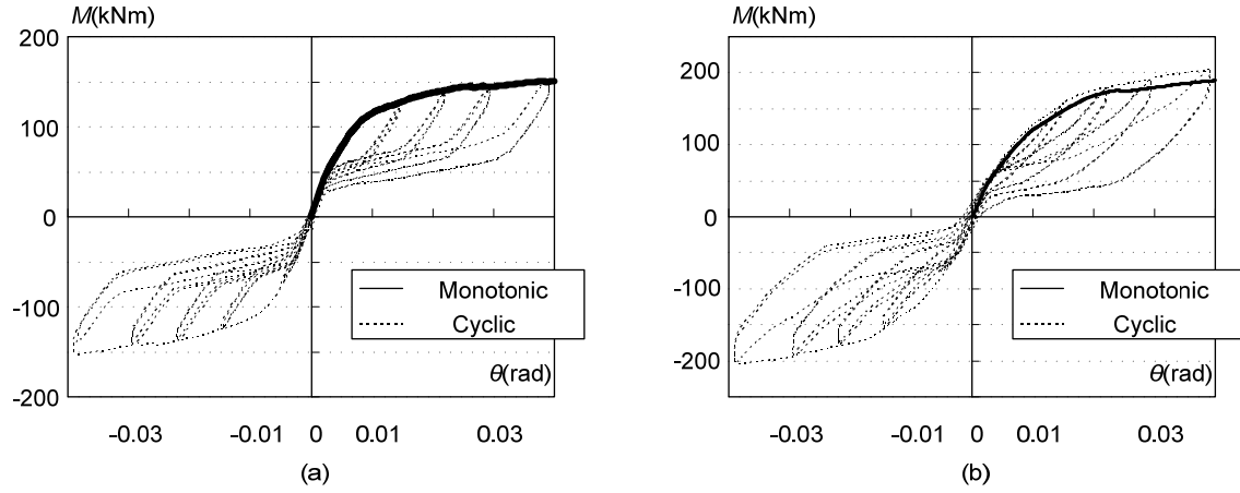
Fig. 3. 21 Comparison between monotonic and cyclic loading analysis: (a) SL-100; (b) SL-100-st
