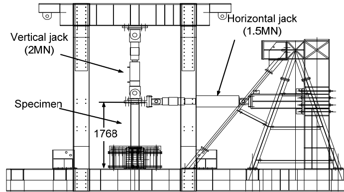
Fig. 2. 4 Elevation of the loading system (unit: mm)
