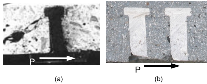
Fig. 5. 16 Sawed section: (a) normal concrete slab; (b) SFRCC slab
