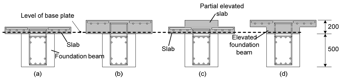
Fig. 2. 2 Shape of concrete slab: (a) Flat slab type ‘SL-100’; (b) Flat slab type ‘SL-200’; (c) Partial elevated slab type ‘Foot-100’; and (d) Elevated foundation type ‘Found.-100’ (Unit: mm)
