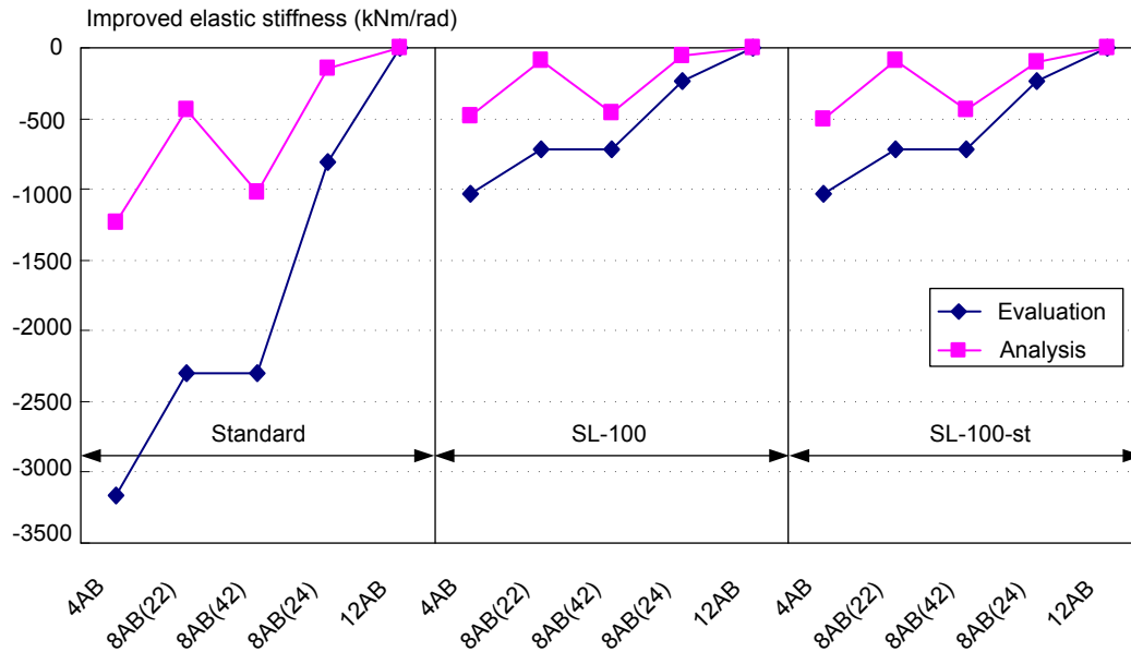
Fig. 3. 29 Comparisons of increased elastic stiffness with respect to number of anchor bolts
