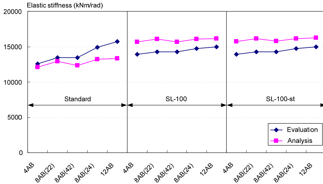
Fig. 3. 28 Comparisons of predicted elastic stiffness with respect to number of anchor bolts
