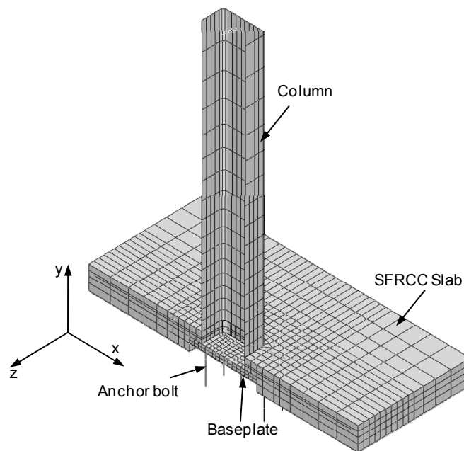
Fig. 4. 19 Analysis model
