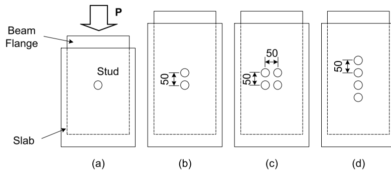
Fig. 5. 6 Layout of studs:
