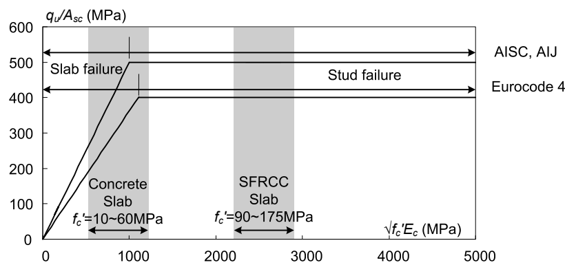
Fig. 5. 4 Nominal shear strength of one stud embedded in solid slab
