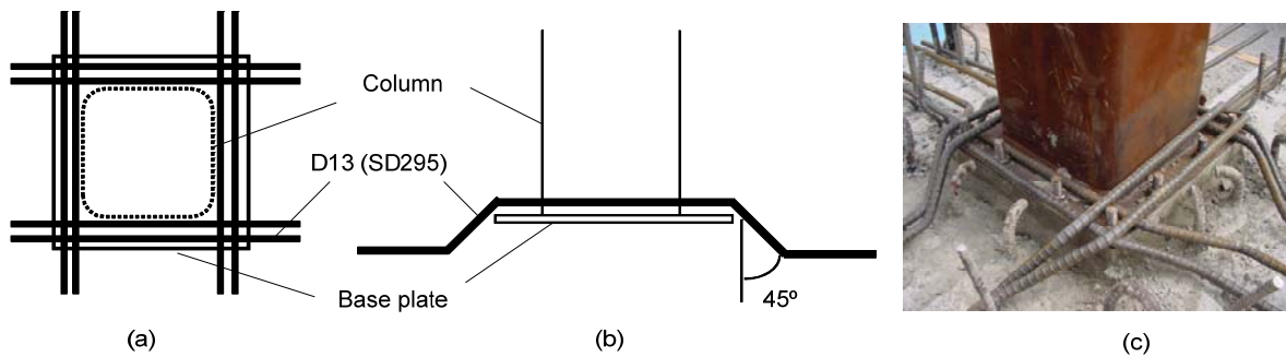
Fig. 2. 3 Arrangement of reinforcing bars: (a) plan view; (b) elevation; and (c) arrangement of reinforcing bars
