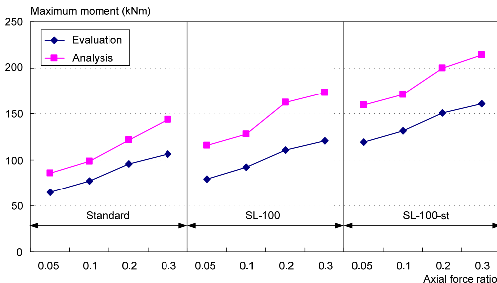
Fig. 3. 38 Comparisons of predicted maximum moment with respect to axial force ratio
