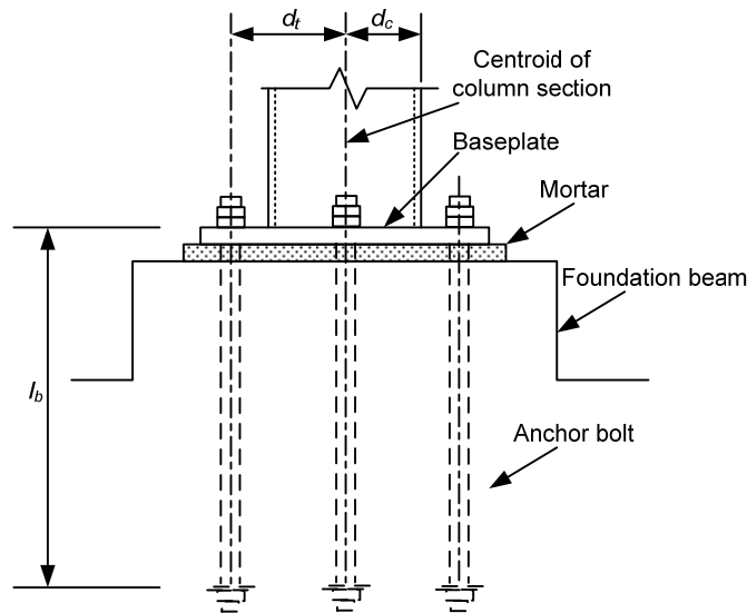
Fig. 2. 13 Dimension of exposed column base (AIJ 2006)
