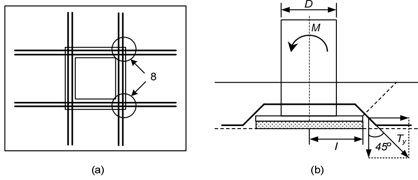
Fig. 2. 10 Model of contribution of rebars: (a) plan view; (b) elevation view
