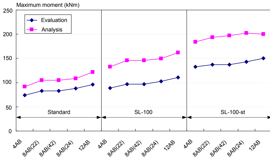
Fig. 3. 36 Comparisons of predicted maximum moment with respect to number of anchor bolts
