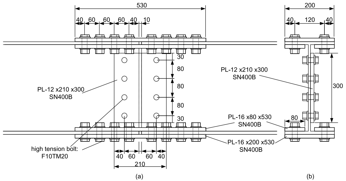
Fig. 6. 7 Details for bolted splice: (a) front view; (b) side view (unit: mm)
