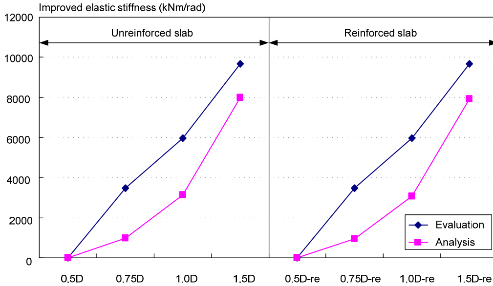
Fig. 3. 33 Comparisons of increased elastic stiffness with respect to slab thickness
