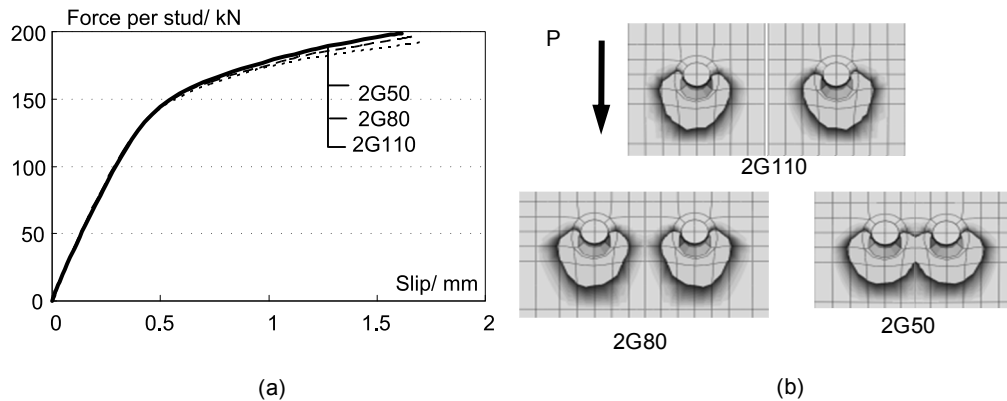
Fig. 5. 26 Effects of the transverse spacing: (a) Load –slip curves; (b) compressive strain contour of the slabs
