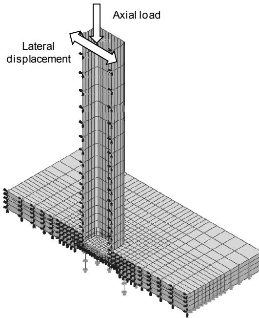
Fig. 3. 16 Application of load and boundary conditions
