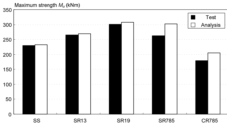
Fig. 4. 23 Comparison of maximum strength
