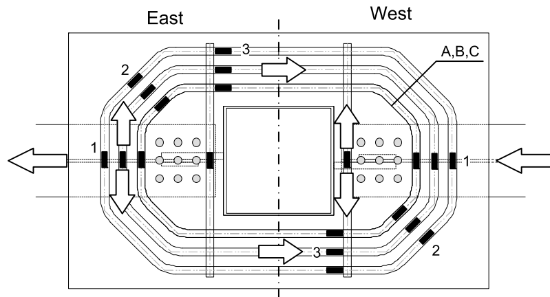
Fig. 6.25 Resisting force flow of rebars in positive loading
