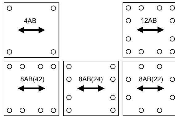
Fig. 3. 23 Layout of anchor bolts
