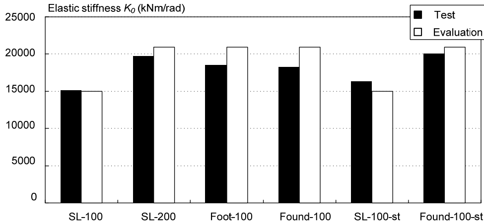
Fig.2.19 Initial stiffnesses of specimens
