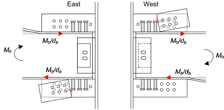
Fig. 6. 18 Exaggerated deformation of specimens
