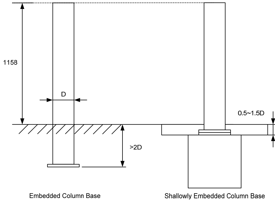
Fig. 3. 34 The corresponding embedded column base
