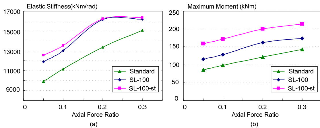
Fig. 3. 25 Influence of axial force ratio: (a) elastic stiffness; (b) maximum moment
