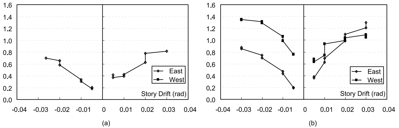
Fig. 6.24 Ratio of resisting force of rebars between location 1 and location 3:
