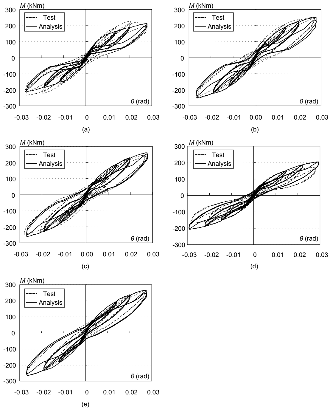
Fig. 4. 21 Comparison of moment-rotation curves: (a) SS; (B) SR13; (c) SR785; (d) CR785 and (e) SR19
