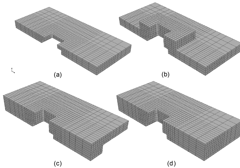
Fig. 3. 10 Modeling of slabs: (a) SL-100/SL-100-st; (b) Foot-100; (c) Found.-100/ Found.-100-st; and (d) SL-200
