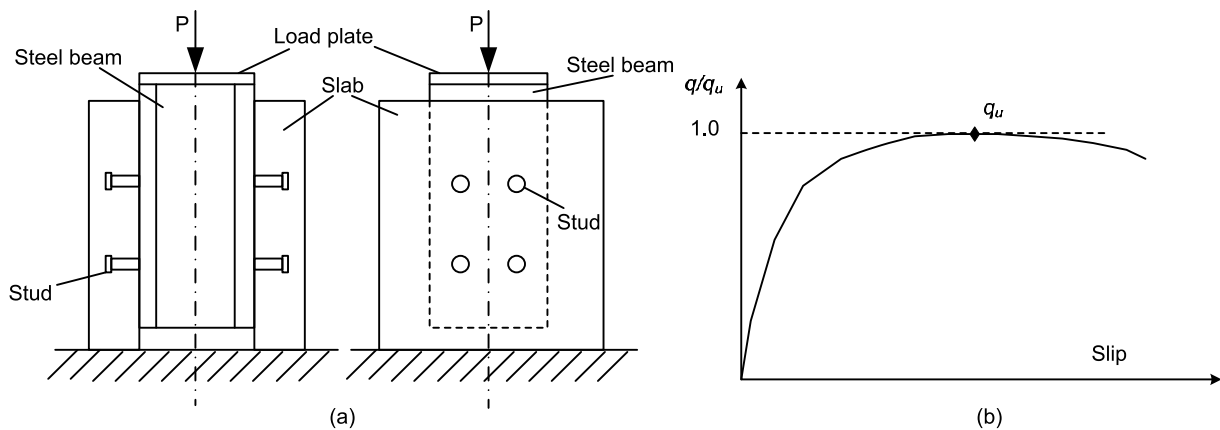
Fig. 5. 3 Test on shear connectors:
