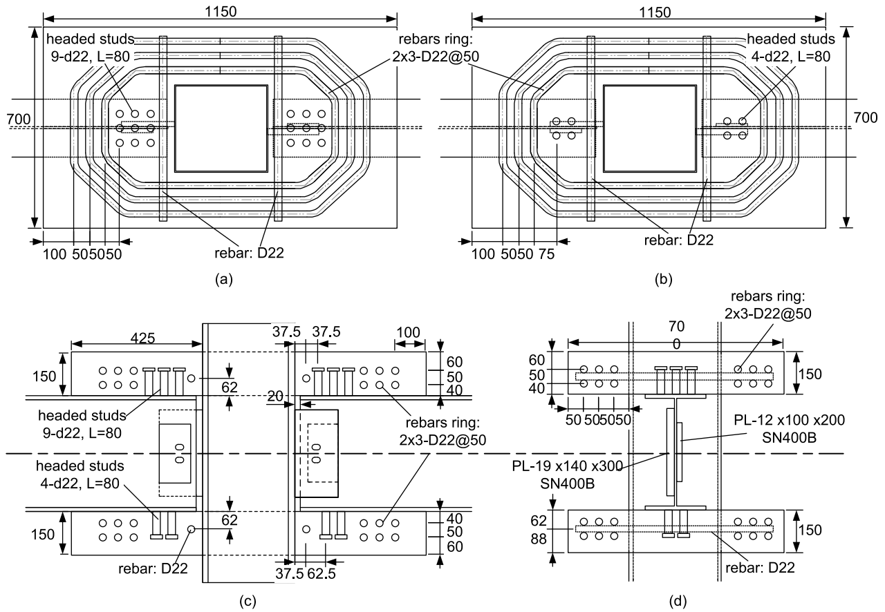
Fig. 6. 6 Details for slab and rebars: (a) plane view of Specimen 'C-9PG50'; (b) plane view of Specimen 'C-4PG50'; (c) front view; and (d) side view (unit: mm)
