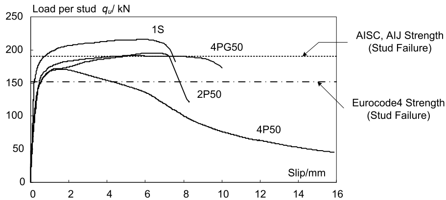
Fig. 5. 8 Load-slip curves
