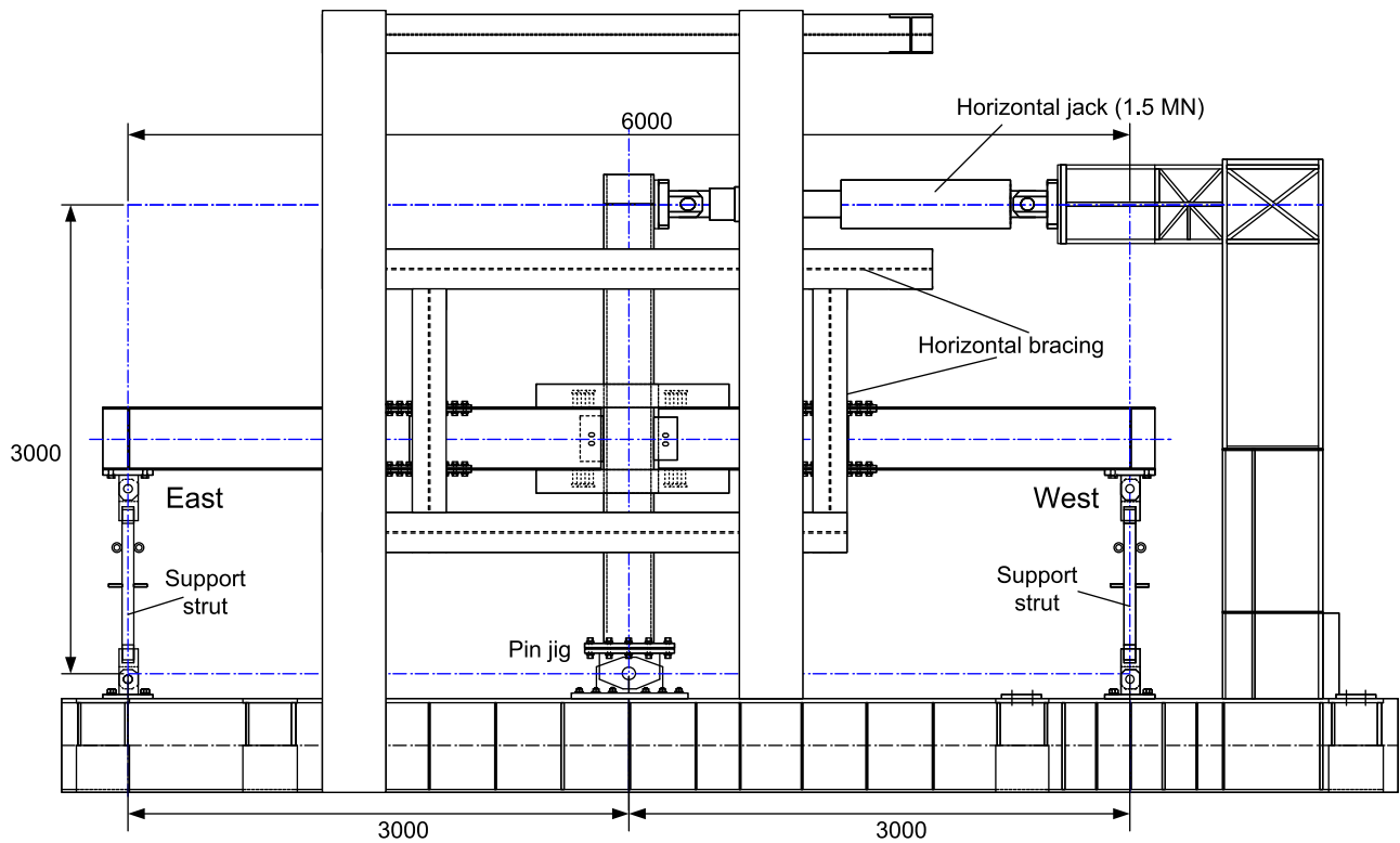
Fig. 6. 8 Test setup (unit: mm)
