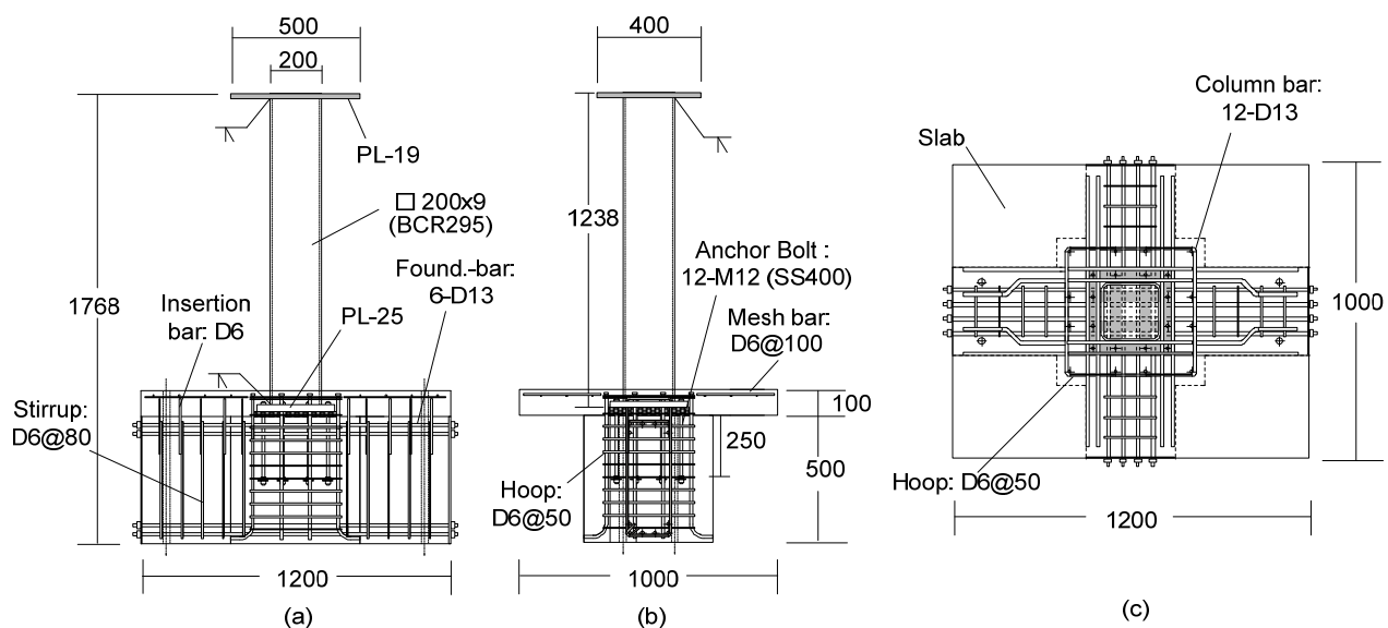
Fig. 2.1 Test specimen (SL-100-st):
