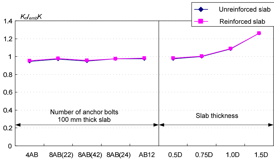
Fig. 3. 35 The ratio of the elastic stiffness based on the corresponding embedded column base
