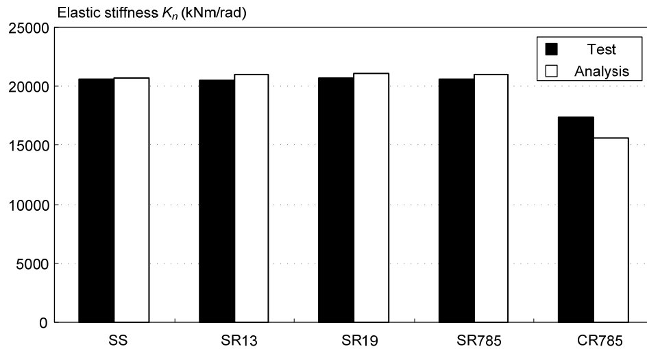
Fig. 4. 22 Comparison of elastic stiffness
