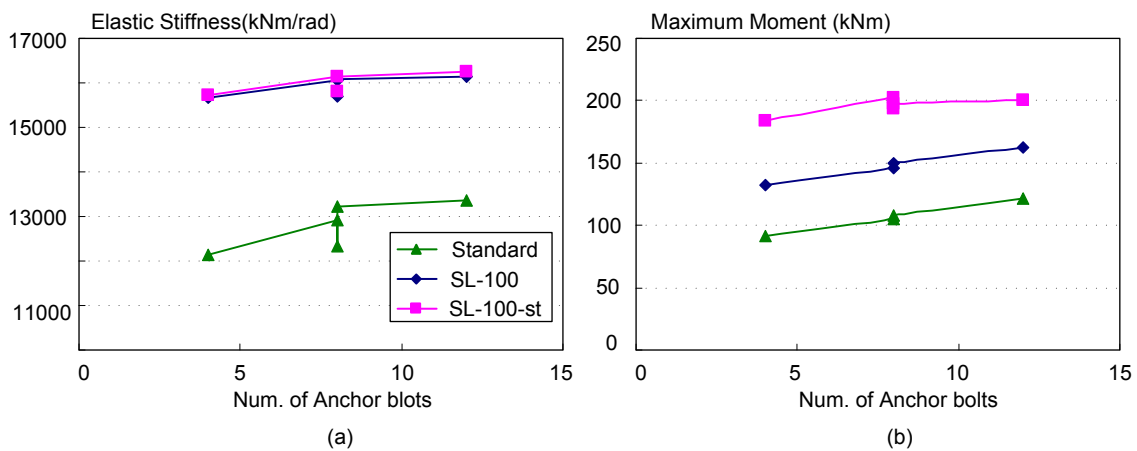
Fig. 3. 24 Influence of anchor bolts: (a) elastic stiffness; (b) maximum moment
