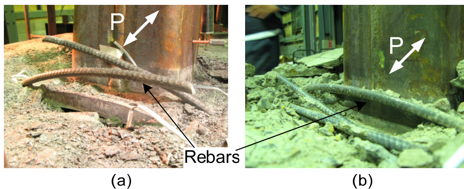
Fig. 4. 17 Deformation of reinforcement: (a) rupture; (b) buckling
