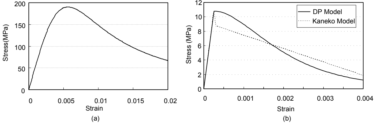
Fig. 4. 20 Material Property: (a) compression; (b) tension
