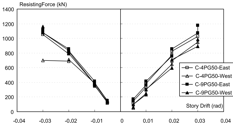
Fig. 6.22 Resisting force of rebars
