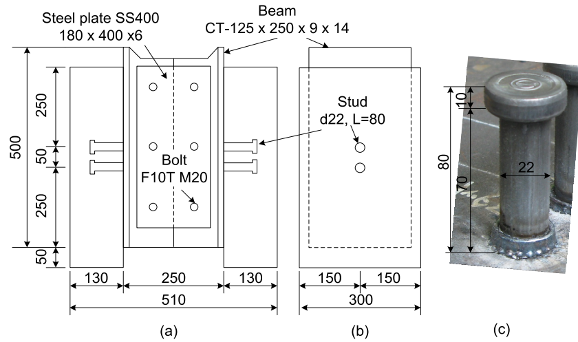
Fig. 5. 5 Details of specimen:
