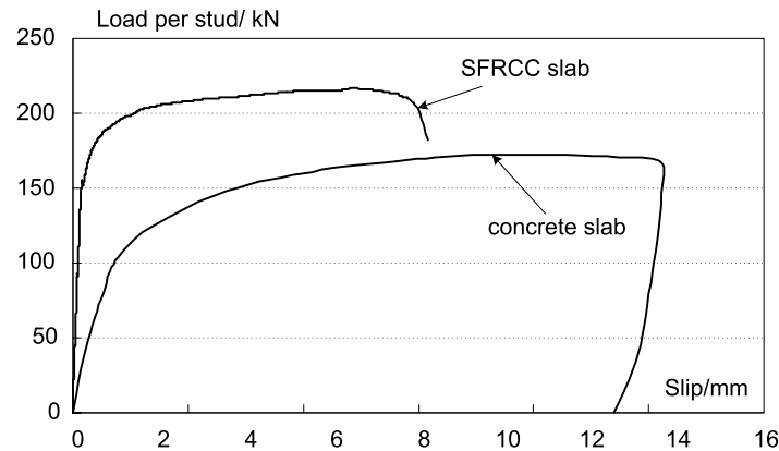
Fig. 5. 17 Comparison of load-slip curves: concrete vs. SFRCC
