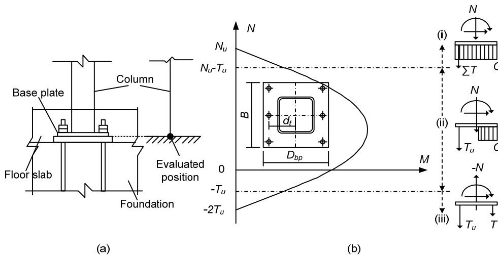
Fig. 2. 7 Model of evaluation of the maximum moment resisted by exposed column base:
