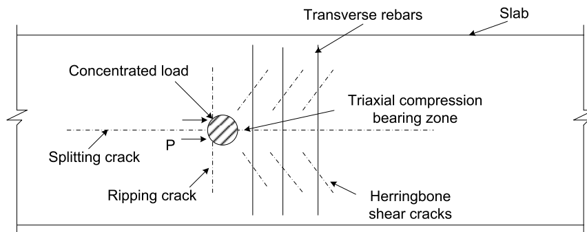
Fig. 5. 18 Tensile cracks induced by concentrated load
