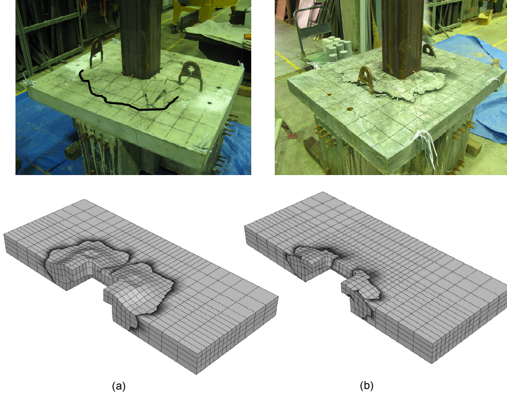
Fig. 4. 24 Failure region obtained from experiment and analysis: (a) CR785; (b) SR785
