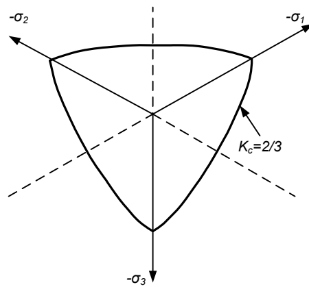
Fig. 3. 12 Yield surfaces in the deviatoric plane
