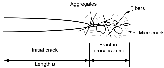
Fig. 4. 4 Fracture process along a crack plane
