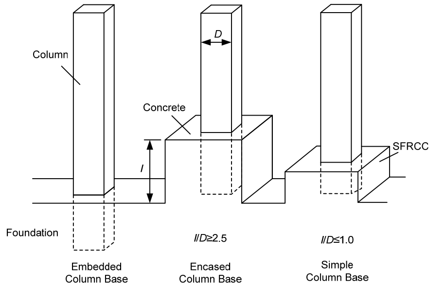
Fig. 4. 1 Simple column base connection (Kaneko et al. 2006)
