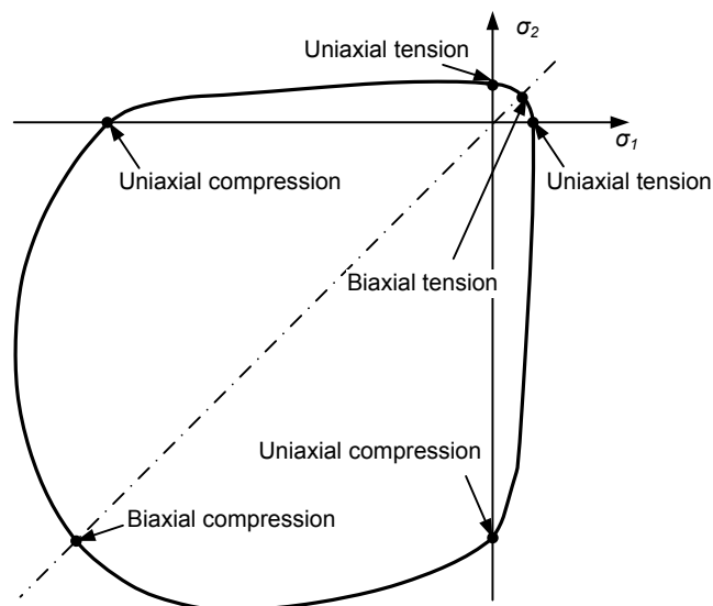
Fig. 3. 13 Yield surface in plane stress
