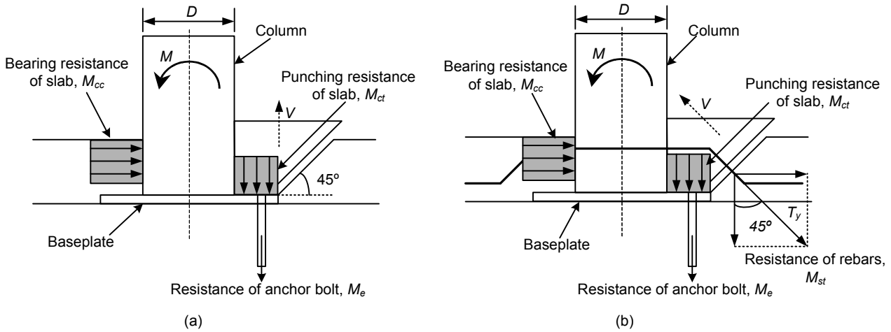
Fig. 4. 28 Mechanism model for maximum resisting moment evaluation:
