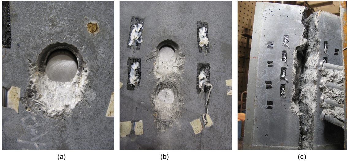
Fig. 5. 12 Failure region in the SFRCC slab: (a) 1S; (b) 2P50; and (c) 4P50
