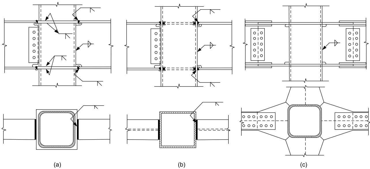
Fig. 6.3 Typical beam-column connections: (a) through plate diaphragm; (b) internal diaphragm; and (c) external diaphragm. (AIJ 2006)
