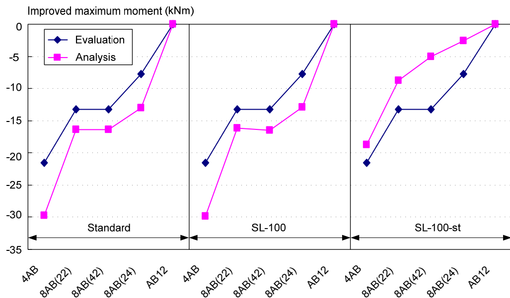
Fig. 3. 37 Comparisons of increased maximum moment with respect to number of anchor bolts
