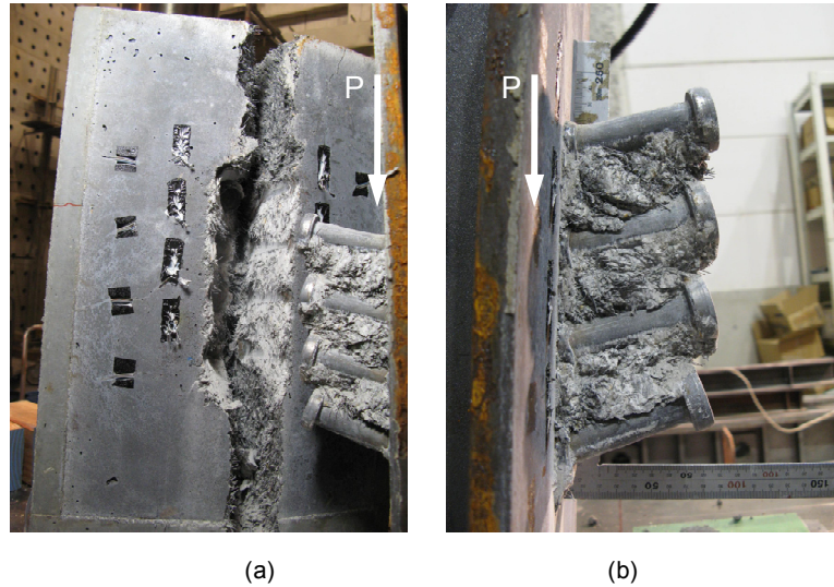
Fig. 5. 10 Detail of specimen failed in the slab: (a) slab side; (b) beam side
