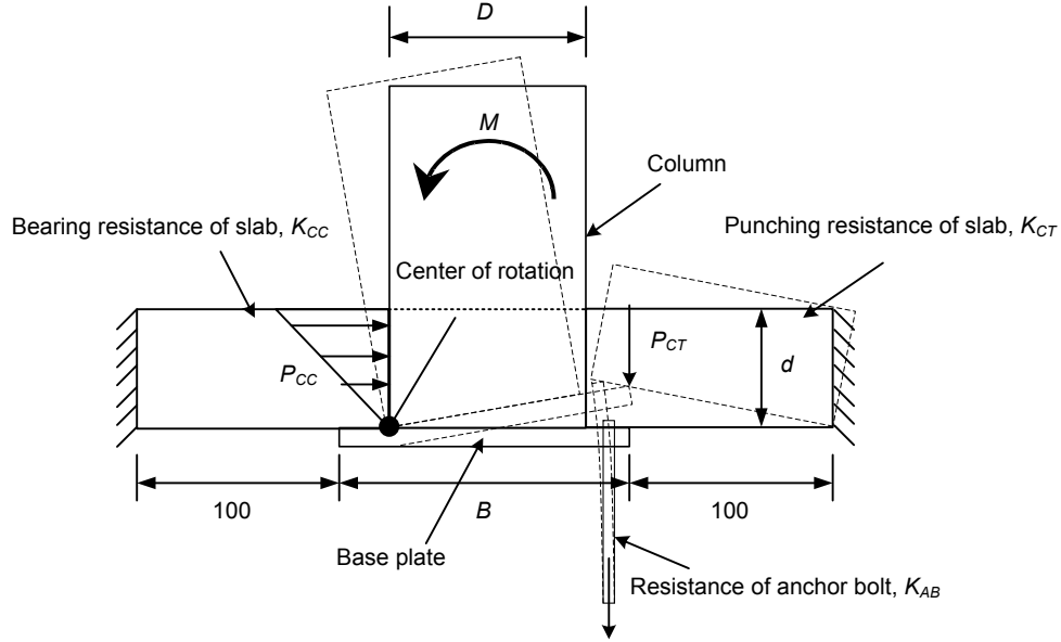
Fig. 4. 25 Mechanism model for elastic stiffness evaluation
