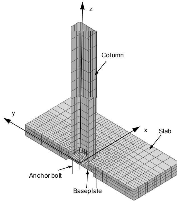
Fig. 3. 7 Analysis model
