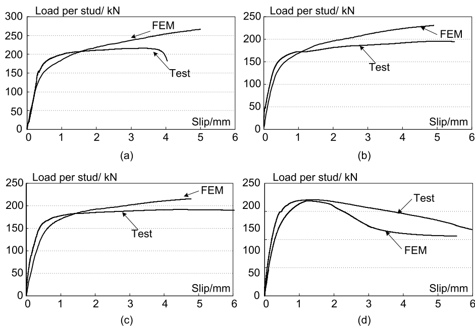
Fig. 5. 22 Load-slip curves of specimens: (a) 1S; (b) 2P50; (c) 4PG50; and (d) 4P50
