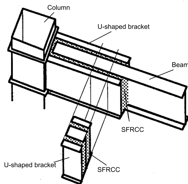
Fig. 6.2 U-shaped bracket beam-column connection (Kaneko et al. 2002)
