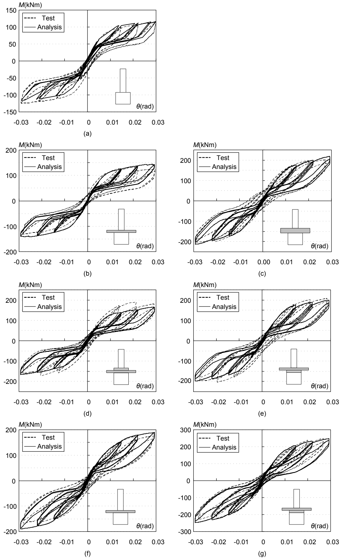
Fig. 3. 17 Comparison of moment-rotation curves: (a) Standard; (b) SL-100; (c) SL-200; (d) Foot-100; (e) Found.-100; (f) SL-100-st; and (g) Found.-100-st-t12
