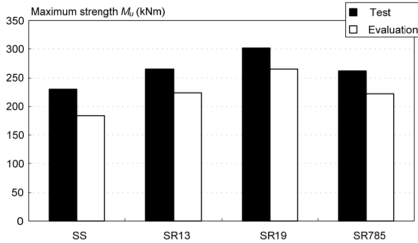
Fig.4.31 Maximum strength of specimen
