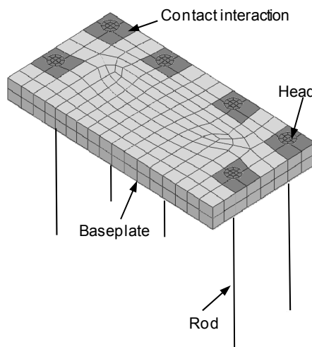
Fig. 3. 9 Modeling of anchor bolts
