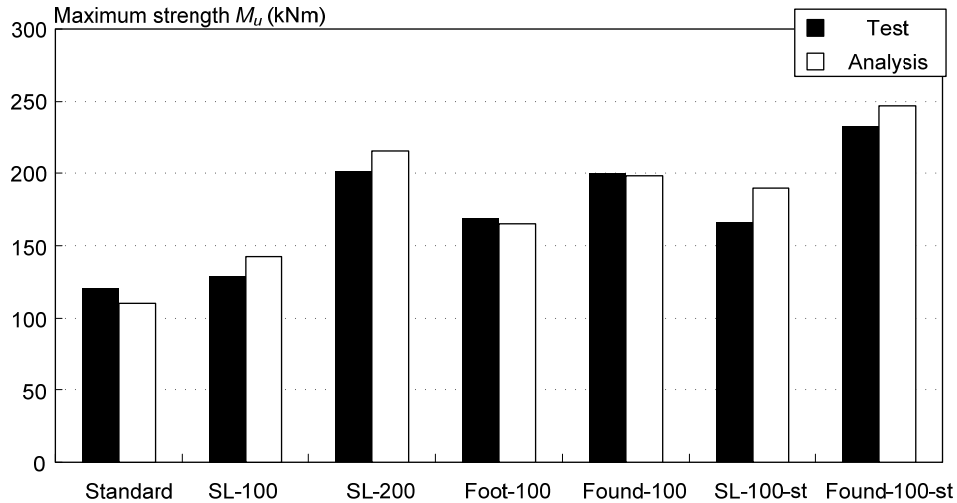
Fig. 3. 19 Comparison of maximum strength between test and analysis
