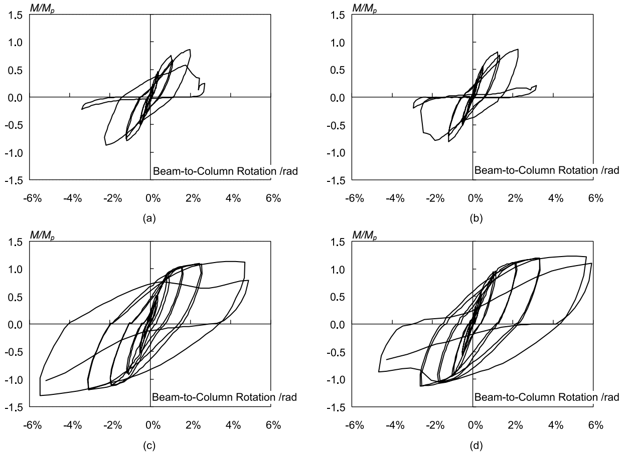
Fig. 6.12 Beam moment versus beam-to-column rotation curves:
