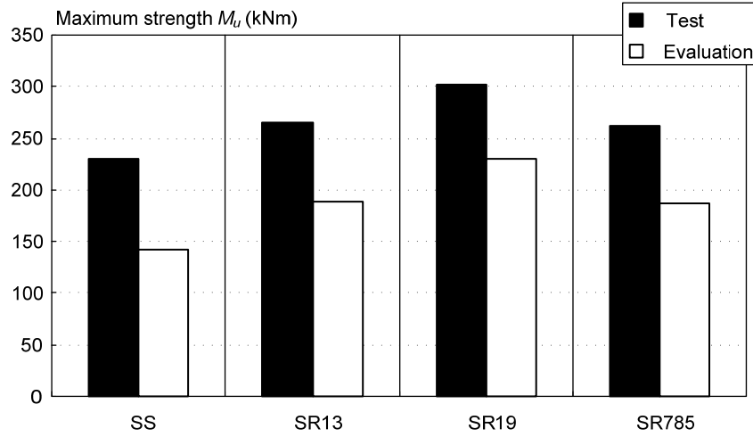
Fig.4.29 Maximum strength of specimen
