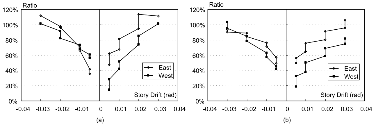
Fig. 6.23 Ratio of resisting force of rebars to beam flange load:
