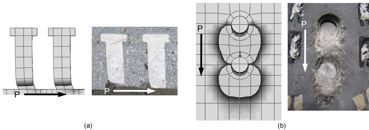
Fig. 5. 23 Comparison of numerical and experimental behavior of specimen failed in the stud: (a) deformation of studs; (b) crushed region in the slab
