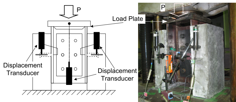
Fig. 5. 7 Setup of push-out tests
