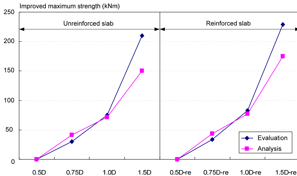
Fig. 3. 41 Comparisons of increased maximum moment with respect to slab thickness
