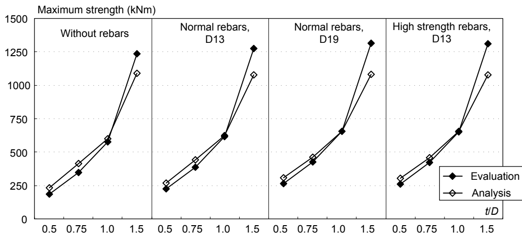
Fig.4.32 Comparisons of revised predicted maximum strength with respect to slab thickness
