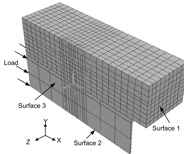
Fig. 5. 21 Application of load and boundary conditions
