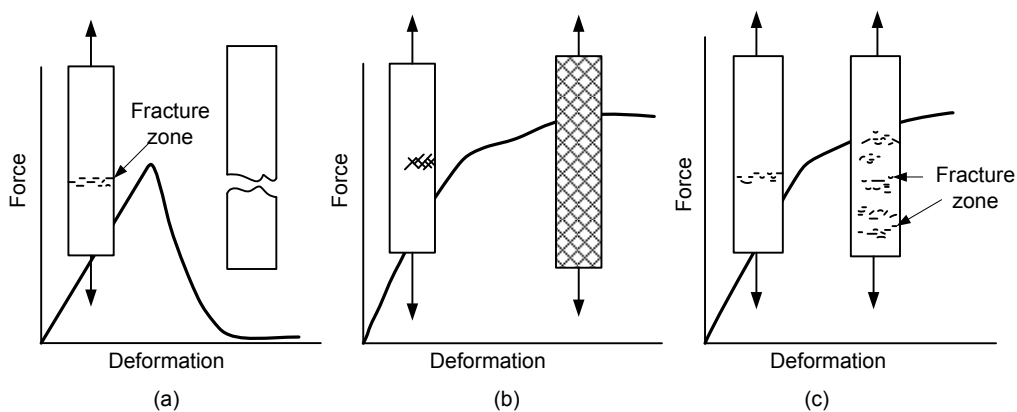
Fig. 4. 7 Tensile behavior of different material: (a) concrete; (b) steel; and (c) SFRCC (Elfgren, 1989)
