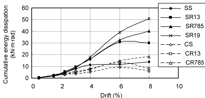
Fig. 4. 18 Cumulative energy dissipation of each loading cycle
