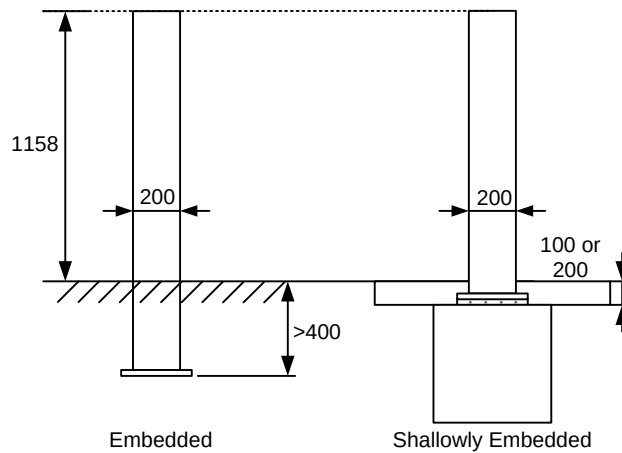
Fig. 2. 20 Comparison between embedded column base and shallowly embedded column base
