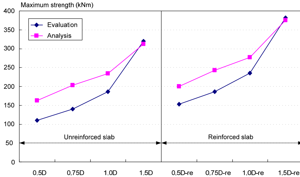
Fig. 3. 40 Comparisons of predicted maximum moment with respect to slab thickness
