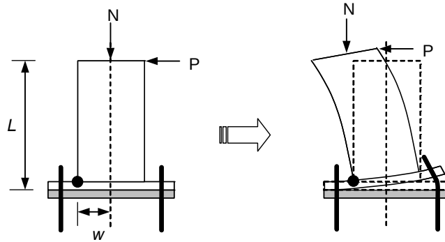
Fig. 2. 17 Deformation of the column before and after detachment
