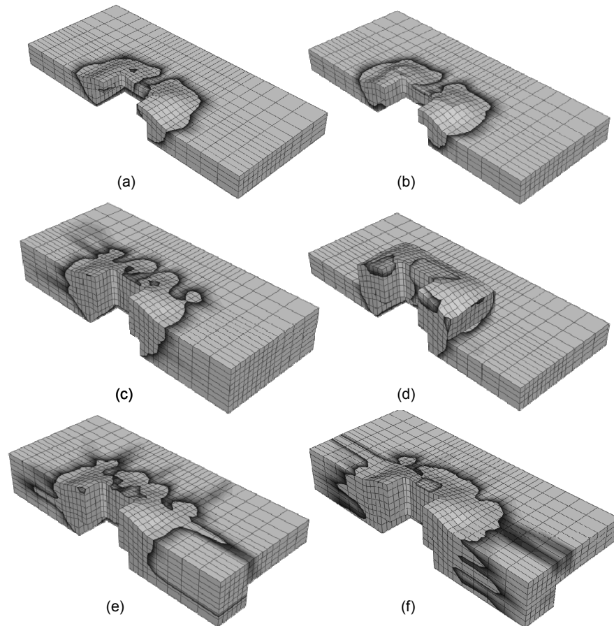
Fig. 3. 20 Failure region obtained from analysis: (a) SL-100; (b) SL-100-st; (c) SL-200; (d) Foot-100; (e) Found.-100; and (f) Found.-100-st-t12
