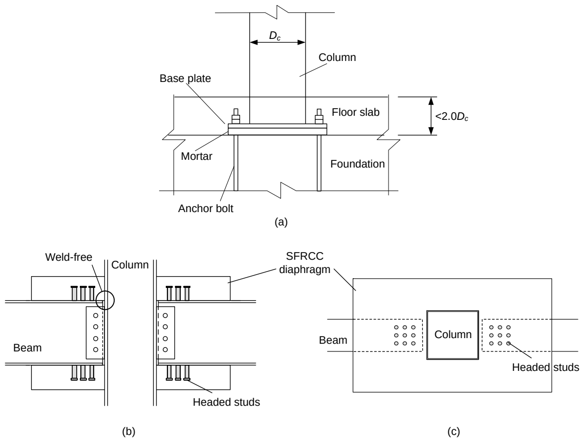
Fig. 1.1 Proposed connections: (a) shallowly embedded column base; (b) elevation view of beam-column connection; and (c) plan view of beam-column connection
