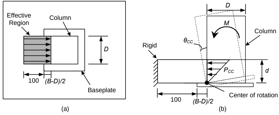
Fig. 2. 15 Model of compressive resistance in concrete slab: (a) plan view; (b) elevation view (Unit: mm)
