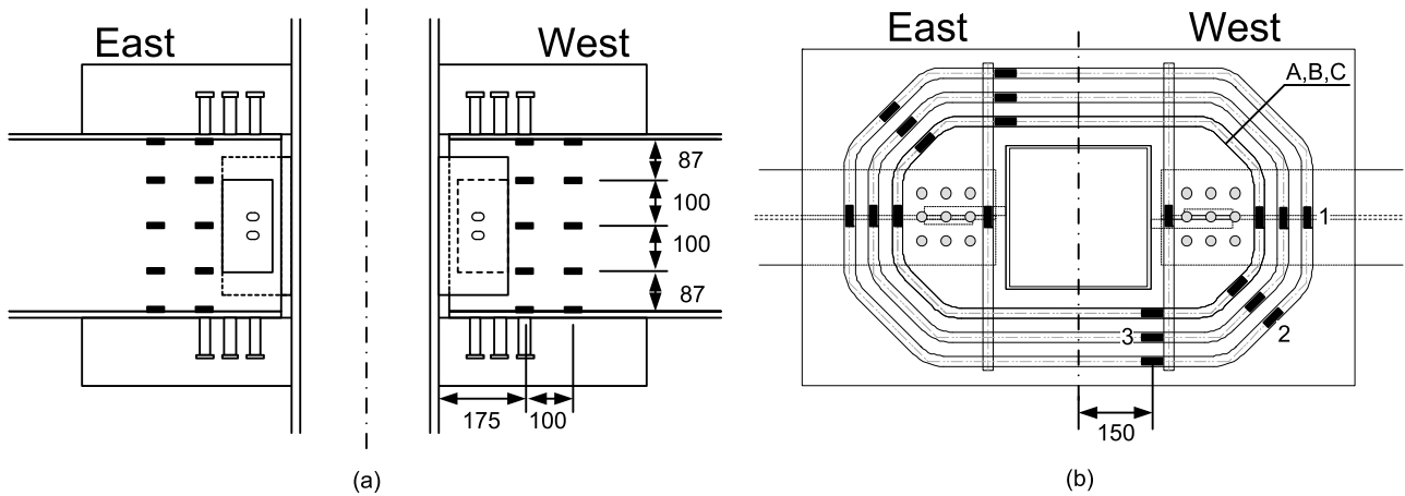
Fig. 6.10 Layout of strain gauges: (a) side view of beam; (b) plane view of rebar (unit: mm)
