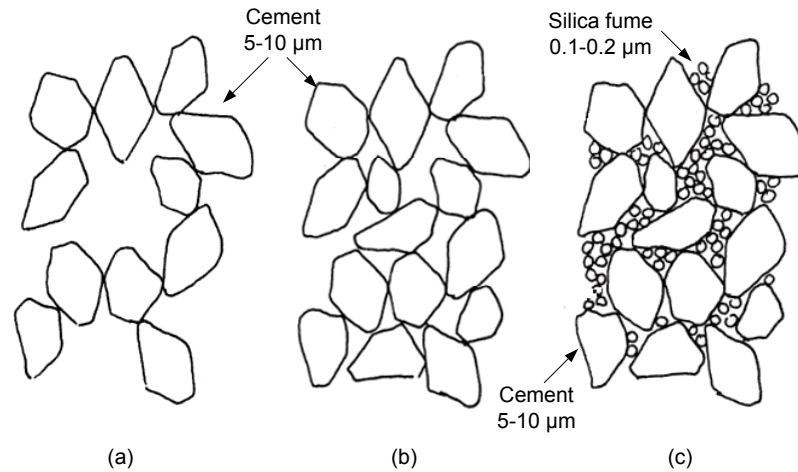
Fig. 4. 5 The structural of the matrix:
