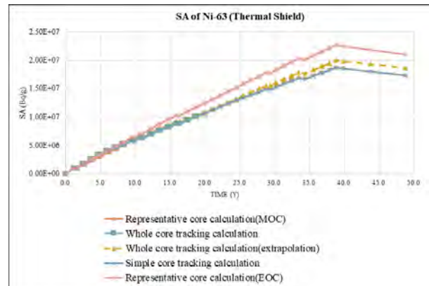
Fig. 6. Specific activity of Ni-63 at thermal shield
