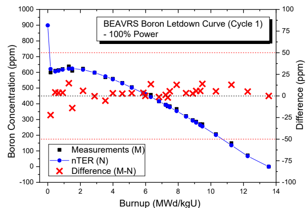
Fig. 3. Boron letdown curve for cycle 1 (100% Power)
