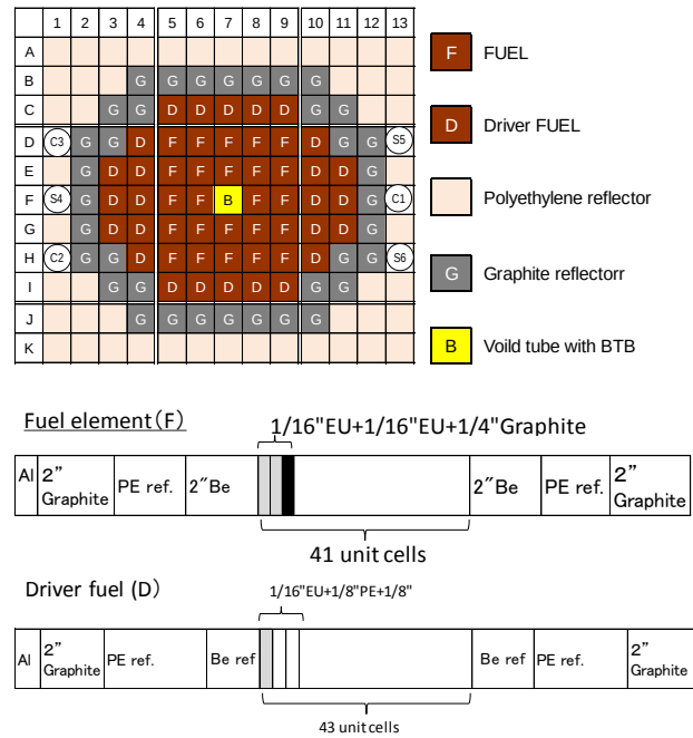
Fig. 3. Configurations of EEG14 core, Fuel element (F) and Driver fuel element (D). (C : Control rod, S : Safety rod)
