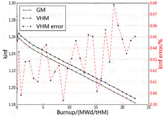
Fig. 2. Comparison of k_{\text{inf}} as function of burnup between the VHM and the GM
