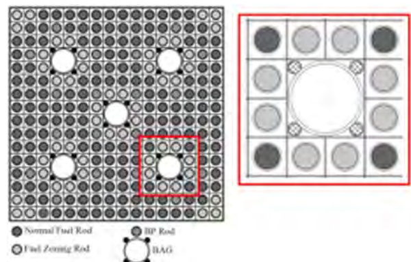
Fig. 4. Standard CE fuel assembly type with BAG design.
