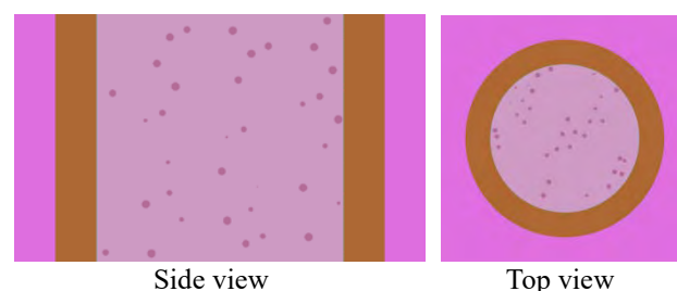
Fig. 1. dispersed positions of 1000 fuel particles with the radius of 100μm
