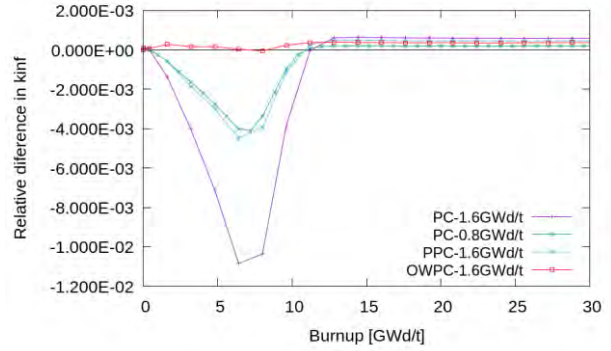
Fig. 3. Errors of k_{inf} in the VERA/2P problem
