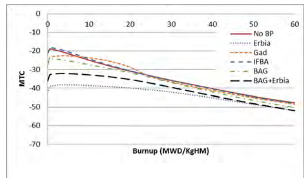
Fig. 11. Comparison of MTC for CE fuel assembly type.
