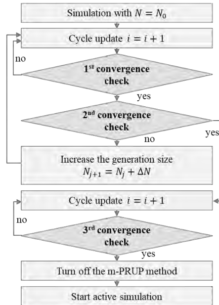
Fig. 1 Flowchart of the m-PRUP method
