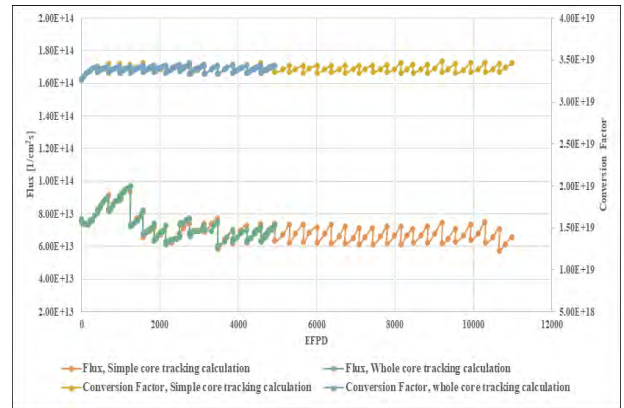
Fig. 4. Neutron flux and conversion factor at baffle
