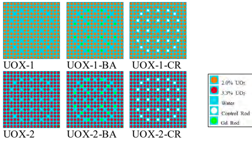
Fig. 1. Geometries of assemblies
