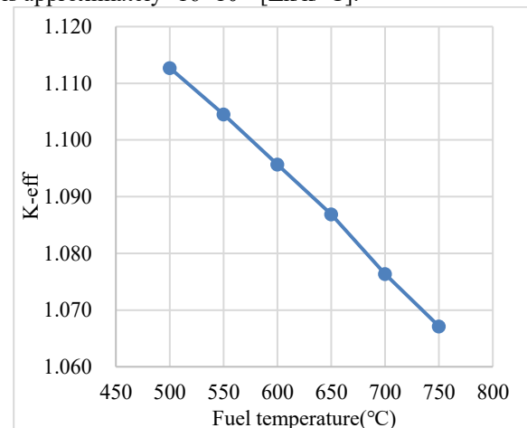
Fig. 3. The K_{\text{eff}} by fuel temperature
