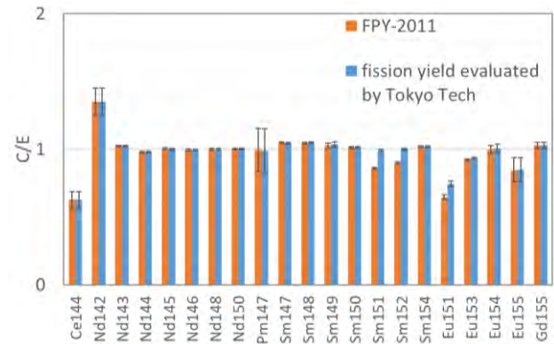
Fig. 3. C/E values of fission products
