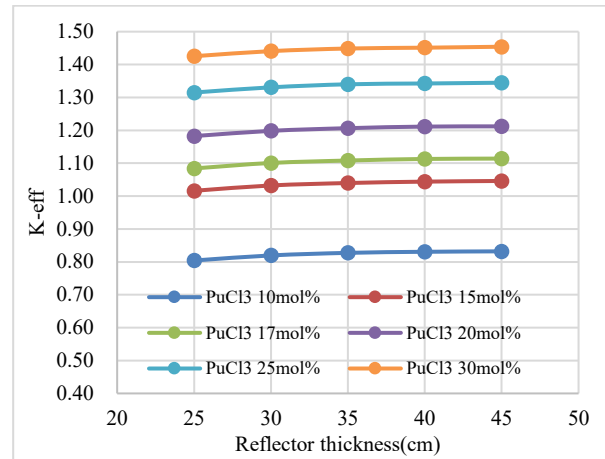
Fig. 2. The K_{\text{eff}} by different molar fraction of fuel and Reflector thickness.
