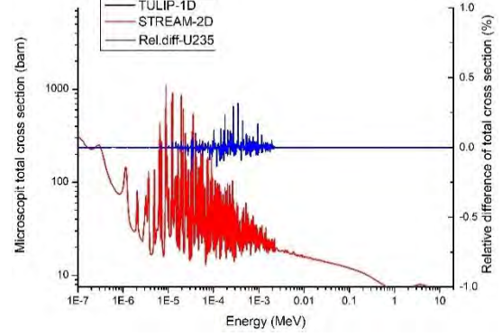
Figure 3 Microscopic total cross section of U-235 and its difference
