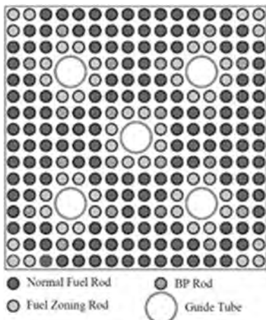
Fig. 2. Standard CE fuel assembly type.
