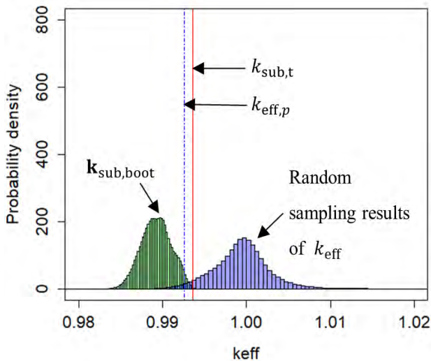
Fig. 6. Probability density distributions of random sampling results of k_{\text{eff}} , k_{\text{sub,boot}} and k_{\text{sub,t}} , k_{\text{eff,p}} . (Case 4)
