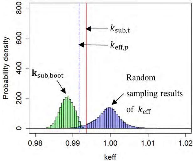
Fig. 5. Probability density distributions of random sampling results of k_{\text{eff}} , k_{\text{sub,boot}} and k_{\text{sub,t}} , k_{\text{eff,p}} . (Case 3)
