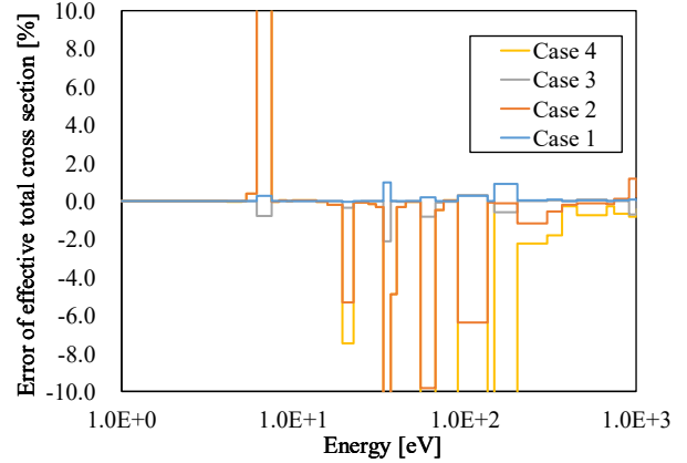
Fig. 3. Error of U238 effective total cross section in 172 XMAS energy group structure (Region 1, inner region of pellet).
