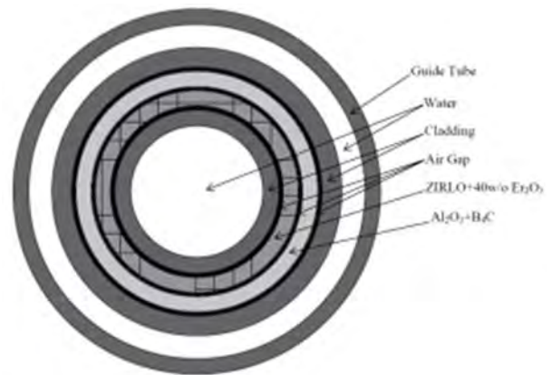
Fig. 3. MDBP design for WH fuel assembly type.
