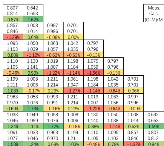
Fig. 5. Assembly power distribution of BOC
