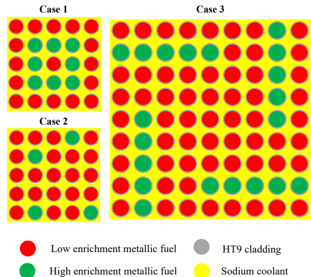
Figure 9 Specification of assembly problem, Case1~Case3
