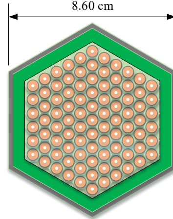
Fig. 2. Fuel assembly design diagram.
