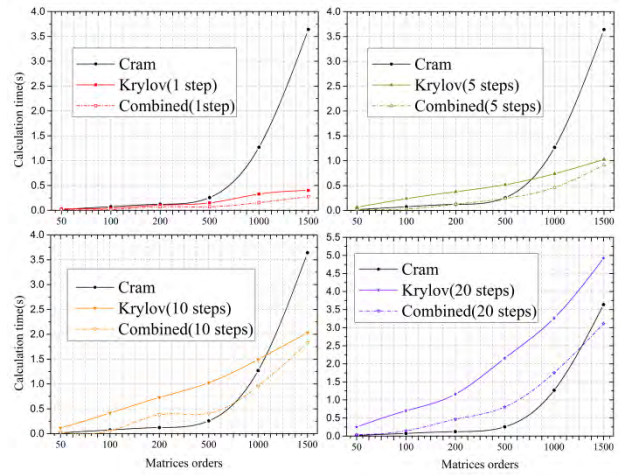
Fig. 1 Calculation time of random matrices
