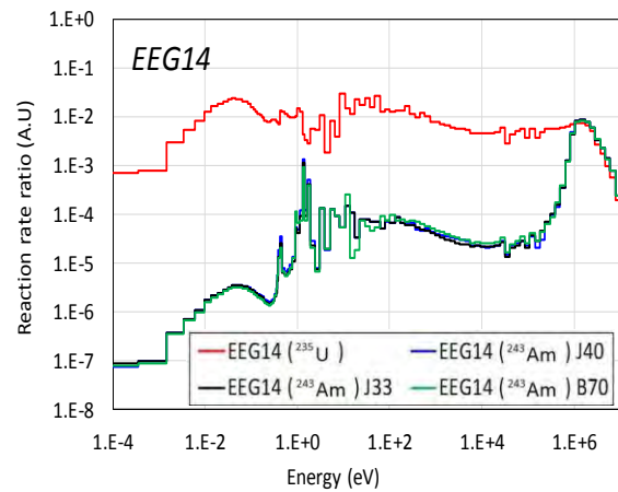
Fig. 5. Energy wise contribution of ^{243}\text{Am} and ^{235}\text{U} fission rate by MVP3 in EEG14.
