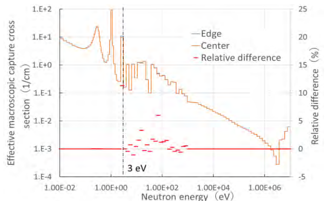
Fig. 4. Effect of position on effective macroscopic capture cross section
