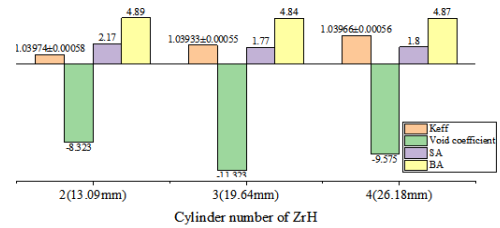
Fig. 14. k_{eff} , VC and axial PPF with ZrH thickness
