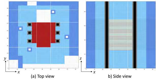
Fig. 3 Calculation geometry (A3/8" p36EU-NU).
