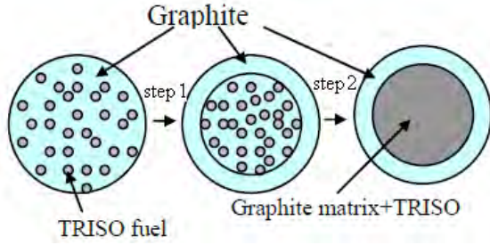
Fig. 4. The RPT Process
