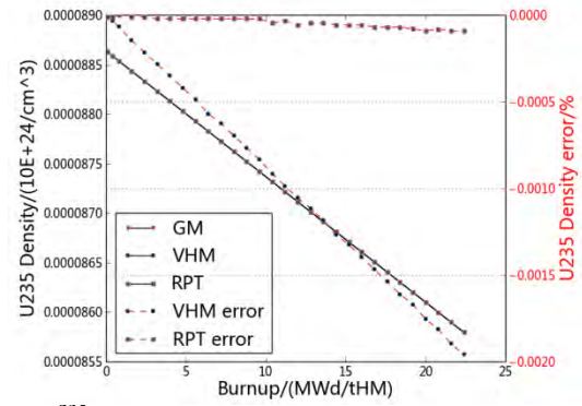
Fig. 5. k_{inf} and ^{235}\text{U} nuclide density as function of burnup in cells with different enrichments and different models
