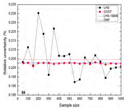
(a) ^{235}\text{U}-\sigma_{(n,\gamma)}
