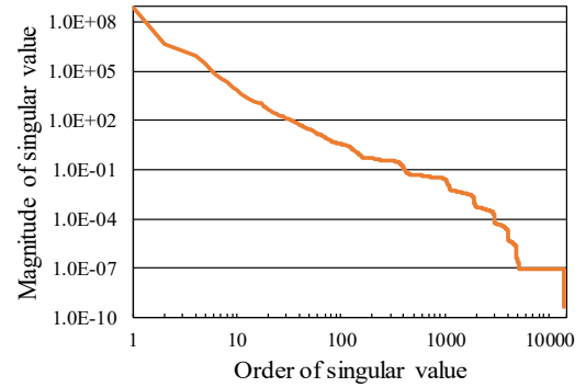
Fig. 4. The magnitude of singular values.
