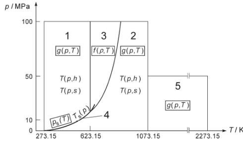
Fig. 2. Steam regions specified in IAPWS-IF97.
