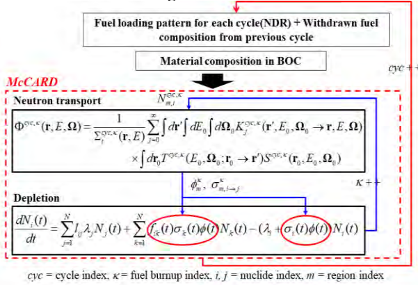
Fig. 2. Calculation procedure of whole core tracking method
