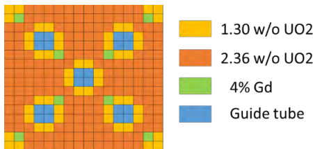
Fig. 2. Material configuration of a single assembly problem
