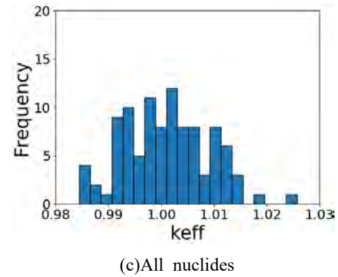
Fig. 1 The histogram of 100 k_{\text{eff}} in the RS method for 3 cases. The number of bins in the histograms is 20.
