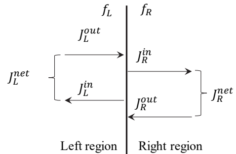
Fig 1. Relationship among partial and net currents
