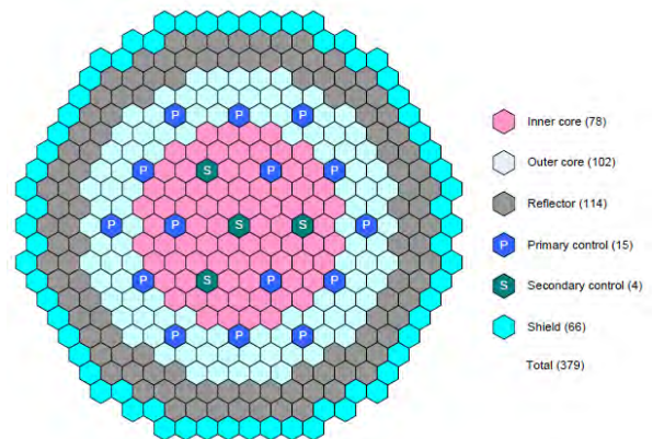
Fig. 4. ABR-1000 radial core layout.
