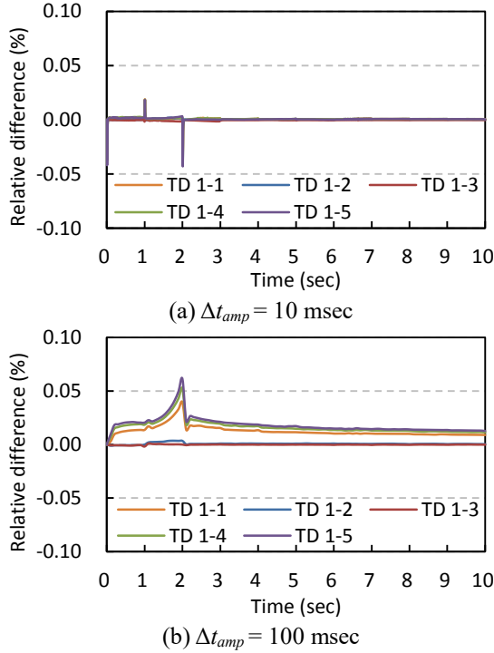
Fig. 4. Relative difference of the core power comparing to the reference solution
