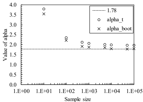
Fig. 3. Margin values of \alpha_t and \alpha_{boot} .
