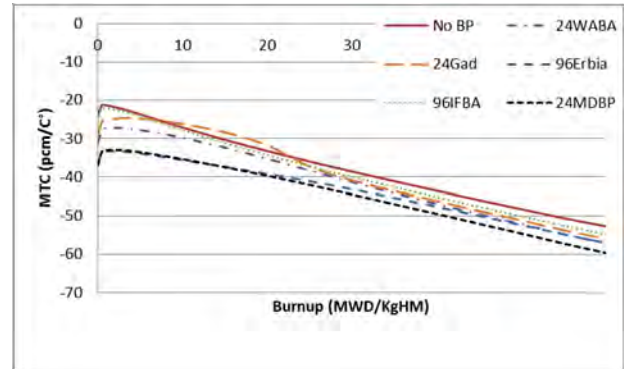
Fig. 10. Comparison of MTC for WH fuel assembly type.
