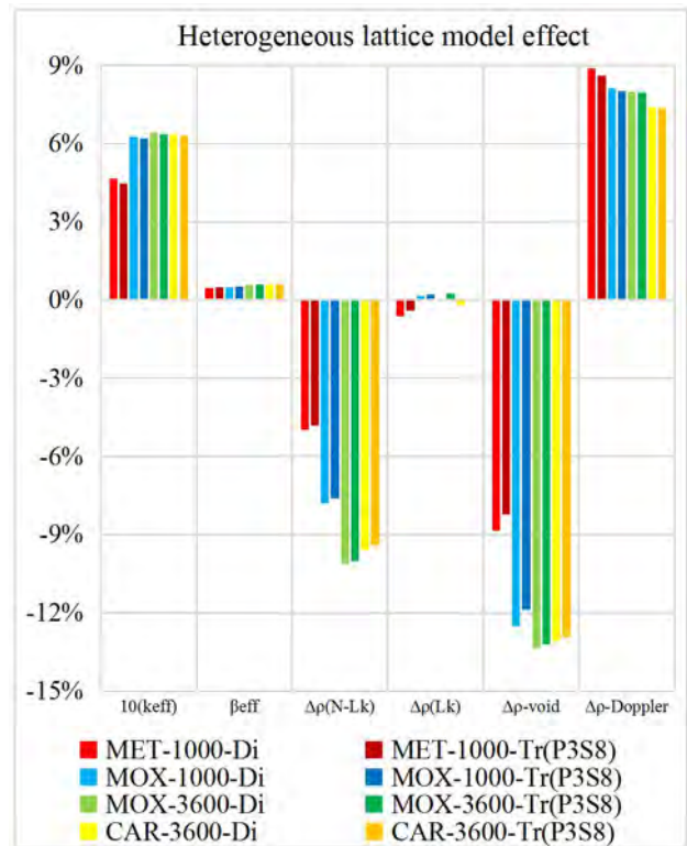
Fig. 3. Heterogeneous lattice model correction effect at BOC
