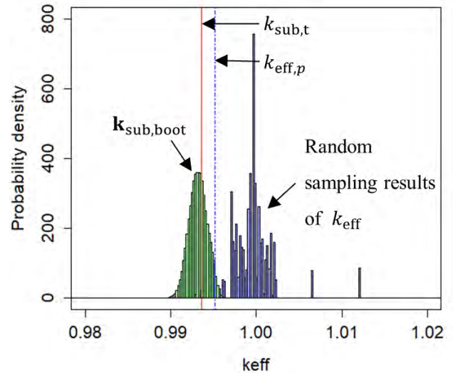
Fig. 4. Probability density distributions of random sampling results of k_{\text{eff}} , k_{\text{sub},\text{boot}} and k_{\text{sub},t} , k_{\text{eff},p} (Case 2)
