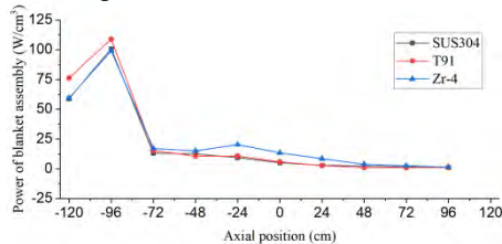
Fig. 17. Axial power distribution of BA with materials.
