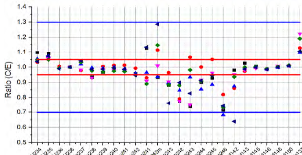
Fig. 6. C/E ratio – Ohi Unit 1&2 (all isotopes)
