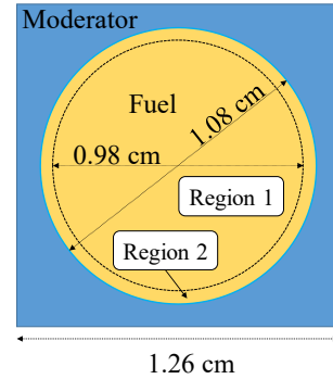
Fig. 1. Pin cell geometry
