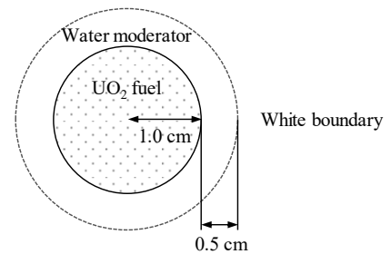
Fig. 1. Cell geometry and boundary condition.
