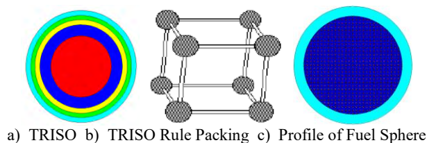
Fig.2 Schematic Diagram of TRISO Particle and Packing
