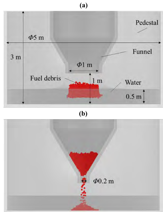
Figure. 3 The fuel debris falls to the bottom of the pedestal where the cooling water is accumulated during the fuel debris removal in case of the funnel outlet diameter (a) \phi 1 m, (b) \phi 0.2 m.
