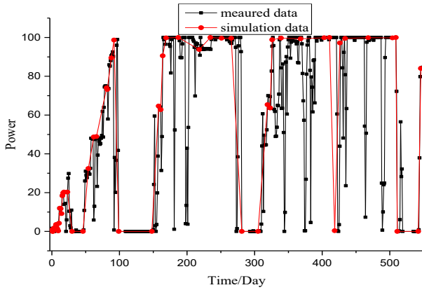
Fig. 1 power history of the first cycle (black) and the power follow approximation (red)
