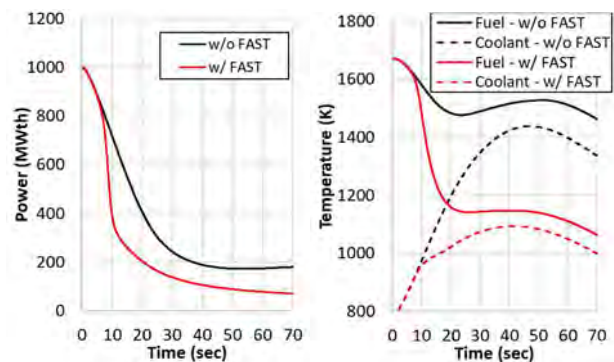
Fig. 4. Time evolution of the core power in ULOF
