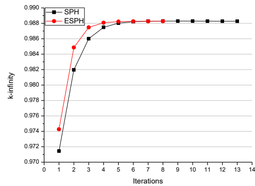
Fig. 3. k_{inf} convergence with SPH/ESPH iterations.
