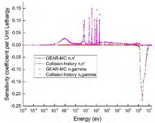
Fig 4. Sensitivity coefficients of ^{238}\text{U}
