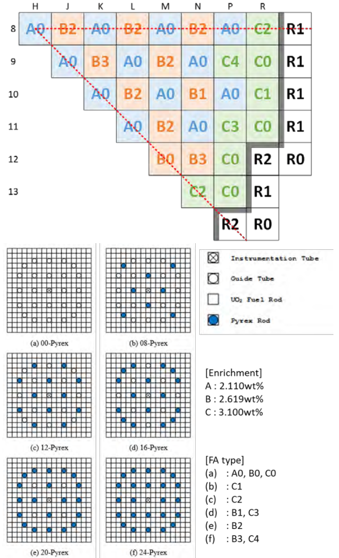
Fig. 1. 2-D VERA core and fuel assembly configuration.
