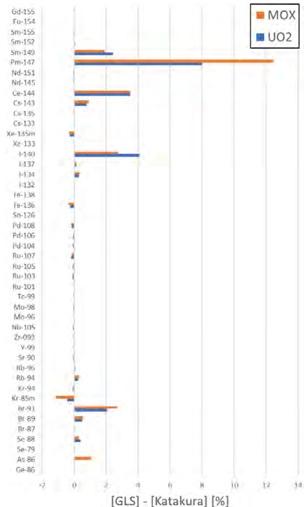
Fig. 3. Uncertainty difference due to adjustment method at 45 GWD/t
