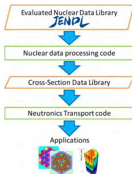
Fig.1. Calculation flow from evaluated nuclear data library to nuclear calculation.
