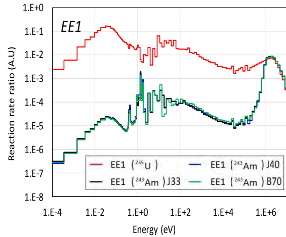
Fig. 4. Energy wise contribution of ^{243}\text{Am} and ^{235}\text{U} fission rate by MVP3 in EE1.
