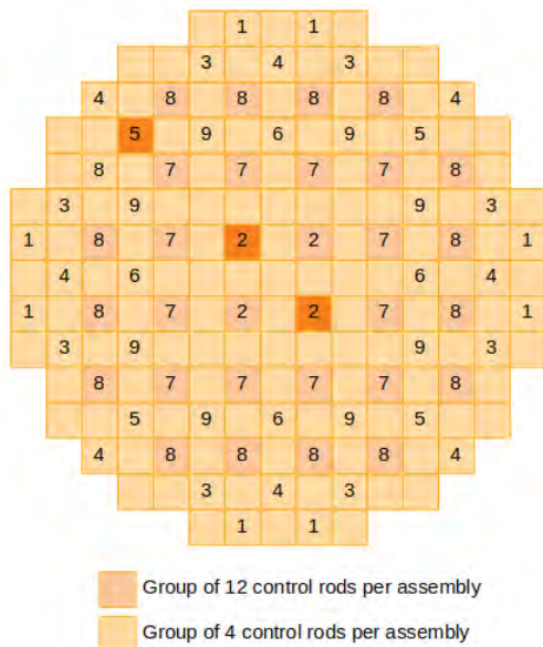
Fig.2. Control rods groups of OPR-1000 reactor core. Ejecting groups are colored by orange.
