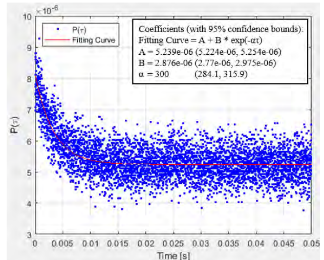
Fig. 4. Rossi- \alpha fitting curve for SCR1
