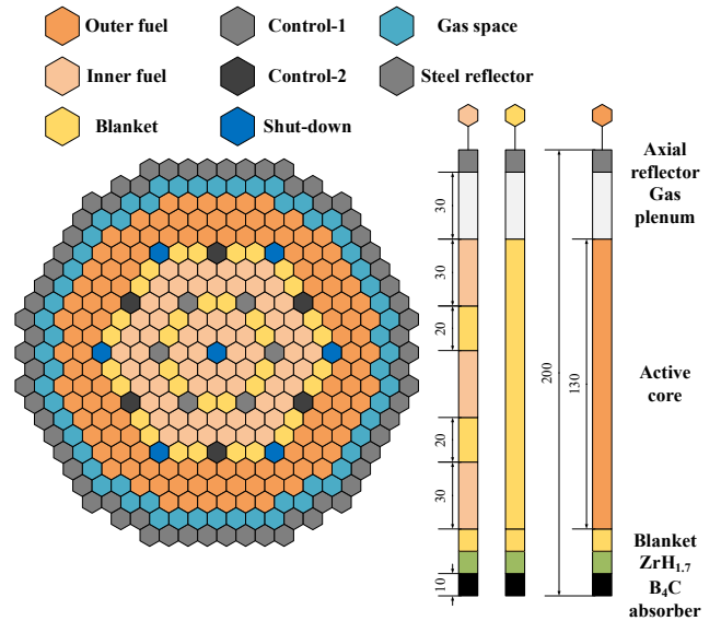
Fig. 3. Layout of gas-cooled core design
