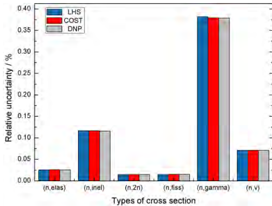
Fig. 2. Comparison of uncertainty results of different methods when the 6 reaction channels \sigma_{(n,elas)} , \sigma_{(n,inel)} , \sigma_{(n,2n)} , \sigma_{(n,f)} , \sigma_{(n,\gamma)} , \sigma_{(n,v)} of ^{238}\text{U} are perturbed separately
