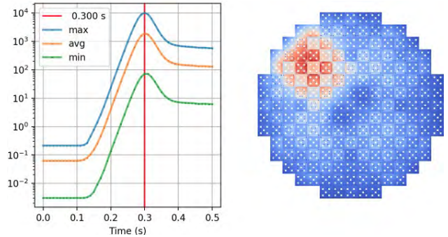
Fig.4. Linear power pulse (W/cm) and shape function at the middle height of reactor core
