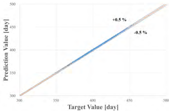
Fig. 9. Training result of cycle length using M1NR
