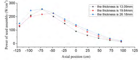
Fig. 12. Axial power of SA with moderator thicknesses.
