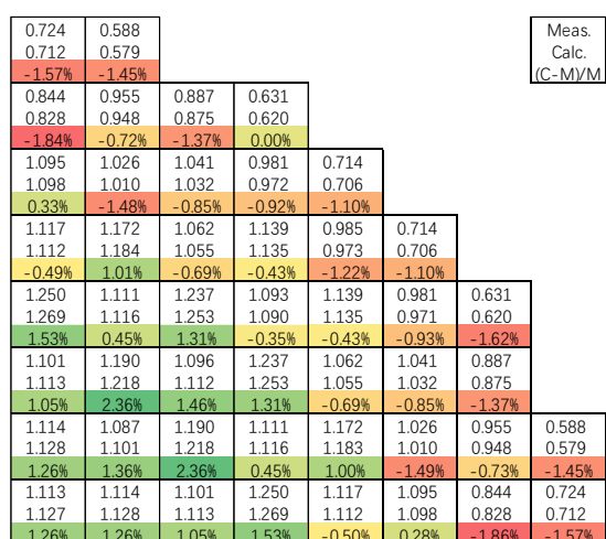
Fig. 6. Assembly power distribution of MOC
