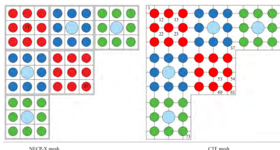
Fig. 1. Model of quarter core.
