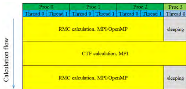
Fig. 2. An example for demonstrating the innovative hybrid coupling method for internal coupling between RMC and CTF.
