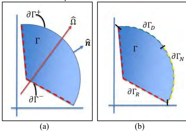
Fig. 1. (a) Geometrical domain \Gamma for transport theory: neutron direction \hat{\Omega} , incoming boundary \partial\Gamma^- , outgoing boundary \partial\Gamma^+ and normal vector \hat{n} are indicated. (b) Geometrical domain for diffusion calculations, with Dirichlet, Neumann, and Robin boundaries indicated as \partial\Gamma_D , \partial\Gamma_N and \partial\Gamma_R
