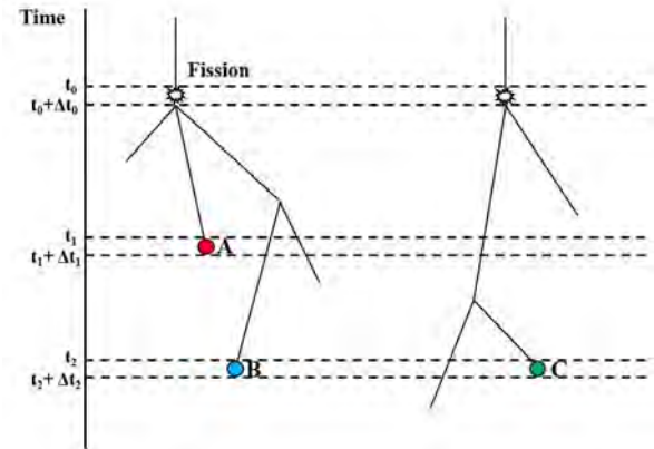
Fig. 1. Random branching process of fission neutron
