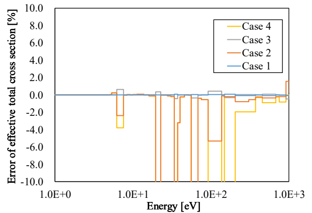
Fig. 5. Error of U238 effective total cross section in 172 XMAS energy group structure (Region 2, outer region of pellet).
