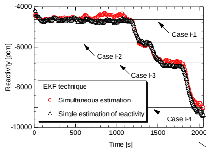
Fig. 5 Comparison of reactivity estimations in beam swing transient experiment.
