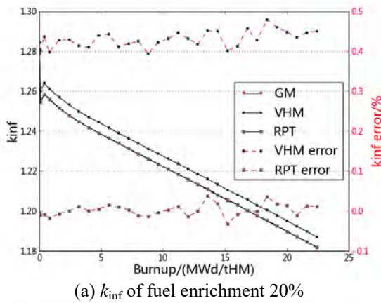
Fig. 5. k_{inf} and ^{235}\text{U} nuclide density as function of burnup in cells with different enrichments and different models
