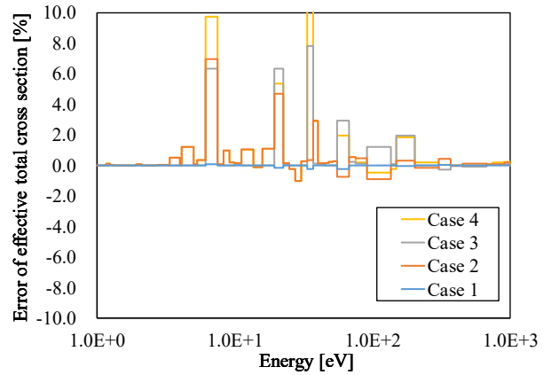
Fig. 4. Error of U235 effective total cross section in 172 XMAS energy group structure (Region 2, outer region of pellet).
