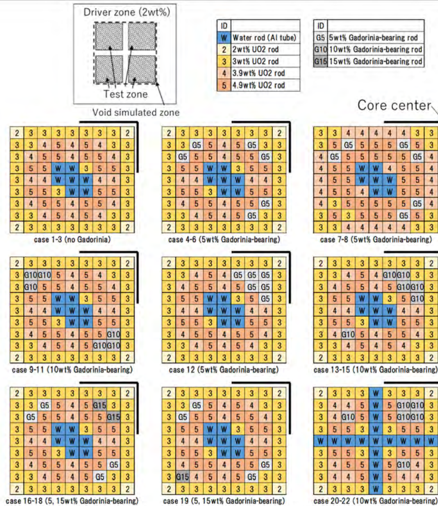
Fig. 3. Core configuration
