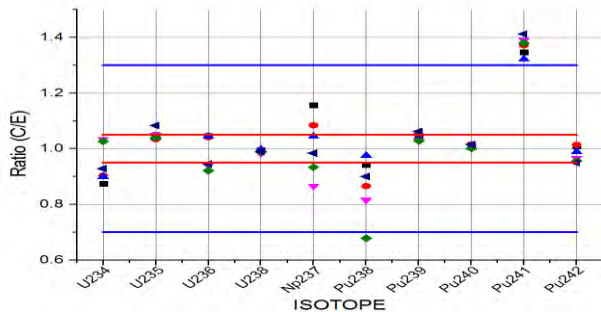
Fig. 4. C/E ratio – Calvert Cliffs Unit 1 (actinide)
