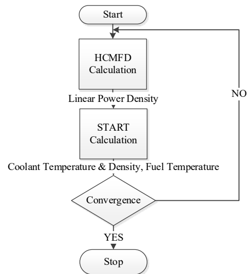
Fig. 2: Flow chart for coupled calculations
