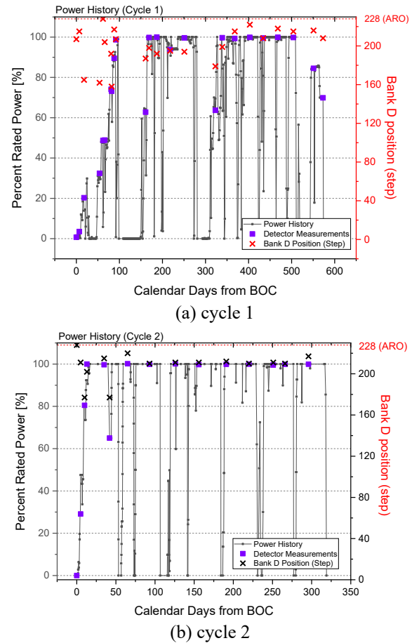
Fig. 2. Power history and control rod bank positions
