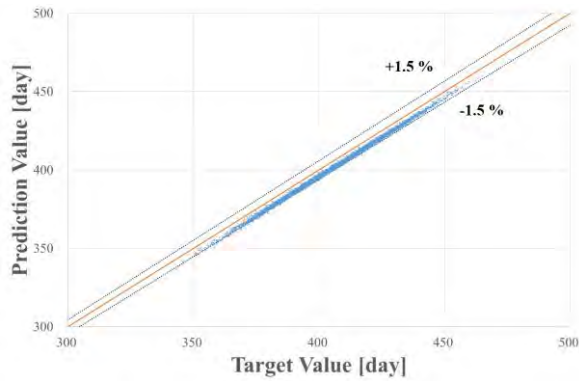
Fig. 8. Training result of cycle length using M1
