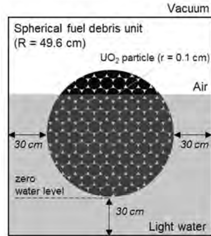
Fig. 1. Cross-sectional view of system (not to scale).
