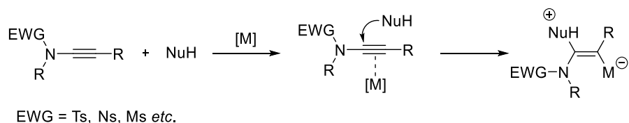
Scheme 14. Transition metal-catalyzed reaction of ynamides
