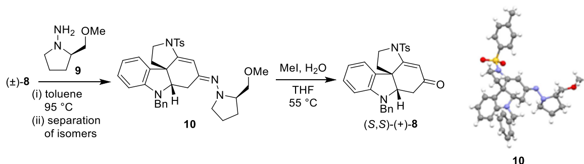
Scheme 3. Determination of absolute configuration of 8
