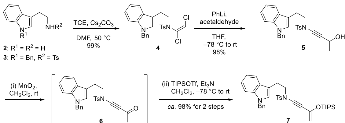
Scheme 2. Synthesis of indole-ynamide having a silyl enol ether
