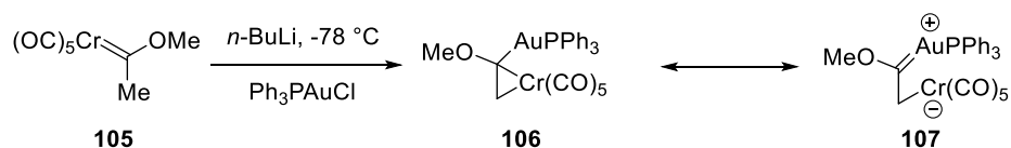
Scheme 21. First example of a gold carbenoid complex
