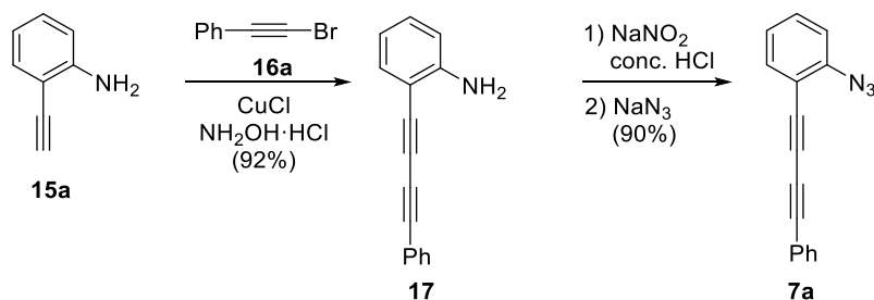
Scheme 4. Synthesis of conjugated diyne 7a
