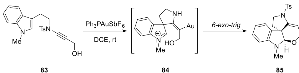
Scheme 16. Gold(I)-catalyzed intramolecular cascade cyclization of an indolyl-ynamide
