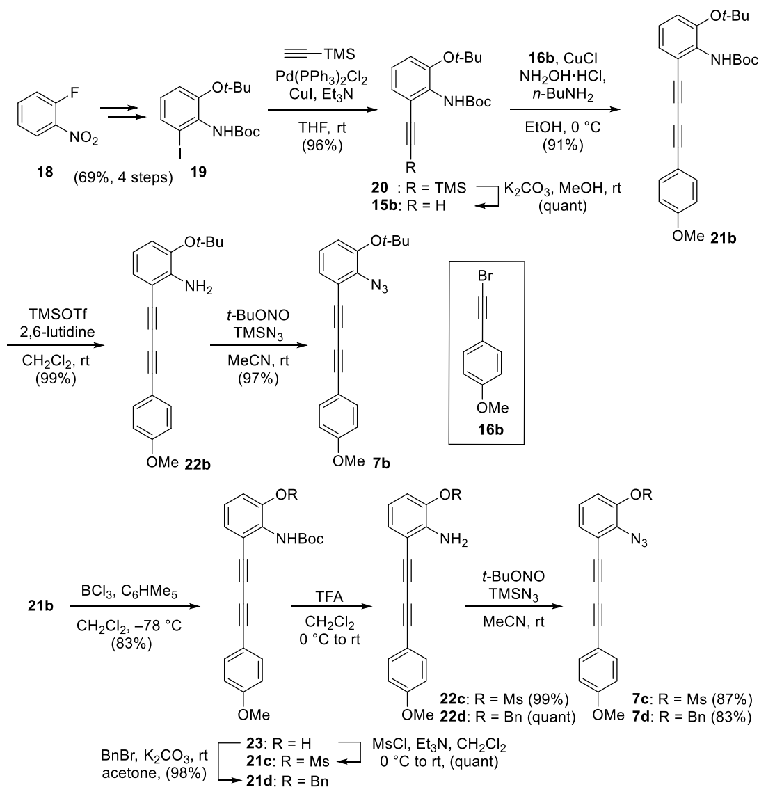
Scheme 5. Synthesis of azidodiyne 7b-d
