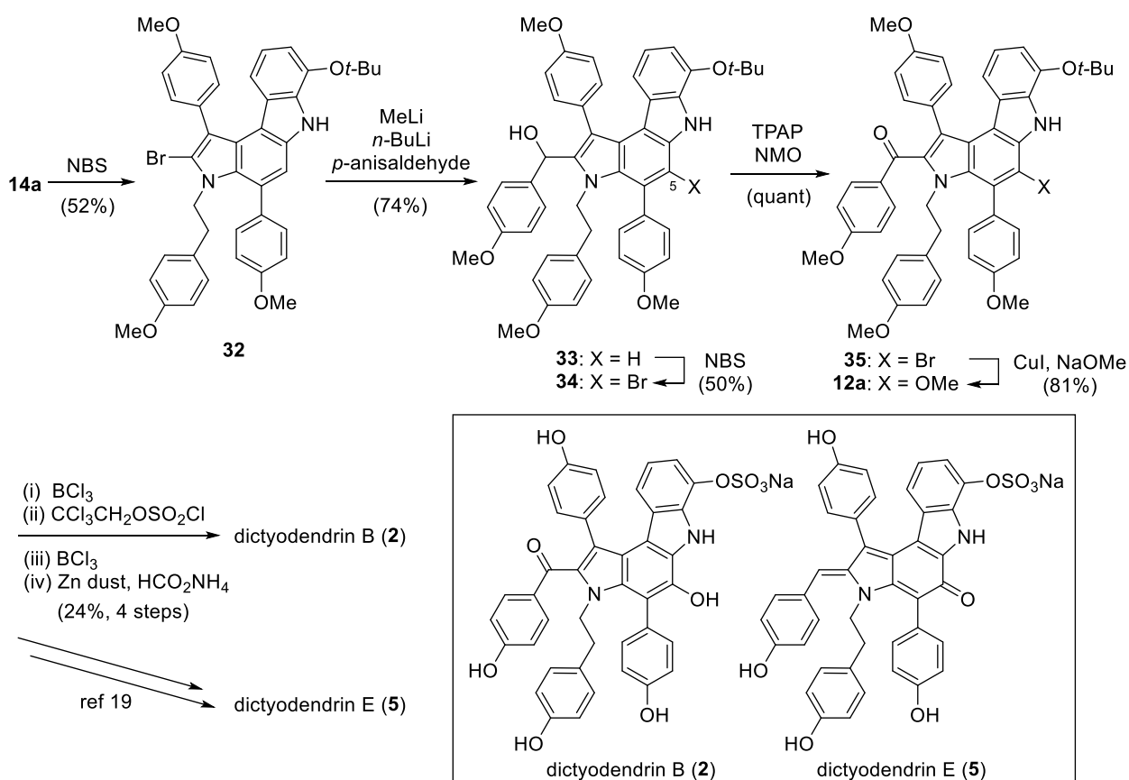
Scheme 9. Total syntheses of dictyodendrins B and E
