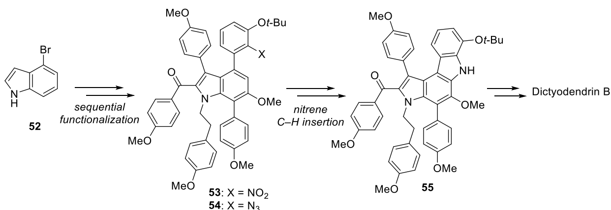
Scheme 8. Total synthesis of dictyodendrin B by Gaunt 24
