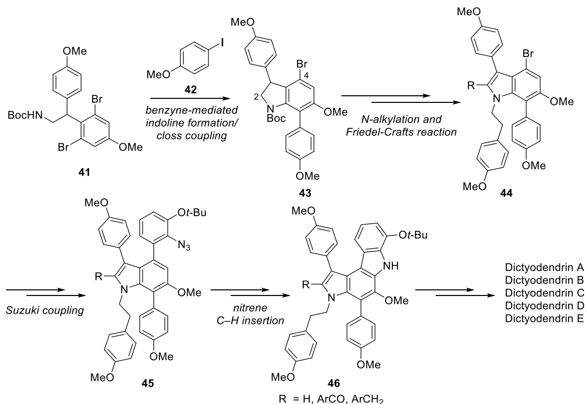
Scheme 6. Total synthesis of dictyodendrins A-E by Tokuyama 20,21
