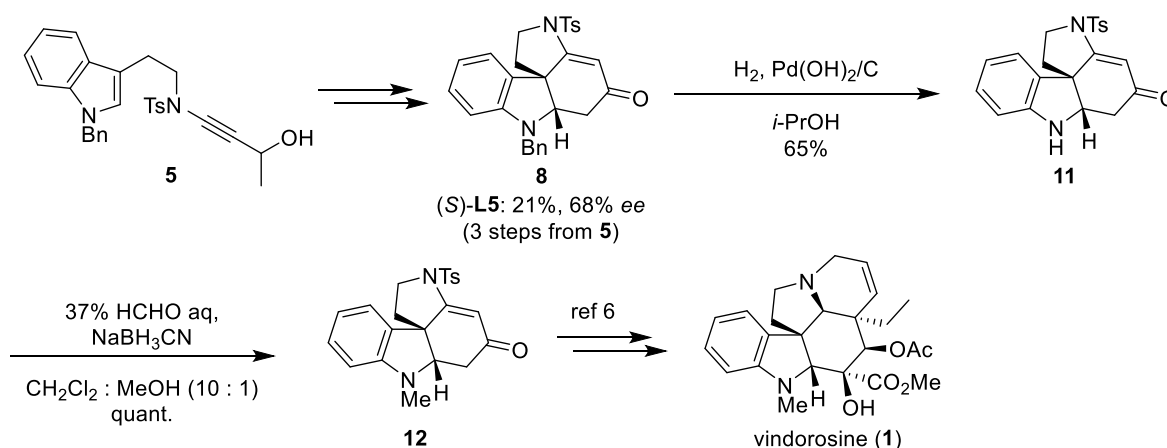
Scheme 4. Formal synthesis of vindorosine
