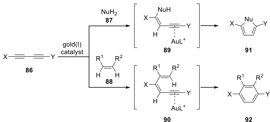
Scheme 17. Gold(I)-catalyzed tandem cyclization of conjugated diynes
