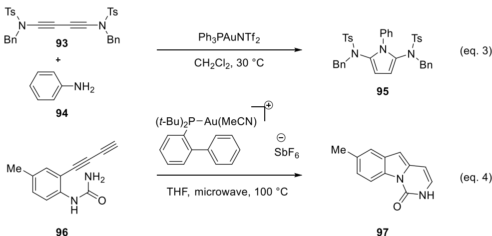
Scheme 18. Gold(I)-catalyzed construction of heterocycles via conjugated diynes
