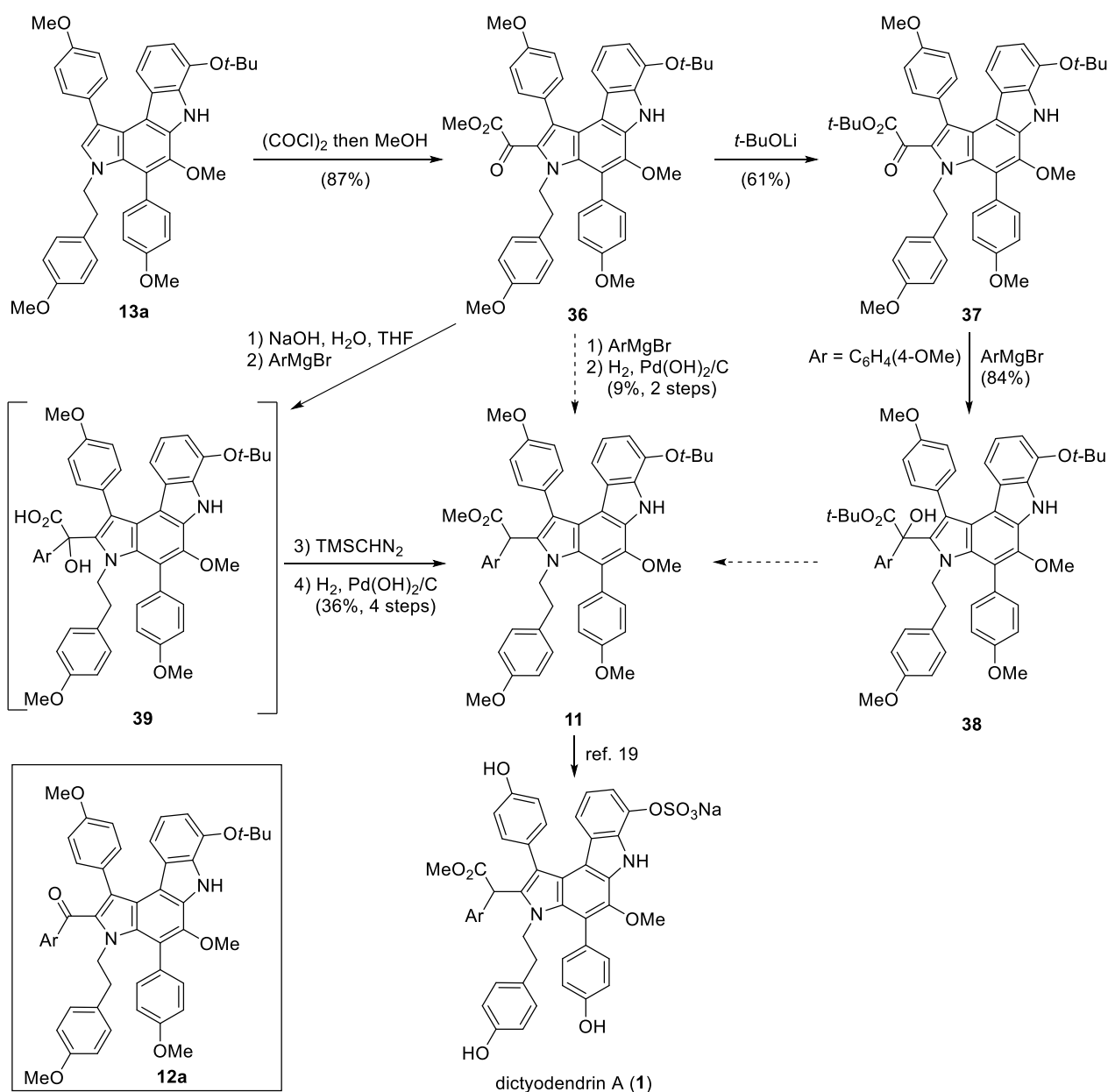
Scheme 10. Formal synthesis of dictyodendrin A
