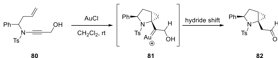
Scheme 15. Gold-catalyzed construction of nitrogen-containing bicyclic compounds
