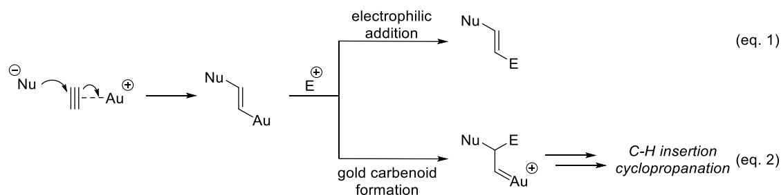
Scheme 13. Gold-catalyzed reactions of alkynes
