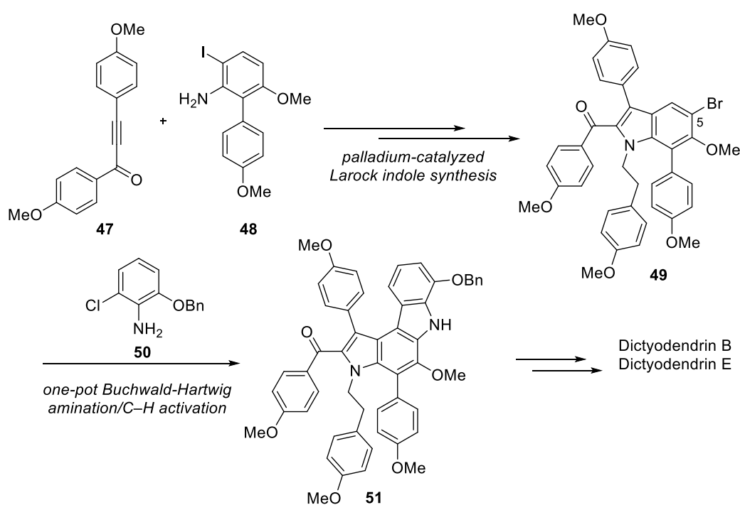
Scheme 7. Total synthesis of dictyodendrins B and E by Jia 22,23
