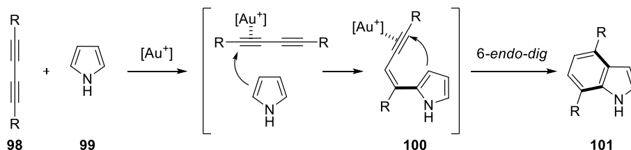
Scheme 19. Gold(I)-catalyzed cascade annulation reported by the author's group
