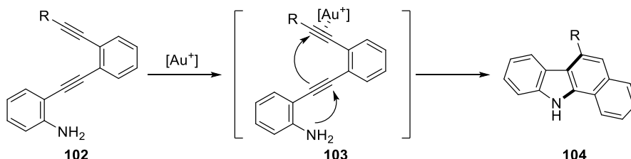
Scheme 20. Gold(I)-catalyzed cascade annulation reported by the author's group
