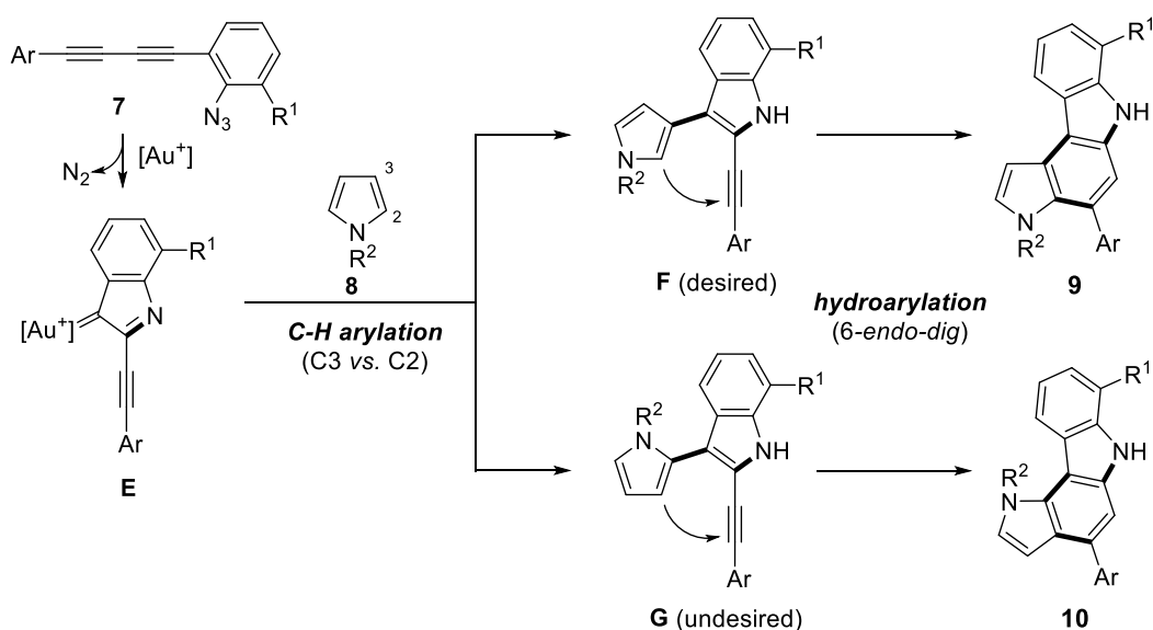
Scheme 2. The author's strategy for the construction of the pyrrolo[2,3- c ]carbazole core structure
