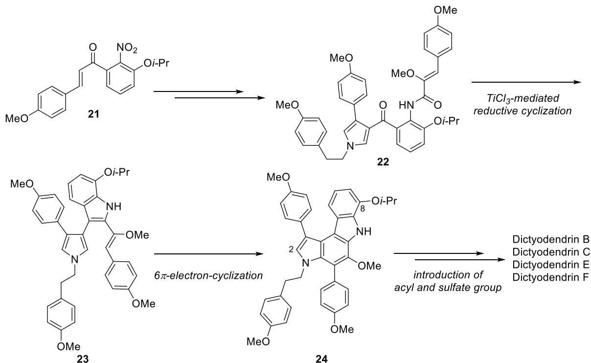
Scheme 2. First total synthesis of dictyodendrins B, C, E, and F by Fürstner 13–15
