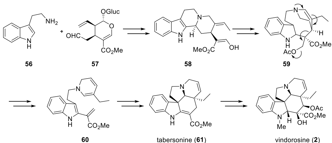
Scheme 9. Proposed biosynthesis of vindorosine
