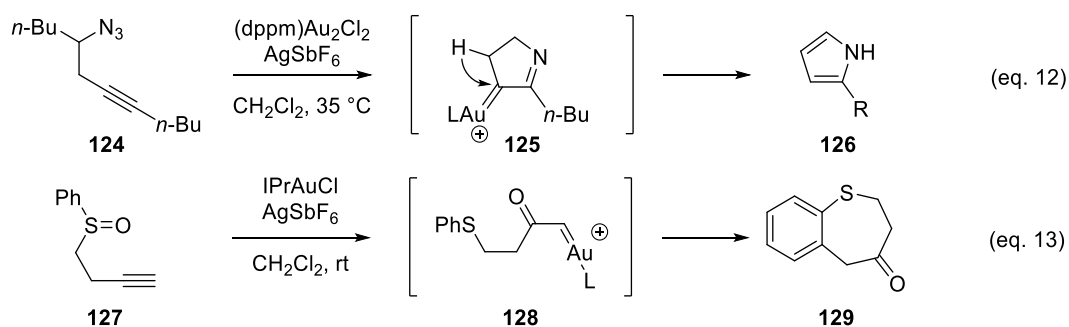
Scheme 24. Gold(I)-catalyzed intramolecular Schmidt reaction and sulfoxide rearrangement
