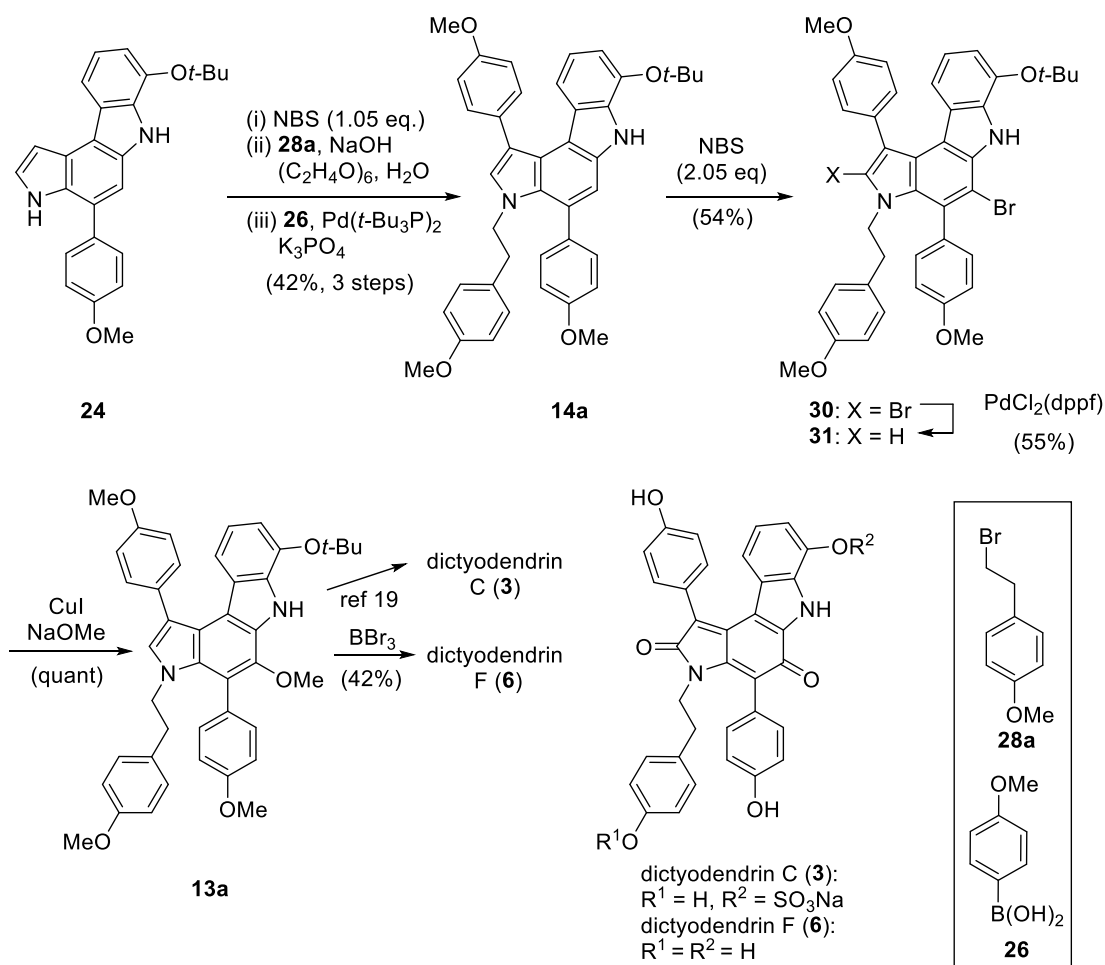
Scheme 7. Total syntheses of dictyodendrins C and F
