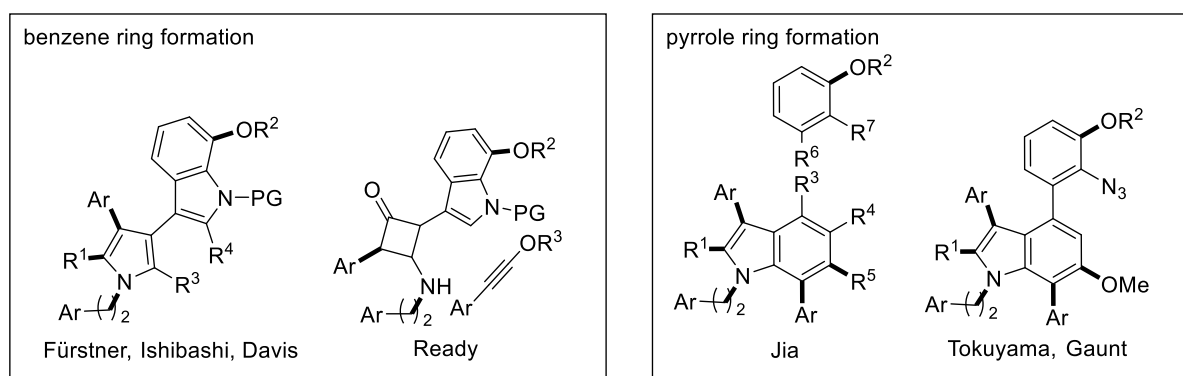
Figure 4. Two main synthetic strategies for the dictyodendrin scaffold
