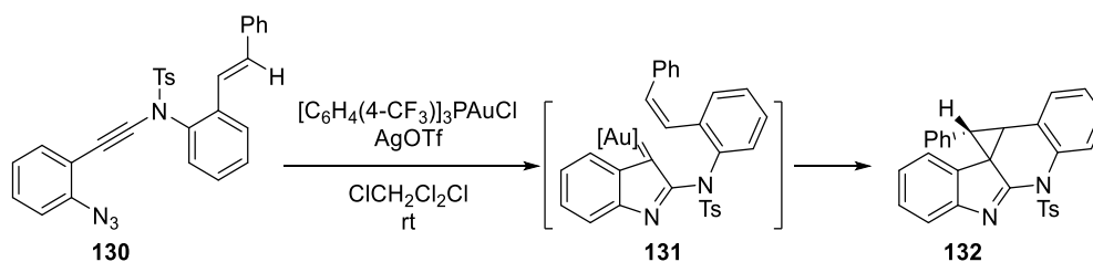
Scheme 25. Gold(I)-catalyzed intramolecular Schmidt reaction of (azido)ynamides
