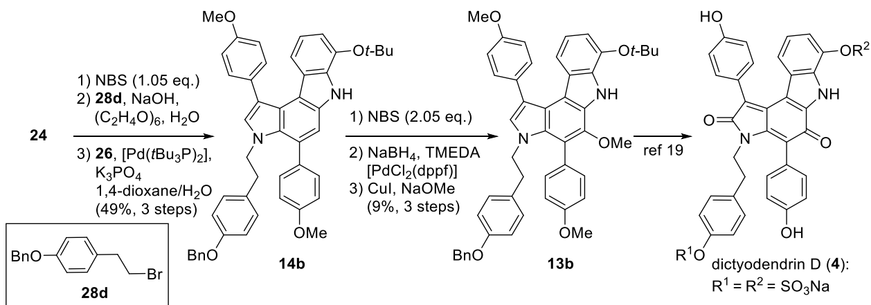
Scheme 8. Total synthesis of dictyodendrin D
