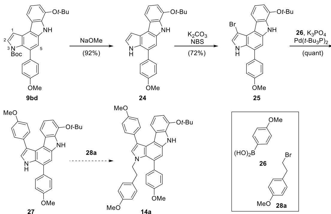
Scheme 6. Attempt at the synthesis of 14a
