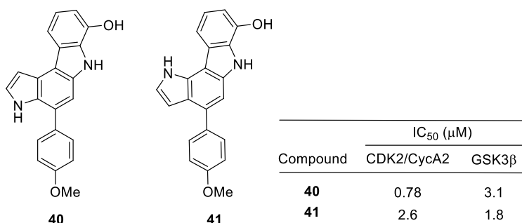
Figure 3. Inhibition of CDK2/CycA2 and GSK3 \beta
