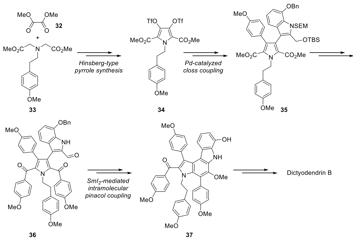
Scheme 4. Formal total synthesis of dictyodendrin B by Ishibashi 17,18
