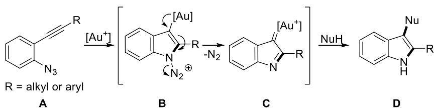
Scheme 1. Gold(I)-catalyzed intramolecular acetylenic Schmidt reaction
