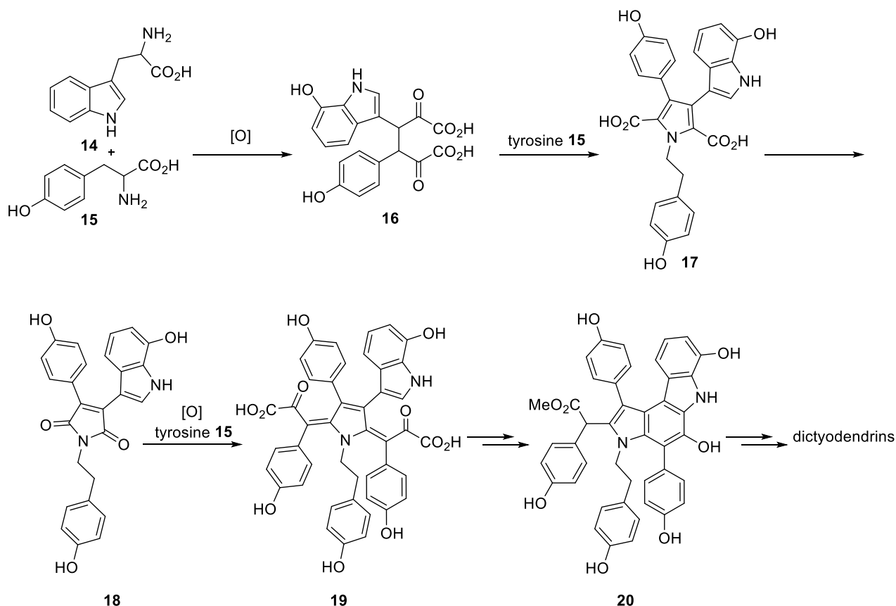
Scheme 1. Proposed biosynthetic route to the dictyodendrins
