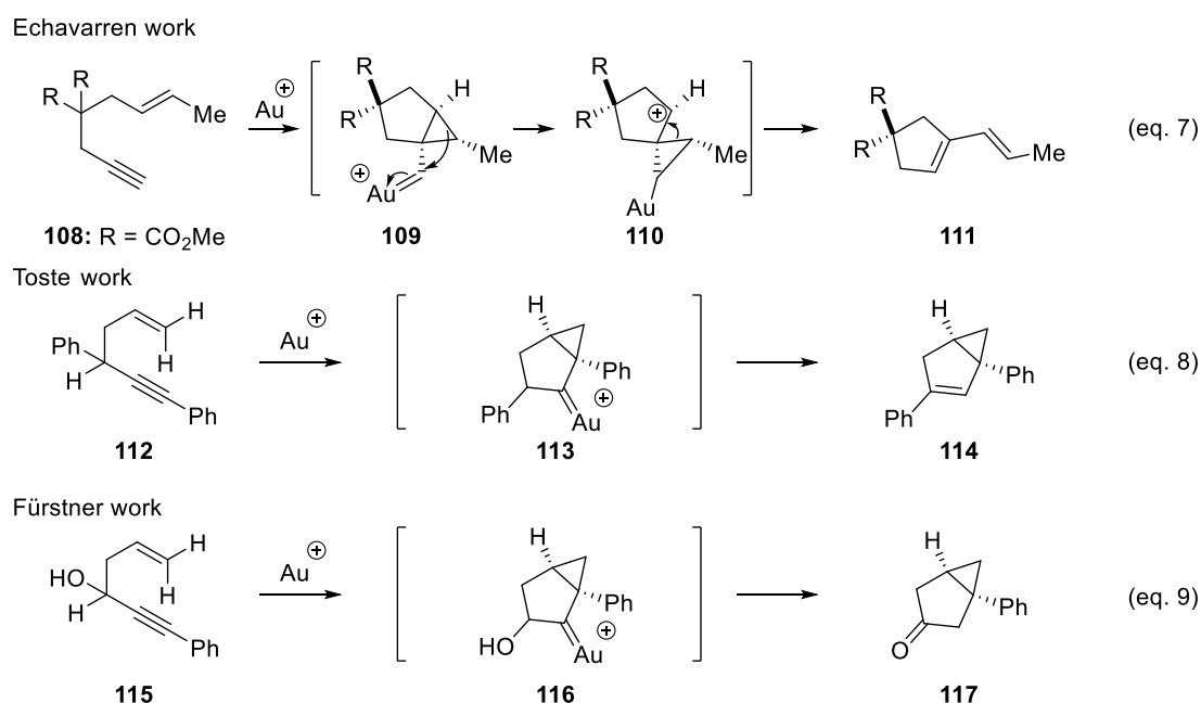
Scheme 22. Gold(I)-catalyzed cycloisomerization-type reaction of enynes
