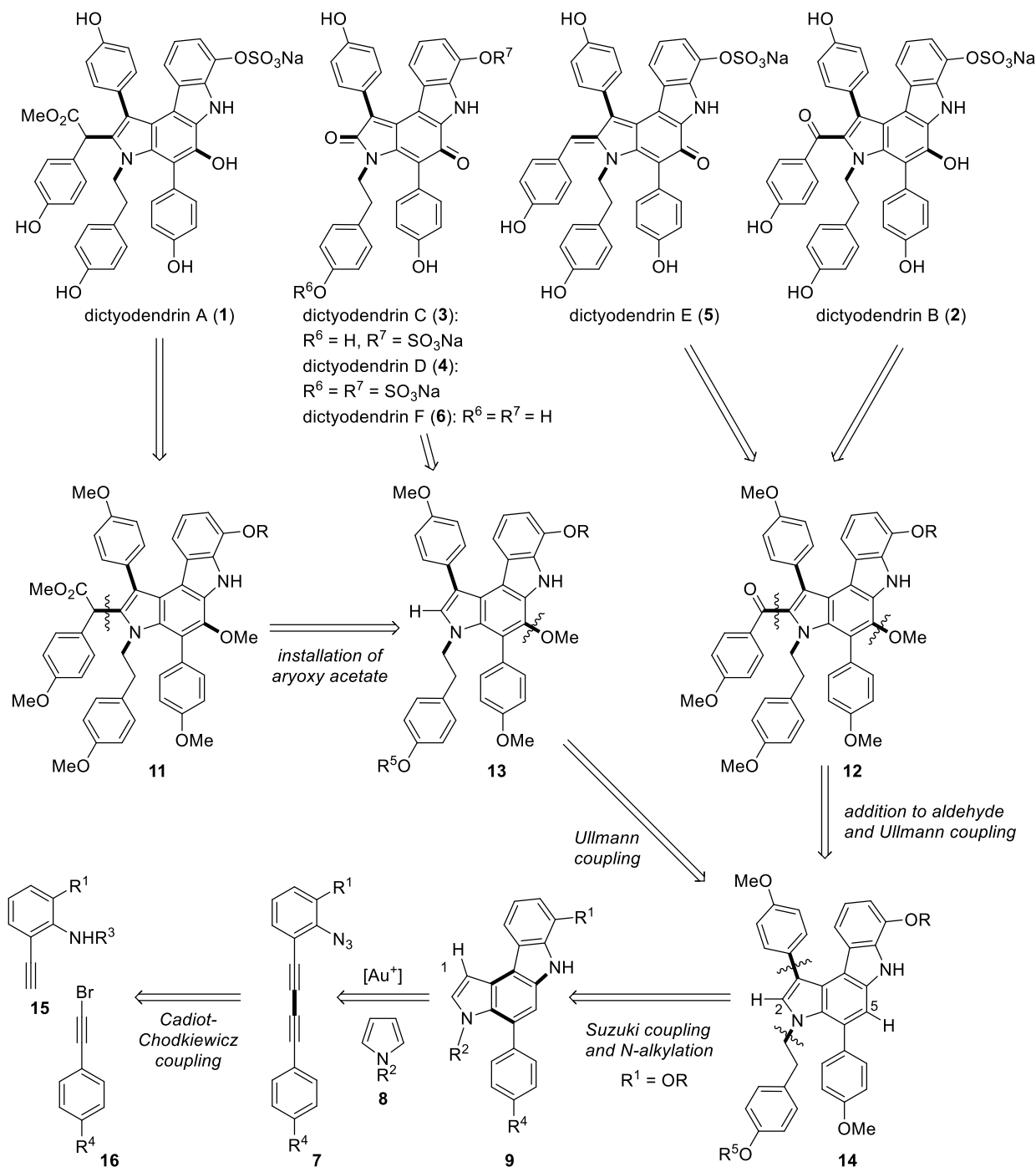
Scheme 3. Retrosynthetic analysis of dictyodendrins.
