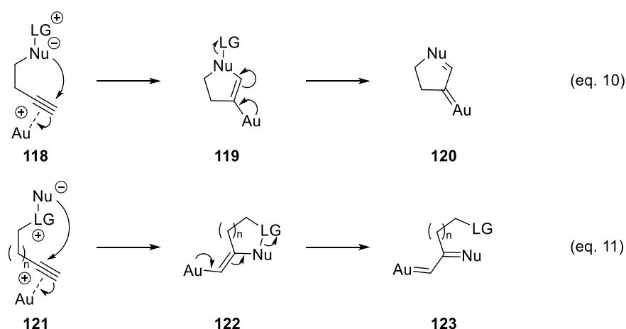
Scheme 23. Generation of gold carbenoids from ylide-tethered alkynes
