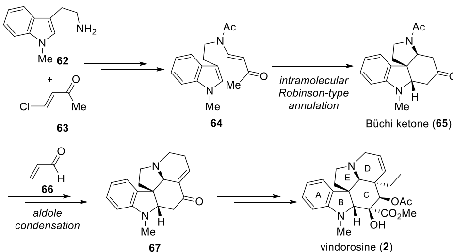
Scheme 10. First total synthesis of vindorosine by Büchi in 1971 28
