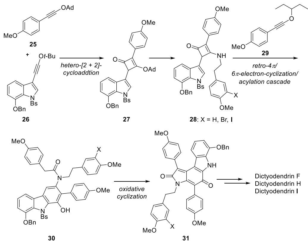
Scheme 3. First total synthesis of dictyodendrin H and I by Ready 16
