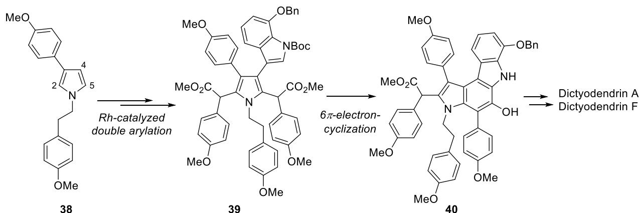
Scheme 5. Total synthesis of dictyodendrins A and F by Yamaguchi, Itami, and Davis 19
