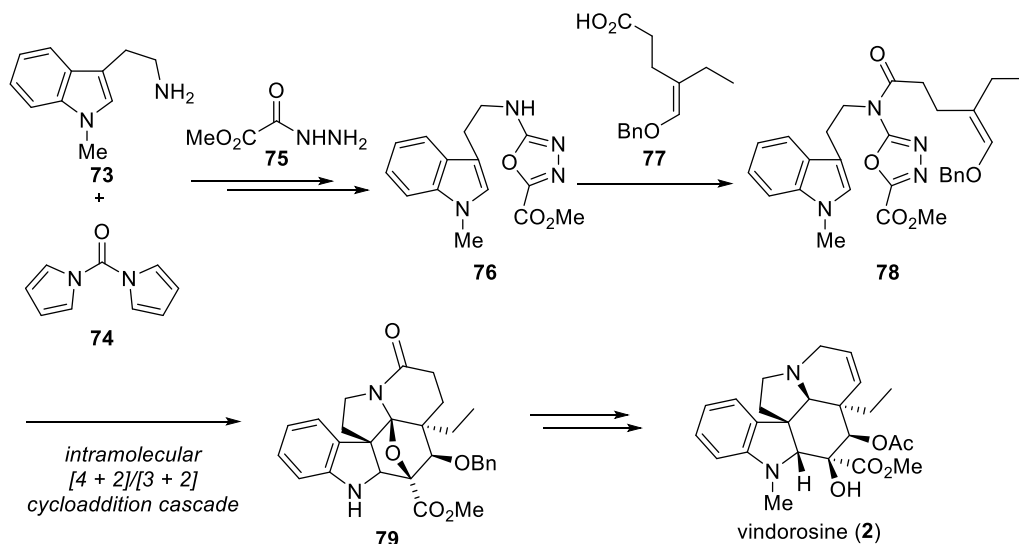
Scheme 12. Asymmetric total synthesis of vindorosine by Boger in 2006 32,33
