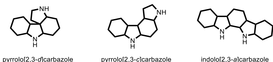
Figure 1. Pyrrolocarbazole scaffolds
