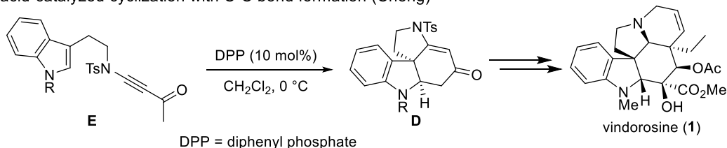
Scheme 1. Intramolecular cascade reaction of indole-ynamides
