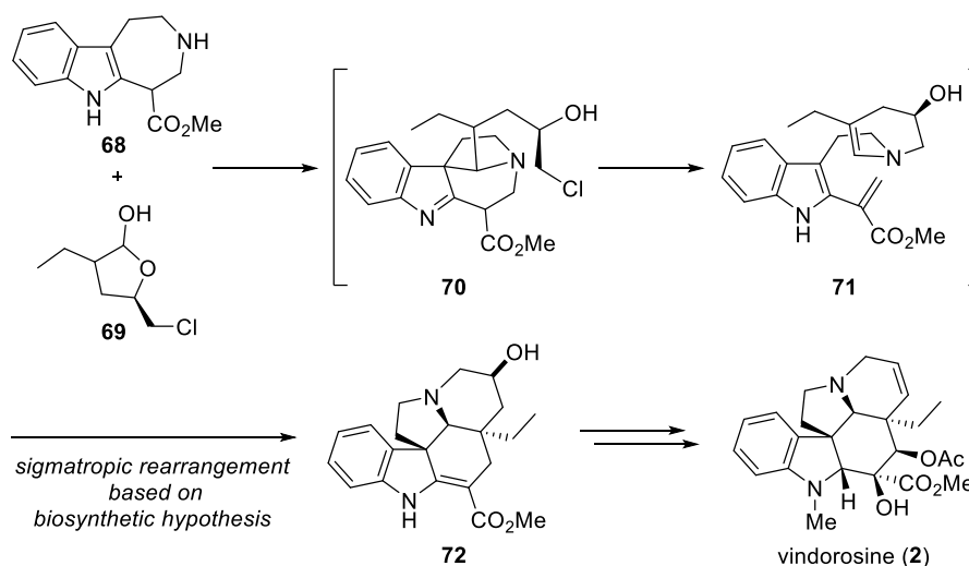
Scheme 11. First asymmetric total synthesis of vindorosine by Kuehne in 1986 31
