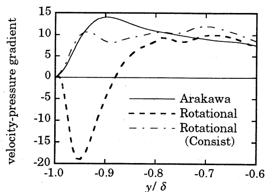
Fig.3 y-distribution of velocity-pressure gradient terms
