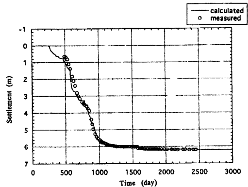
Fig. 12. Measured and calculated settlements of the alluvium at No. 1 point
