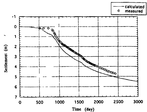
Fig. 13. Measured and calculated settlements of the diluvial deposit at No. 1 point
