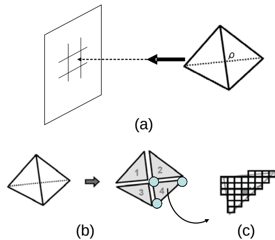
Fig.1 Concept of the SPT rendering
