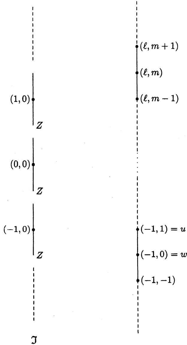
FIGURE 2. Algebra \mathcal{J} (left) and its magnified detail (right)
