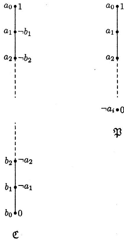
FIGURE 1. Chang's chain \mathcal{C} and product algebra \mathfrak{P}
