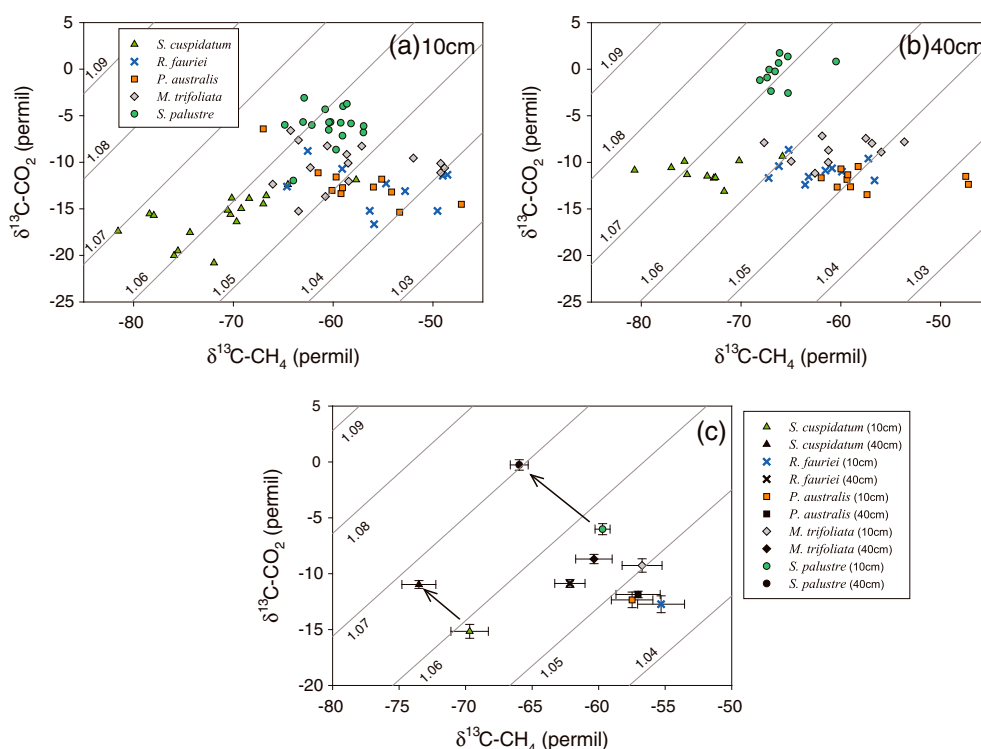
Figure 9. Crossplots of \delta^{13}\text{C} data from \text{CH}_4 and \text{CO}_2 for each habitat type at (a) 10 cm (a), (b) 40 cm, and (c) averaged ( C_i \pm \text{SE} ). The dashed lines indicate the apparent fractionation between \text{CO}_2 and \text{CH}_4 ( \alpha ) calculated by the ratio of (\delta^{13}\text{C-CO}_2 + 10^3)/(\delta^{13}\text{C-CH}_4 + 10^3) .
