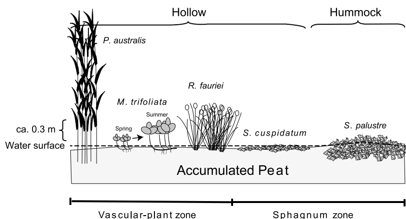
Figure 3. Schematics of cross-sectional diagram of habitat types on the floating mat in Mizorogaike Pond (summer period).
