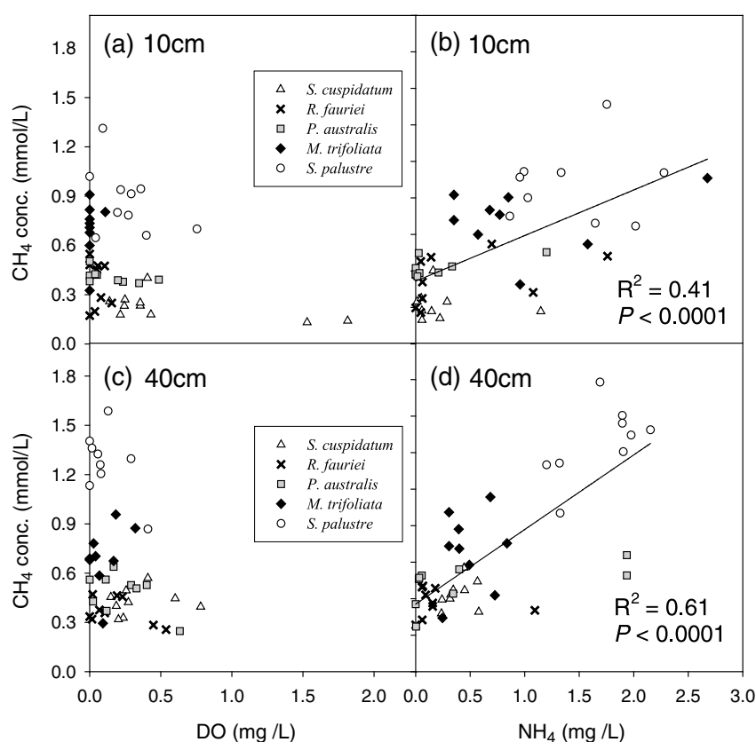
Figure 7. (a and c) Relationships between dissolved oxygen and (b and d) ammonium concentration, and CH 4 concentration.
