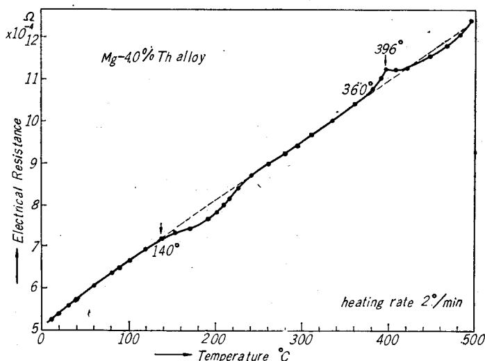
Fig. 1. Electrical resistance change of Mg-4.0%Th alloy in heating at a constant rate. (2°C/min)
