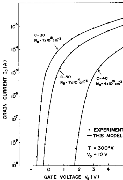
Figure 3.4 Comparison of the model and experiments of the log I_D - V_G characteristics in samples having 5030-Å oxide thickness.
