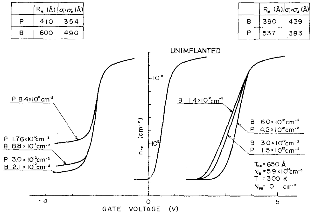
Figure 3.24 Comparison of the shift of \log n_{SF} - V_G curve due to single and double-layer impurities. The main impurity is implanted in the surface side.
