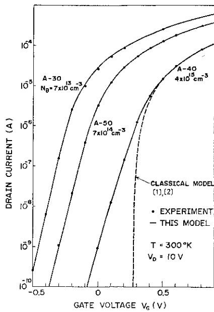
Figure 3.2 Comparison of the model and experiments of the log I_D - V_G characteristics in samples having 675-Å oxide thickness.
