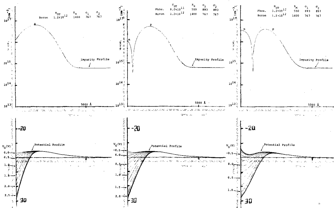
Figure 3.32 Potential profiles corresponding to the case shown in Fig. 3.31.
