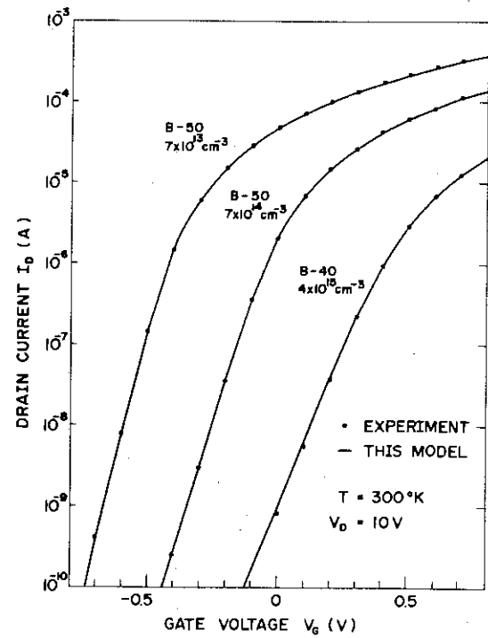
Figure 3.3 Comparison of the model and experiments of the log I_D - V_G characteristics in samples having 1470-Å oxide thickness.
