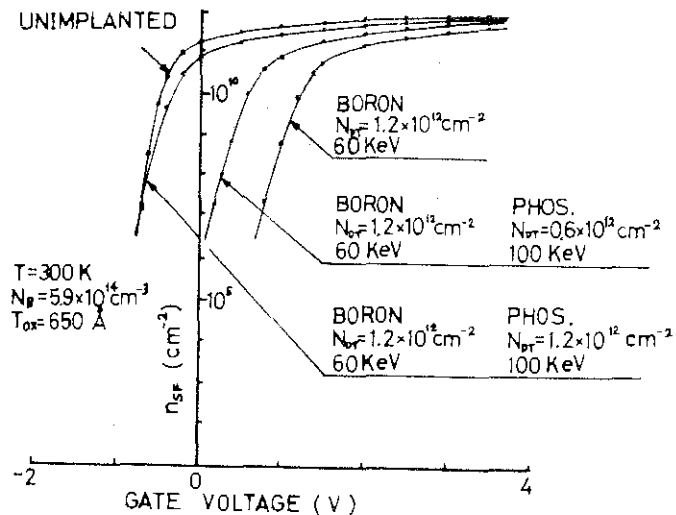
Figure 3.33 Experimental results of \log n_{SF}-V_G curves for the condition shown in Fig. 3.31.
