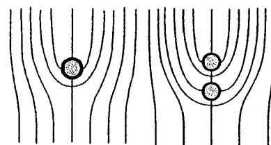
Fig. 1: Director field of LC with spherical particles.
