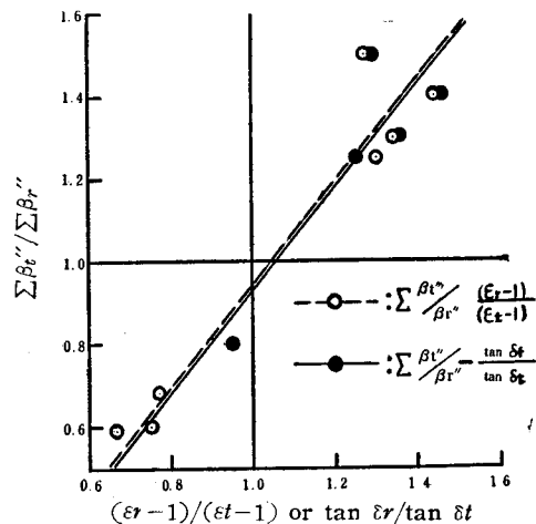
Fig 5. Anisotropy-degree of integral shrinkage in transverse section ( \sum \beta_t''/\sum \beta_r'' ) of the isolated spring- and summerwood of a few coniferous woods plotted against the anisotropy-degree of dielectric constant and dielectric loss ((\epsilon_r-1)/(\epsilon_t-1), \tan \delta_r/\tan \delta_t) in oven dried condition
