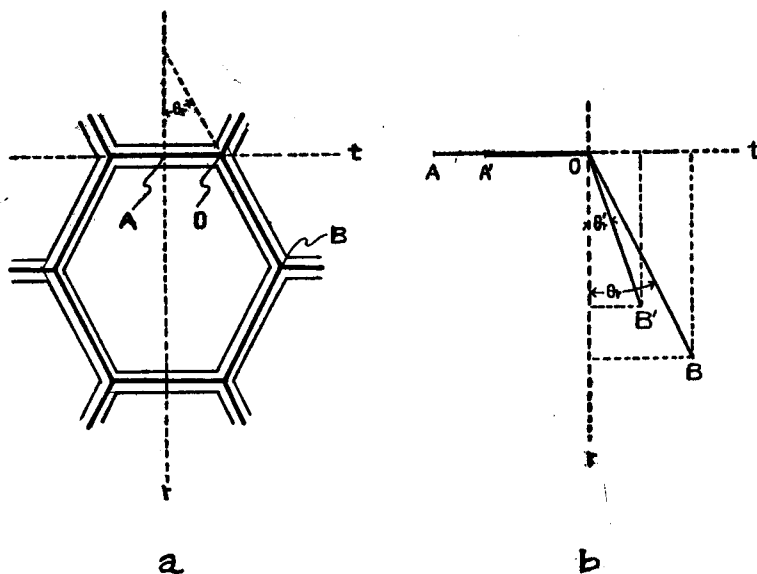
Fig. 3. Schematic cross section of a springwood tracheid illustrating the shape of a cell (a) and the deformation of tangential and radial wall in the case of shrinkage (b)
