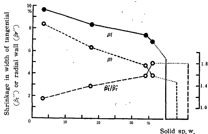
Fig 6. Relations between the delignification and the shrinkage in width of tracheid cell-wall — Springwood of Sugi
