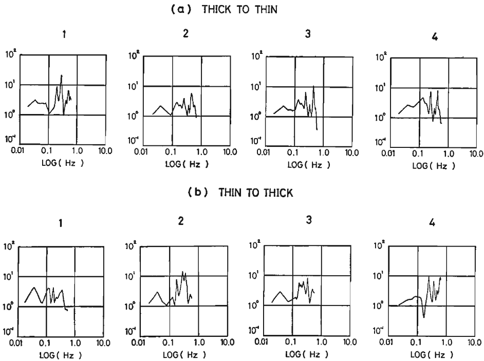
Fig. 12: Theoretical spectral ratios of the radial to vertical component of the ground motions at the free surface for the incident plane SV -waves. (a): the spectral ratios for the SV -wave from the thick layer side, (b): those from the thin layer side.
