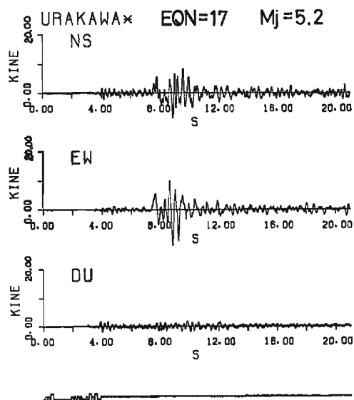
Fig. 8: An example of ground motions observed at URK station (the largest aftershock)
