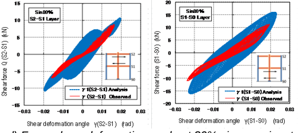
d) Force-shear deformation angle at 80% sin wave input. (blue: analysis red: observation)
