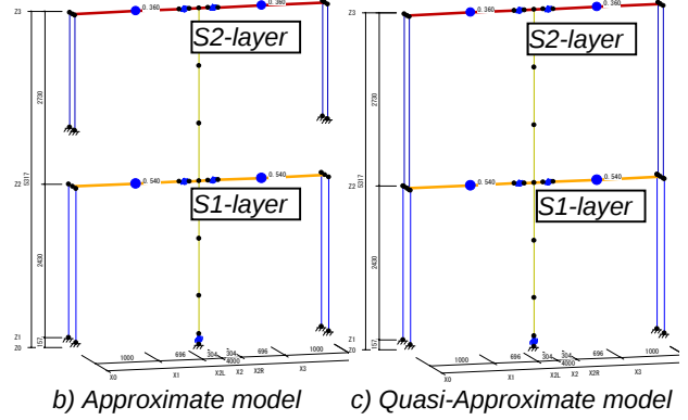
Figure 8 Three FEM response analyse models
