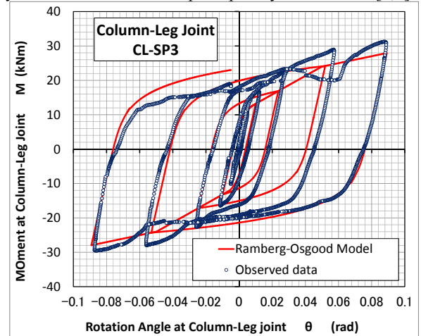
(a) Column-Leg Joint [6,7]
