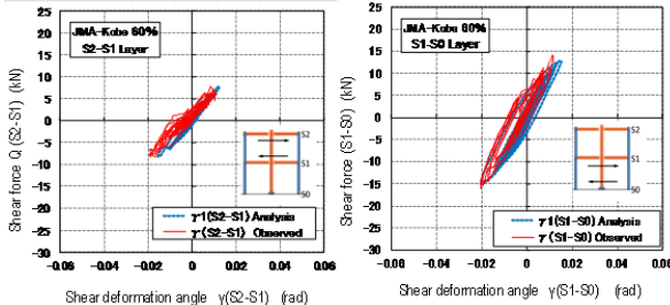
c) Force-shear deformation angle at 60% JMA-Kobe input. (blue: analysis red: observation)
