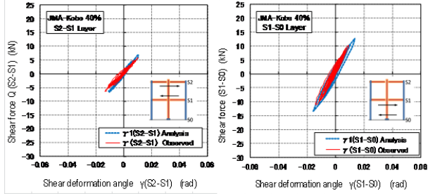
b) Force-shear deformation angle at 40% JMA-Kobe input.
