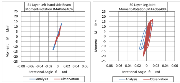
b) Moment-rotational angle at 40% JMA-Kobe input. (blue: analysis red: observation)
