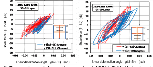
f) Force-shear deformation angle at 120% JMA-Kobe input.
