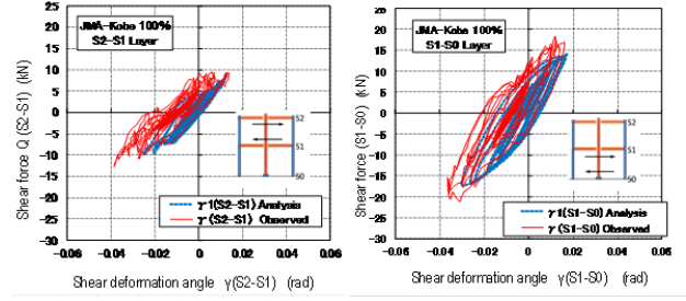
e) Force-shear deformation angle at 100% JMA-Kobe input.
