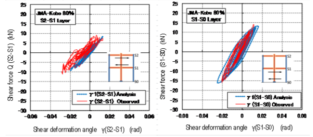
d) Force-shear deformation angle at 80% JMA-Kobe input.
