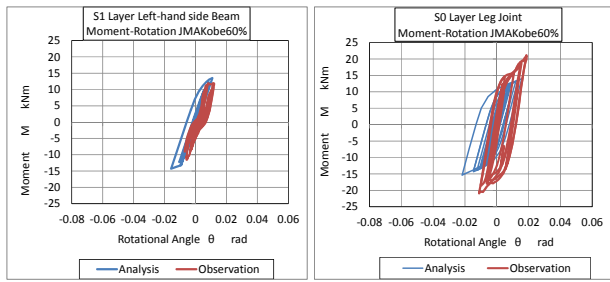
c) Moment-rotational angle at 60% JMA-Kobe input. (blue: analysis red: observation)
