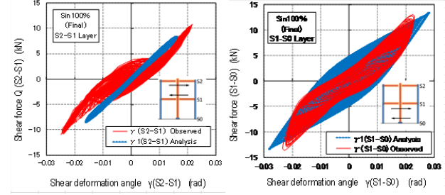
(blue: analysis red: observation) g) Force-shear deformation angle at 100% sin wave input.
