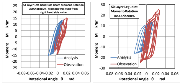
d) Moment-rotational angle at 80% JMA-Kobe input. (blue: analysis red: observation)
