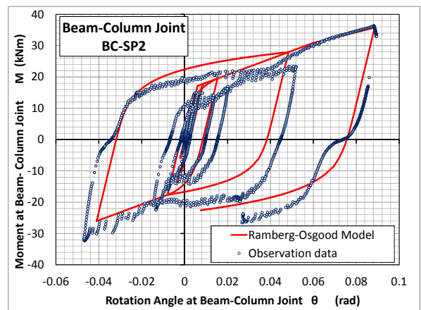
(b) Beam-Column Joint [6,7]
