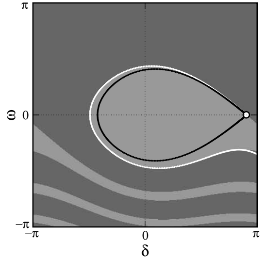
Fig. 4 Stability region, original separatrix and analytical criterion by the proposed method for the autonomous swing equation. The symbol \circ denotes the assumed saddle type equilibrium point.
