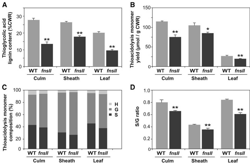
Figure 3. Chemical lignin analysis of cell walls from wild-type (WT) and FNSII -knockout mutant ( fnsl ) rice plants. A, Lignin content determined by thioglycolic acid assay. B to D, Lignin composition analysis by thioacidolysis. Shown are total monomer yield per CWR (B) and relative abundances (C and D) of H-, G-, and S-type trithioethylpropane monomers released from H-, G-, and S-type lignins. Values are means ± SD from individually analyzed plants ( n = 3), and asterisks indicate significant differences between wild-type and fnsl mutant plants (Student's t test: *, P < 0.05 and **, P < 0.01).
