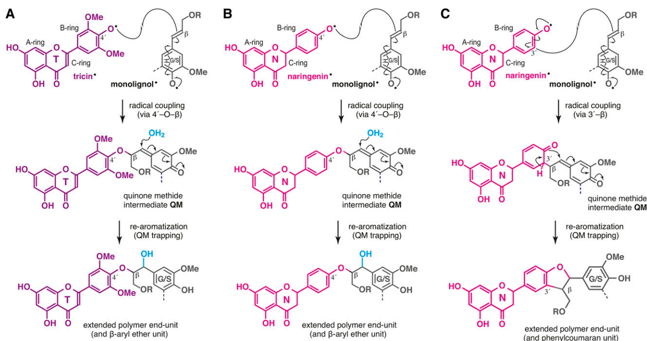
Figure 8. Generation of flavonoid-bound lignin units upon lignification. A. The 4'- O - \beta pathway for \beta -aryl units via cross-coupling of tricin and monolignols upon lignification in wild-type rice cell walls. B and C, The 4'- O - \beta (B) and 3'- \beta (C) pathways for \beta -aryl ether and phenylcoumaran units via cross-coupling of naringenin and monolignols upon lignification in fnsII mutant rice cell walls.
