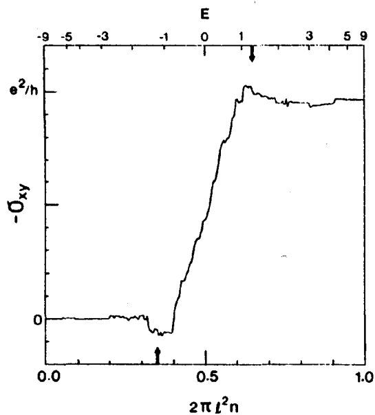
Figure 3. The Hall conductivity against the Landau-band filling. The arrows indicate the transition to extended behaviour for the finite sample size considered here.
