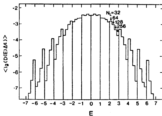
Figure 4. Logarithmic plot of the Thouless number. Within each energy bin, the system size is increased from N_t=32 to 256.
