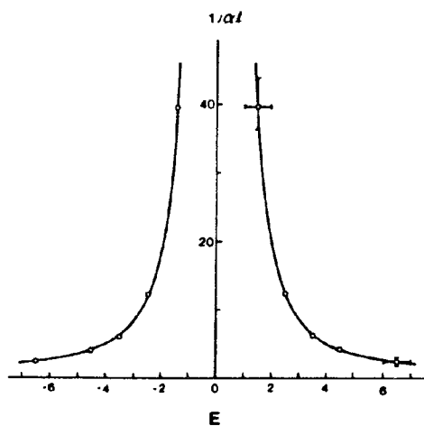
Figure 5. The quantity, 1/\alpha , with \langle D(E)\Delta\epsilon \rangle \sim \exp(-\alpha L) in figure 4 is plotted versus energy.
