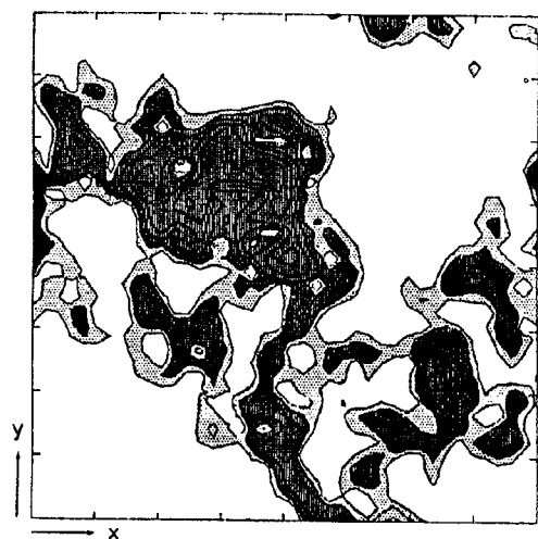
Figure 6. An eigenstate with energy \xi = E_0 - 0.007 is shown. The absolute value of the normalised wavefunction in the area of 40\frac{1}{2} \times 40\frac{1}{2} is shown with contour heights 0.1/2^{n/2} ( n=0, \dots, 5 ).
