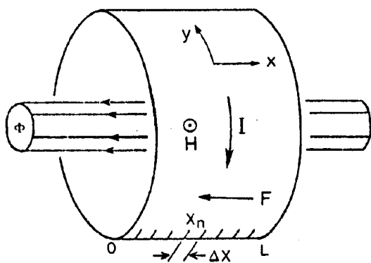
Figure 1. The Hall current I in the loop geometry with a magnetic field H , an electric field F and a magnetic flux \Phi through the cylinder. A discrete set of values is allowed for X .
