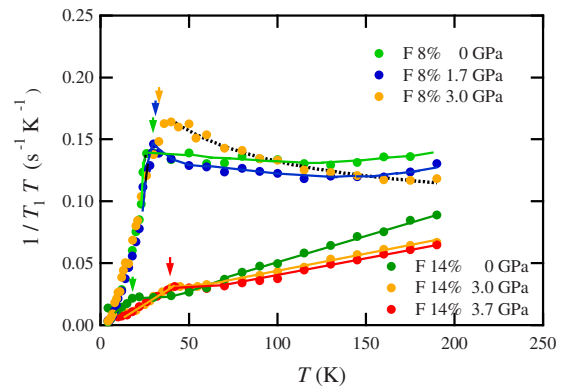
FIG. 4. (Color online) 1/T_1 T measured at several pressures. The dotted curve represents a Curie-Weiss curve. The other lines are guide to the eyes.
