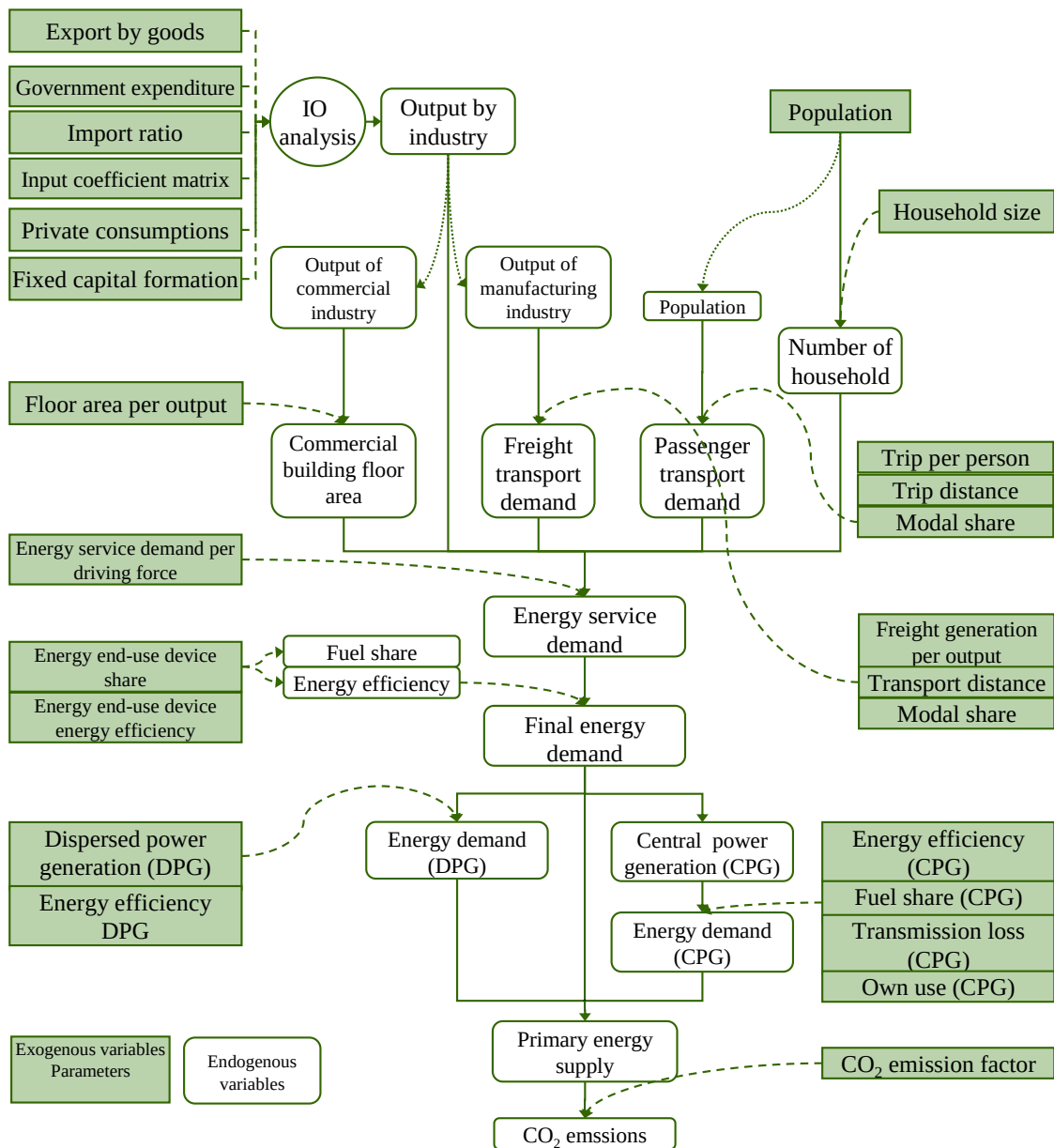
Fig. 3.4 Structure of ExSS
