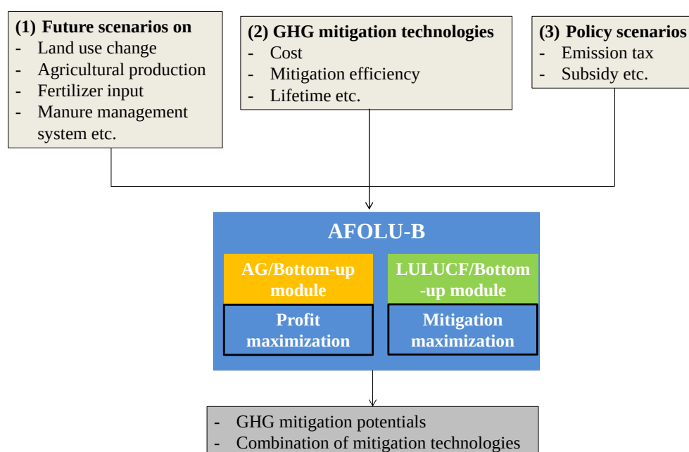
Fig. 3.7 Input and output of the AFOLUB model
