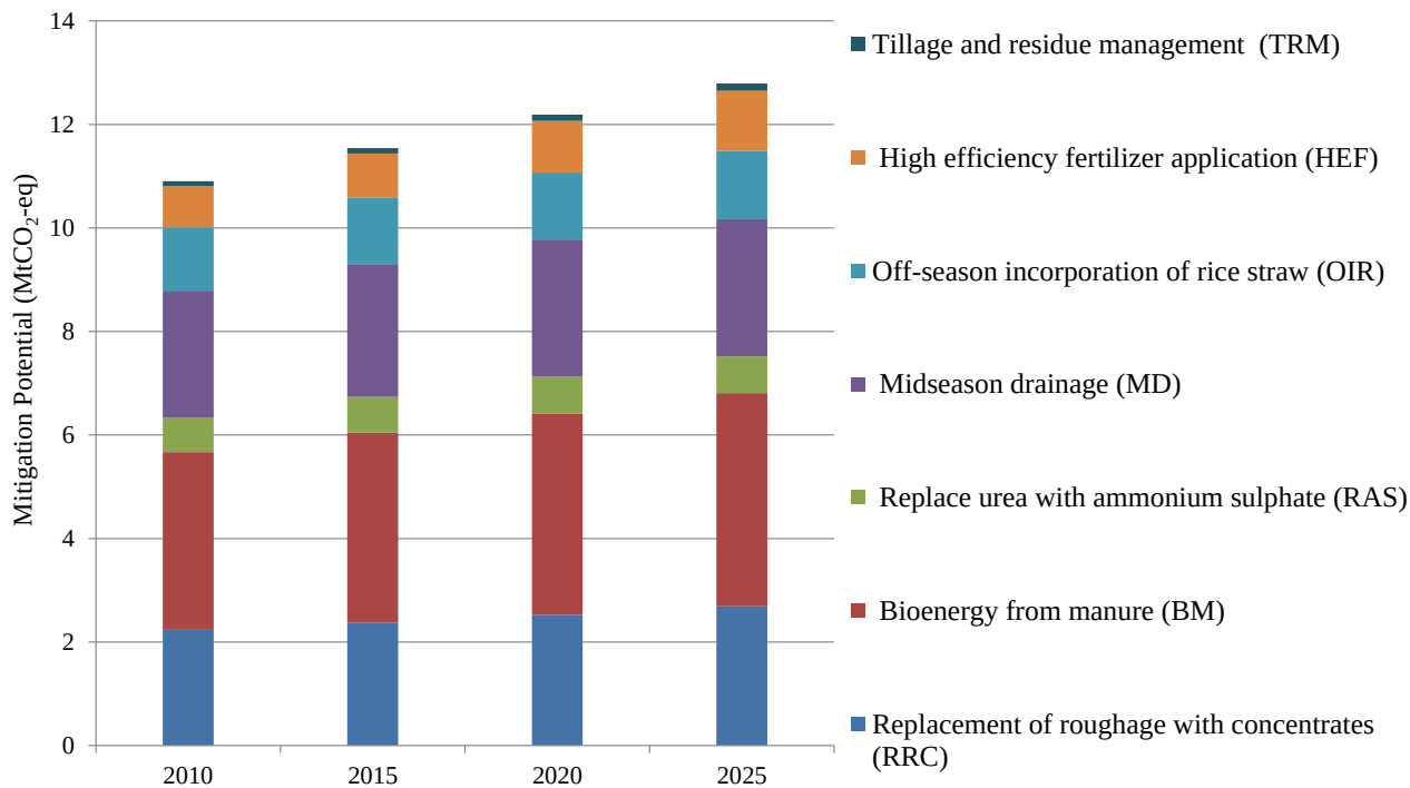
Fig. 7.15 Mitigation potential under 10 US$/tCO 2 -eq
