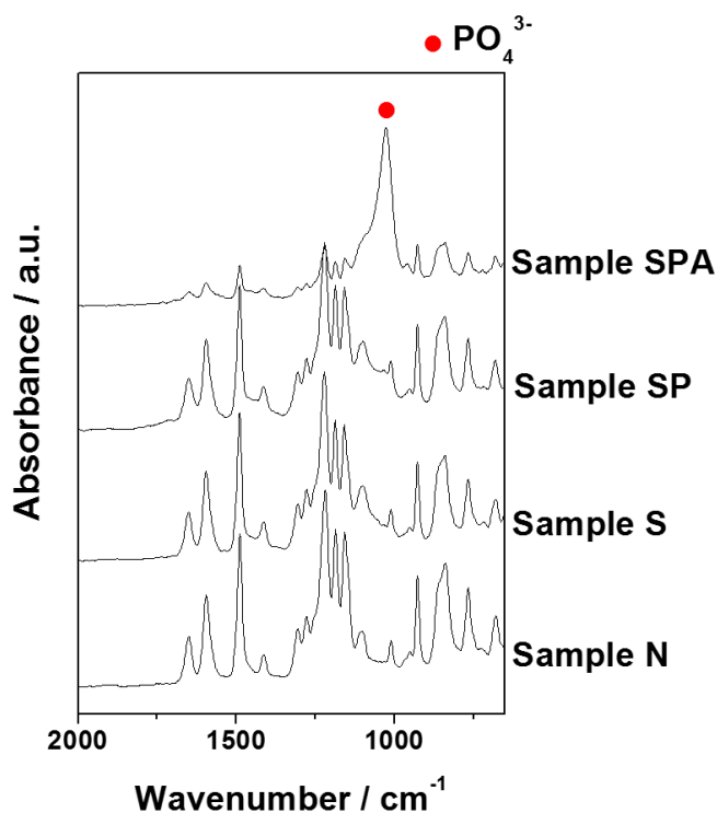
Fig.4 FT-IR spectra of the surface of Sample N, Sample S, Sample SP and Sample SPA.
