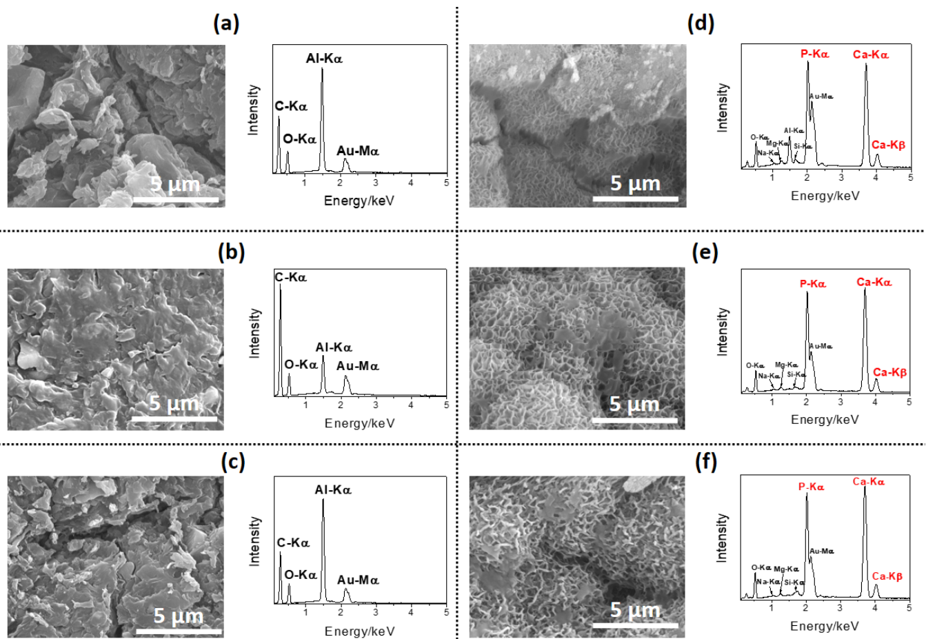
Fig.10 FE-SEM photographs and EDX spectra of (a) 44P, (b) 13P, (c) 44-13P, (d) 44PA after the immersion in SBF for 7 days, (e) 13PA after the immersion in SBF for 7 days, and (f) 44-13PA after the immersion in SBF for 7 days.
