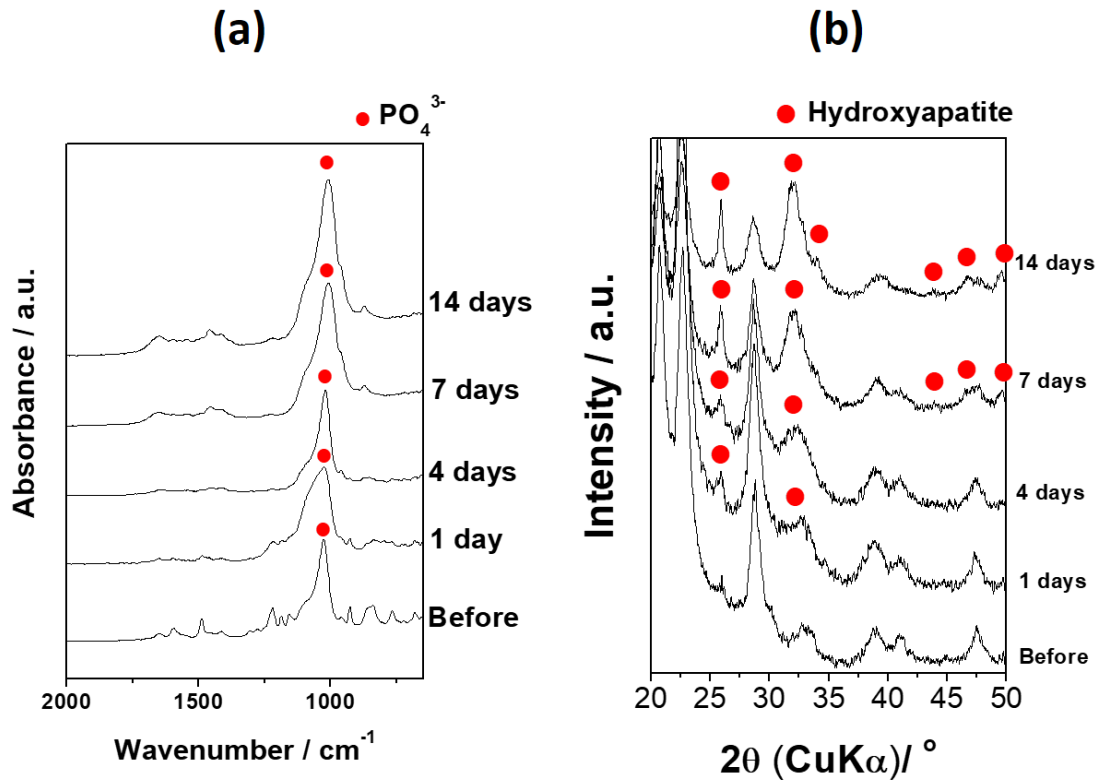
Fig.7 (a) FT-IR spectra and (b) TF-XRD patterns of the surface of Sample SPA before and after the immersion in SBF for 1 day, 4 days, 7 days and 14 days.
