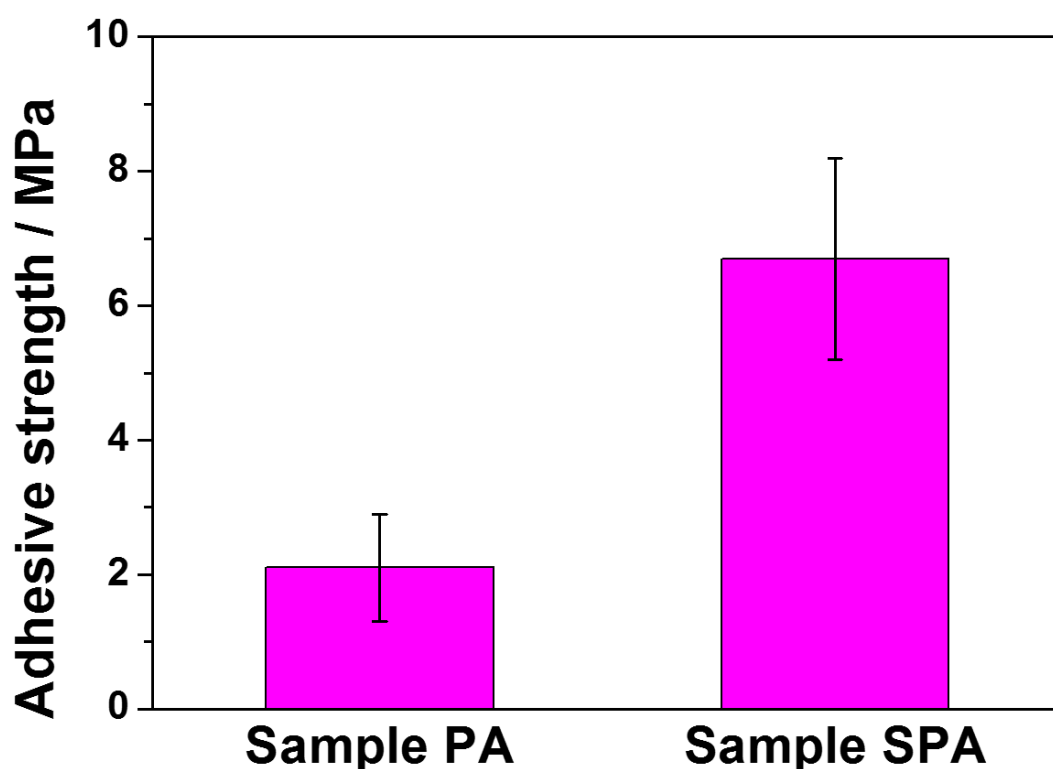
Fig.9 Average adhesive strength between PEEK substrate and hydroxyapatite layer formed on Sample PA and Sample SPA by immersion in SBF for 14 days.
