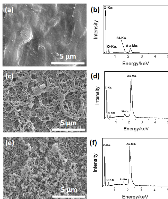
Fig.1 (a,c,e) FE-SEM photographs and (b,d,f) EDX spectra of the surface of (a,b) Sample N, (c,d) Sample S and (e,f) Sample SP.
