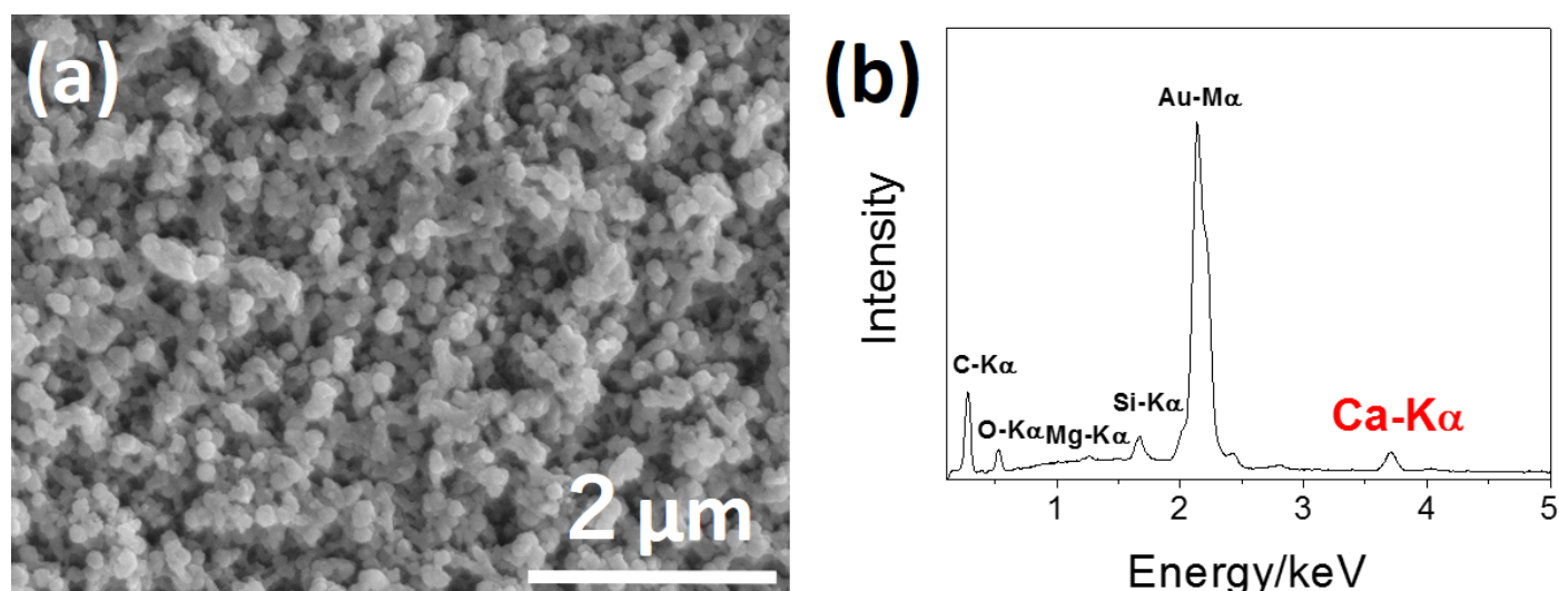
Fig. 5 (a) FE-SEM photograph and (b) EDX spectrum of the surface of Sample SPA.
