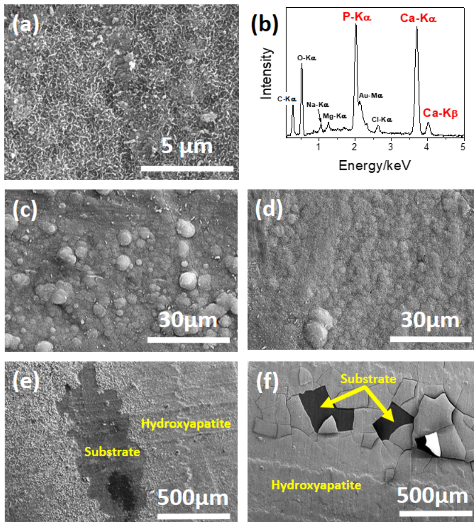
Fig.8 (a) FE-SEM photograph and (b) EDX spectrum of the surface of Sample SPA after the immersion in SBF for 1 day, and FE-SEM photographs after the immersion in SBF for 7 days for the surface of (c) Sample SPA, (d) Sample PA, (e) Sample SA and (f) Sample A.
