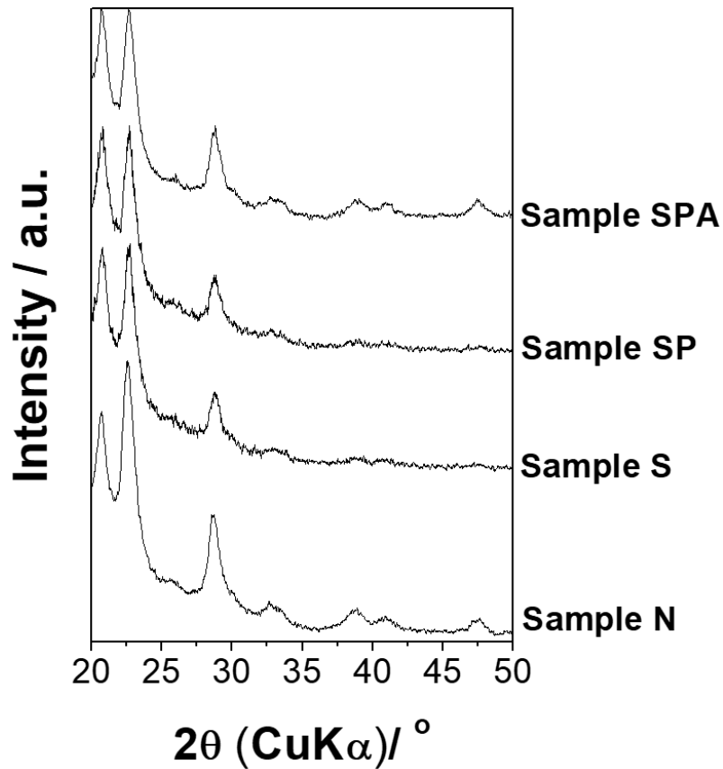
Fig.6 TF-XRD patterns of the surface of Sample N, Sample S, Sample SP and Sample SPA.
