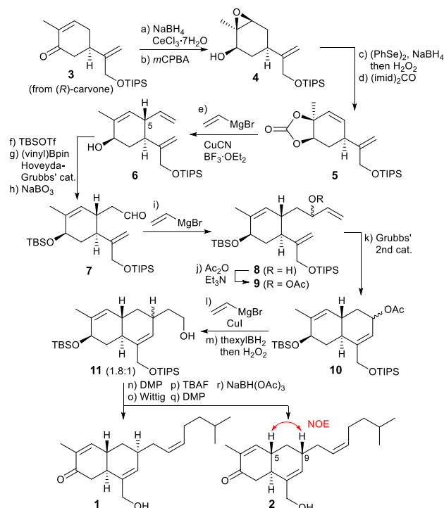
Scheme 1 Synthesis of 1 and 2 . Reagents and conditions: a) \text{NaBH}_4 , \text{CeCl}_3 \cdot 7\text{H}_2\text{O} , \text{MeOH} , -78^\circ\text{C} , quant., dr >19:1; b) m\text{CPBA} , \text{CH}_2\text{Cl}_2 , -20^\circ\text{C} , 90%, dr 21:1; c) (\text{PhSe})_2 , \text{NaBH}_4 , \text{EtOH} then \text{H}_2\text{O}_2 , \text{THF} , reflux; d) 1,1'-carbonyldiimidazole, \text{CH}_2\text{Cl}_2 , 46% (2 steps); e) (\text{vinyl})\text{MgBr} , \text{CuCN} , \text{BF}_3 \cdot \text{OEt}_2 , \text{THF} , -78^\circ\text{C} , 98%, dr >19:1; f) \text{TBSOTf} , 2,6-lutidine, \text{CH}_2\text{Cl}_2 , 94%; g) (\text{vinyl})\text{Bpin} , Hoveyda-Grubbs 2nd gen. cat., \text{CH}_2\text{Cl}_2 , reflux; h) \text{NaBO}_3 \cdot 4\text{H}_2\text{O} , \text{THF} , \text{H}_2\text{O} ; i) (\text{vinyl})\text{MgBr} , \text{THF} , 0^\circ\text{C} , 42% (3 steps), dr 1.3:1, 27% of starting material was recovered (BRSM 57%); j) \text{Ac}_2\text{O} , \text{Et}_3\text{N} , DMAP, \text{CH}_2\text{Cl}_2 , 98%; k) Grubbs' 2nd gen. cat., \text{CH}_2\text{Cl}_2 , reflux, 98%; l) (\text{vinyl})\text{MgBr} , \text{CuI} , \text{THF-Me}_2\text{S} (10:1), -30 to 0^\circ\text{C} ; m) \text{thexylborane} , \text{THF} , -20^\circ\text{C} , 30% (2 steps); n) Dess-Martin periodinane, pyridine, \text{CH}_2\text{Cl}_2 , 0^\circ\text{C} ; o) (4-methylpentyl)(triphenyl)phosphonium bromide, \text{NaHMDS} , \text{THF} , -78 to 15^\circ\text{C} ; p) \text{TBAF} , \text{THF} , 50^\circ\text{C} ; q) Dess-Martin periodinane, \text{NaHCO}_3 , \text{CH}_2\text{Cl}_2 , 40% (4 steps), E/Z >19:1; r) \text{NaBH}(\text{OAc})_3 , benzene-AcOH (10:1), 0^\circ\text{C} to r.t., 71%.
