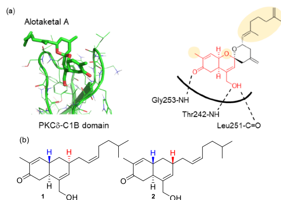
Figure 3 (a) Docking and molecular dynamics simulation of Alotaketol A with PKC \delta -C1B domain; (b) simplified compounds 1 and 2 .
