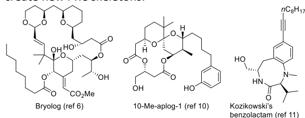
Figure 1. Isozyme-selective PKC ligands.
