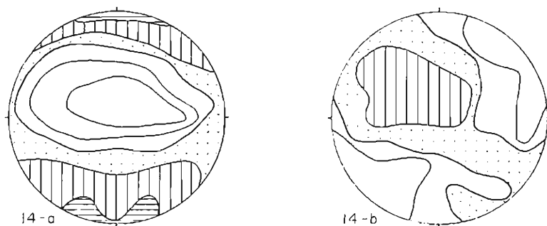
Fig. 30. Hindu-Kush, intermediate.
