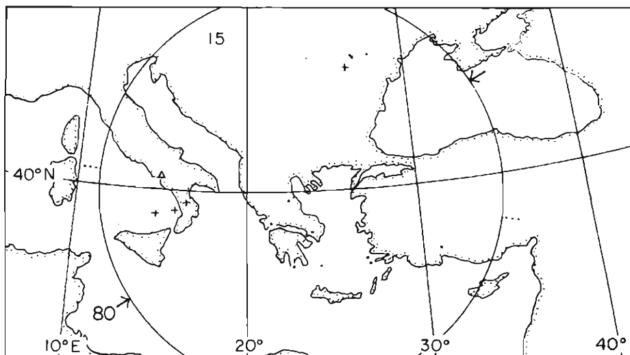
Fig. 34. Epicenter distribution and the results of the Italy-Greece-Turkey region.
