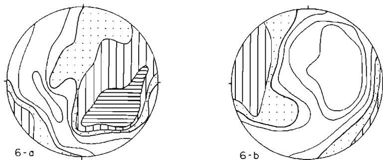
Fig. 16. (6-a): Alaska, intermediate, and (6-b): Aleutian Islands, intermediate.
