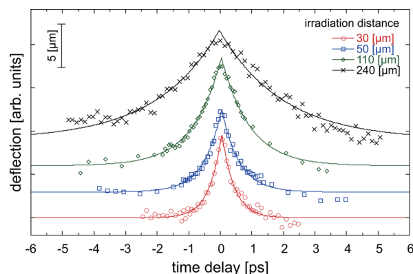
FIG. 3. (Color online) Electron pulse deflections as a function of time delay for laser spot distance of 30 \mu\text{m} (circle), 50 \mu\text{m} (square), 110 \mu\text{m} (diamond), and 240 \mu\text{m} (cross). The deflection is determined by the difference of the distance between the two electron source images from that between the laser spots. Each point is obtained by averaging the distances obtained from 30–50 laser shots. The solid lines are fitted to exponential functions to estimate the interaction times of the two electron pulses.
