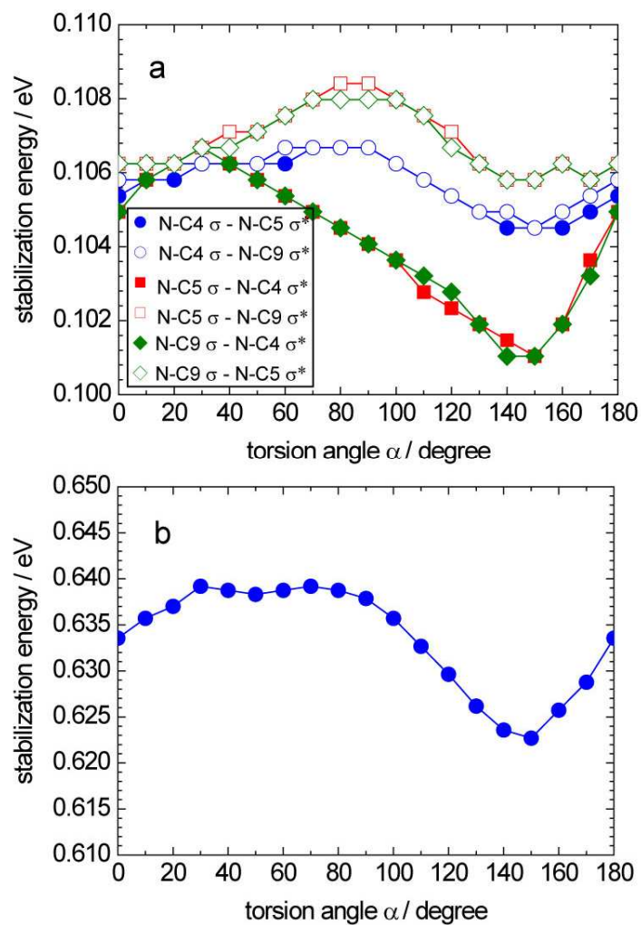
Fig. 3.11. Torsion angle \alpha dependence of the stabilization energy for the \sigma orbitals of the N-C4 ( \bullet , \circ ), N-C5 ( \blacksquare , \square ), and N-C9 ( \blacklozenge , \lozenge ) bonds by the interaction with the \sigma^* orbitals. The stabilization energy for each interaction is shown in (a) and the total stabilization energy is shown in (b). The calculations were performed at the level of HF/STO-3G.
