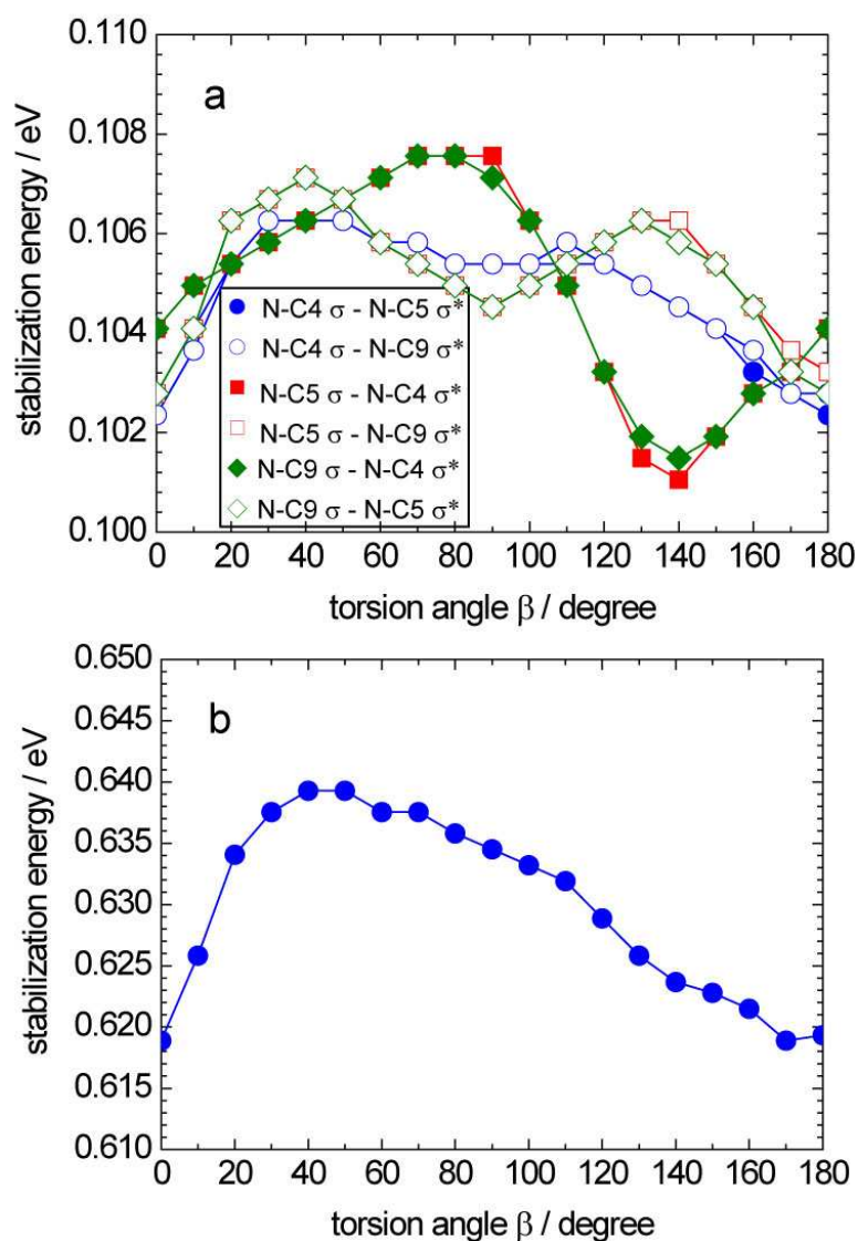
Fig. 3.17. Torsion angle \beta dependence of the stabilization energy for the \sigma orbitals of the N-C4 ( \bullet , \circ ), N-C5 ( \blacksquare , \square ), and N-C9 ( \blacklozenge , \lozenge ) bonds by the interaction with the \sigma^* orbitals. The stabilization energy for each interaction is shown in (a) and the total stabilization energy is shown in (b). The calculations were performed at the level of HF/STO-3G.
