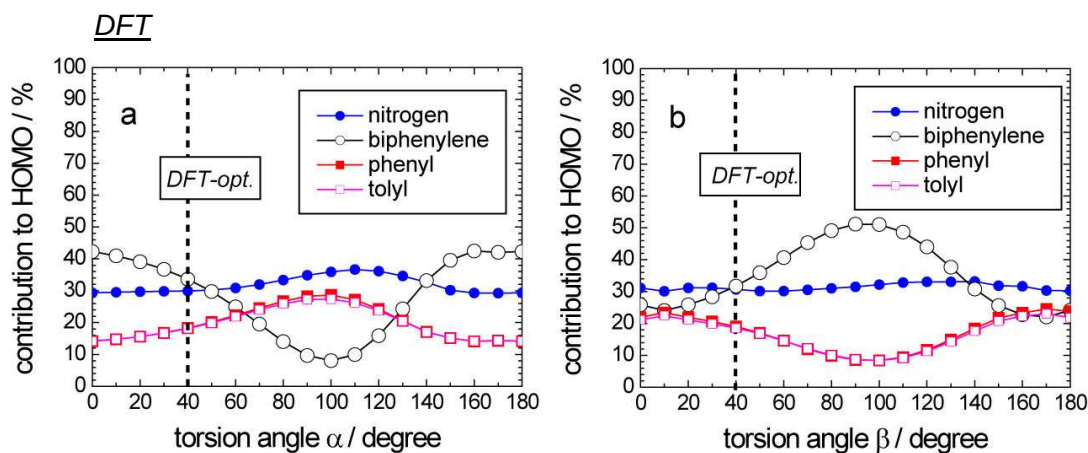
Fig. 3.19. Torsion angles, (a) \alpha and (b) \beta , dependences of HOMO of TPD, expressed by the summation of the squares of the MO coefficients in percentage for respective molecular moieties, nitrogen ( \bullet ), biphenylene ( \circ ), phenyl ( \blacksquare ), and tolyl ( \square ). The \beta and \gamma values are assumed to be equal and all the other structural parameters are fixed to the optimized values. The calculations were performed by B3LYP/6-31G(d) method.
