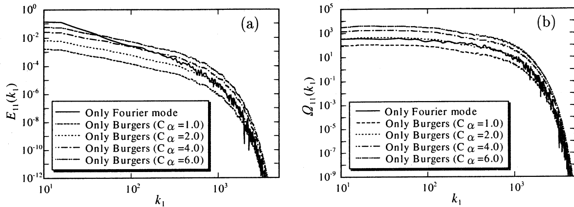
Figure 2: The effect of the parameter \alpha of the Burgers vortex on the 1-D wavenumber energy and enstrophy spectrum. (a) Change of 1-D energy spectrum. (b) Change of 1-D enstrophy spectrum.
