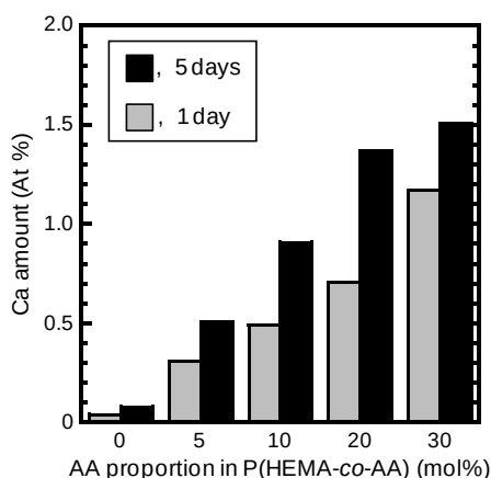
Fig. 3. Ca amount (in At %) incorporated in the films of m -9CNC/PHEMA nd and m -9CNC/P(HEMA y -co-AA (100- y ) ) nd ( n = 1, 5 ), plotted as a function of the AA proportion (100- y ) in the vinyl polymer.
