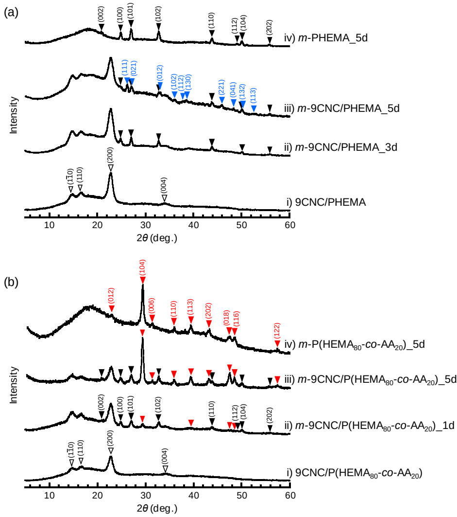
Fig. 4. WAXD intensity profiles for mineralized films of (a) 9CNC/PHEMA series and (b) 9CNC/P(HEMA 80 -co-AA 20 ) series. Black, blue, and red arrows indicate a diffraction coming from vaterite, aragonite, and calcite crystals, respectively. In data of nonmineralized CNC/polymer films (data a-i and b-i), major diffraction peaks from cellulose I \beta are marked by white arrows.
