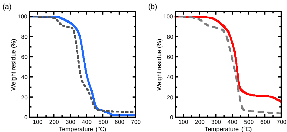
Fig. 6. TGA data obtained for various film specimens: (a) 9CNC/PHEMA (dotted line in black) and m -9CNC/PHEMA_5d (solid line in blue); (b) 9CNC/P(HEMA 90 -co-AA 10 ) (dashed line in gray) and m -9CNC/P(HEMA 90 -co-AA 10 )_5d (solid line in red).
