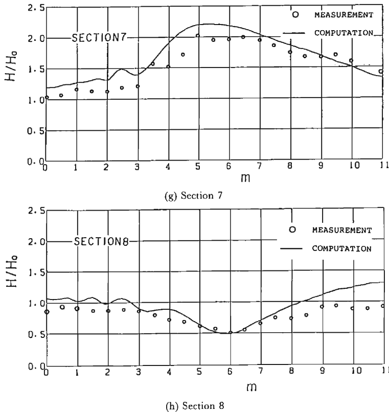
Fig. 11. Comparison of wave height distributions between calculations and experiments by the Delft Hydraulics Laboratory 15) .
