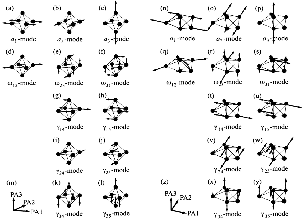
Figure 1: The twelve hyperspherical modes of the six-atom cluster, M_6 , around the OCT ((a)-(l)) and the CTBP isomers ((n)-(y)). The cluster is aligned so that the first, second, and third principal axes (PA1, PA2, and PA3 respectively) are parallel to the axes indicated in (m) for OCT and in (z) for CTBP. (The OCT isomer shown here is slightly deformed from the potential energy minimum.)
