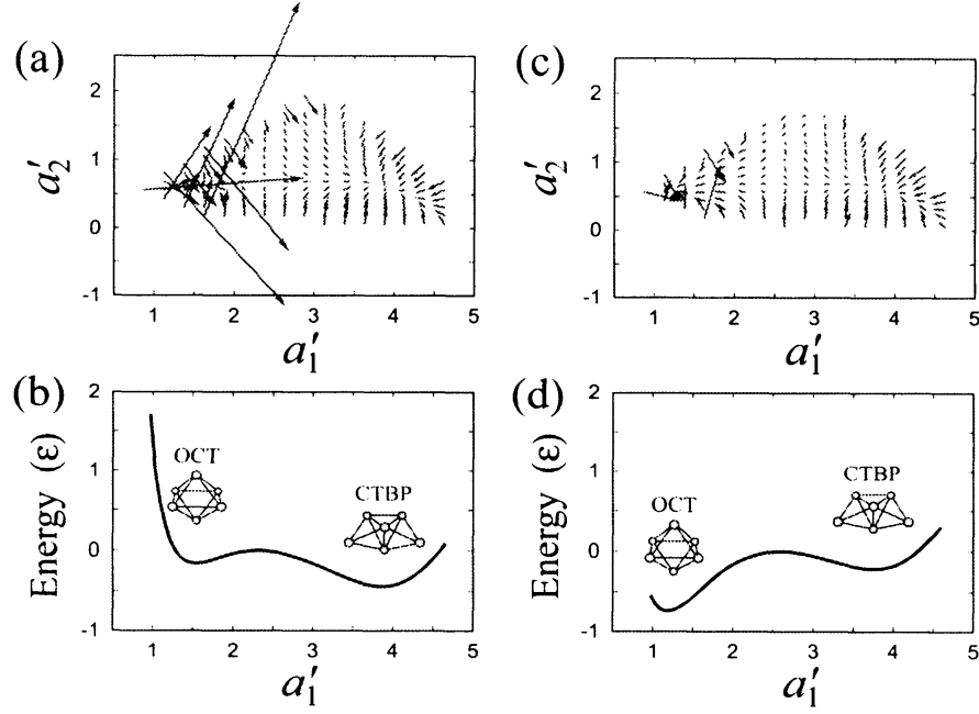
Figure 2: (a) Averaged force field in the space of the reaction coordinate a'_1 and a “bath” mode a'_2 when the three twisting modes are highly active . (b) Line integral (mean force potential) of the average force field in (a) along the reaction coordinate a'_1 . (c) Average force field in the space of the reaction coordinate a'_1 and a'_2 when the three twisting modes are highly inactive . (d) Line integral (mean force potential) of the average force field in (c) along the reaction coordinate a'_1 .
