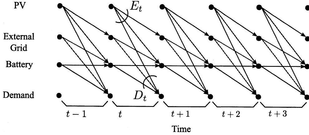
Figure 2: Time-Space Network Model for the Electric Power Network
