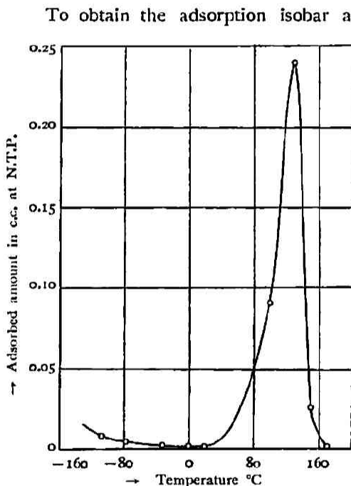
Fig. 8.— Adsorption isobar of methane at 0.01 c.c. for Ni(I).
