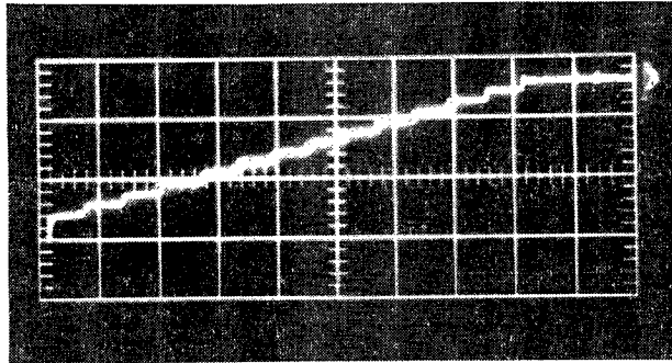
(a) Granular TNT, sweep velocity 100 \mu\text{s}/\text{div} .
