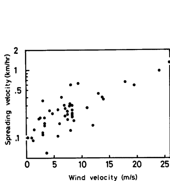
Fig. 4 Fire spreading velocity for urban area against wind velocity 9)
