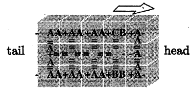
Figure 10: A simple Worm in SR_9 .
