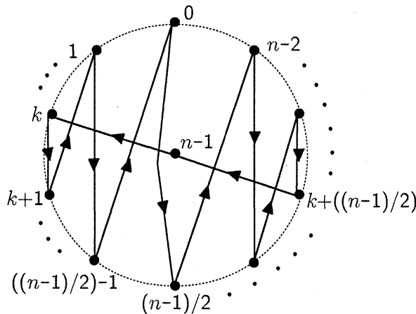
Figure 1: Structure of Hamiltonian path H_k .
