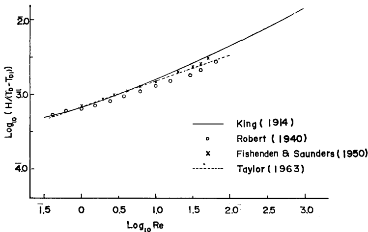
Fig. 1. Heat transfer rate ( \text{watt cm}^{-1} \text{ } ^\circ\text{C}^{-1} ) from fine wire as a function of Reynolds number.
