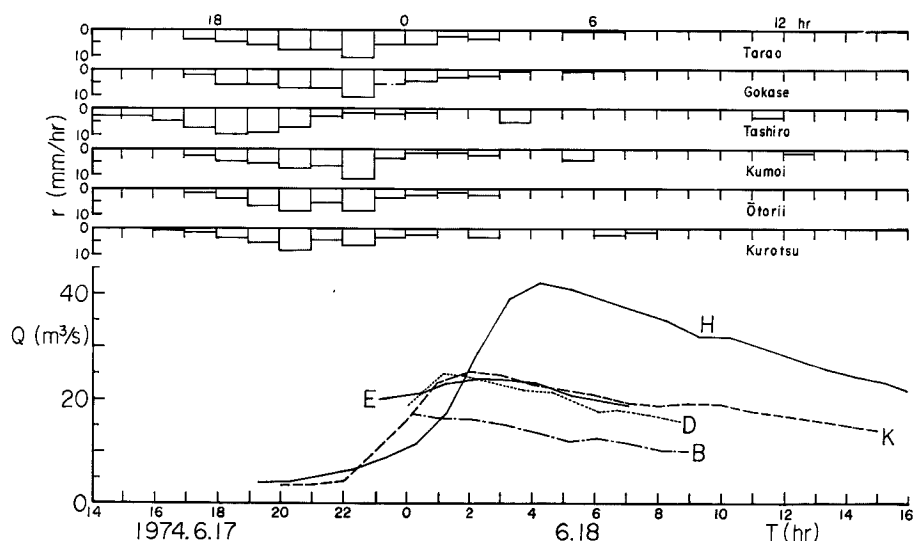
Fig. 3 Hydrographs observed at several stations along the main channel.
