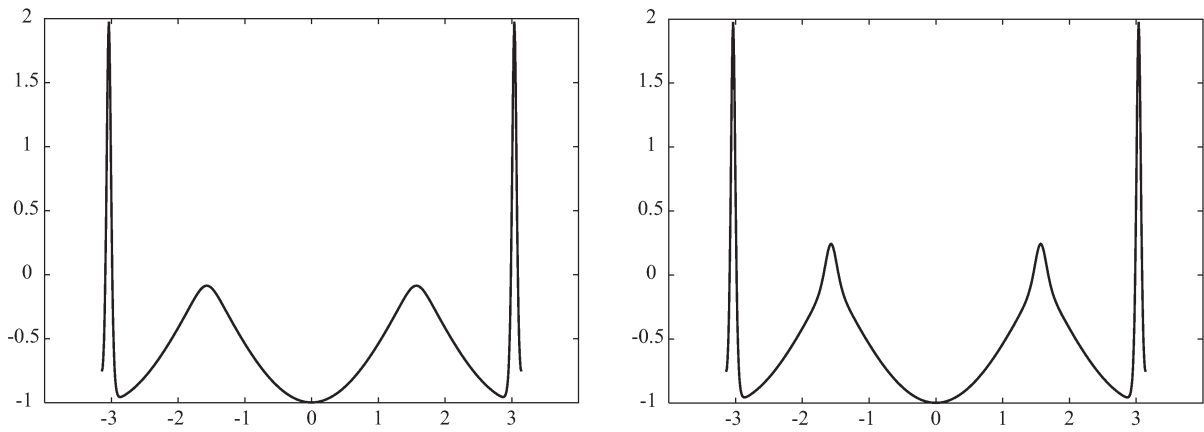
Figure 10. Two solutions at R = 1000 , on the branch separated from the trivial solutions. \ell = 1 .
