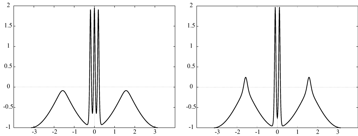
Figure 8. Two solutions at R = 1000 , bifurcating from the third bifurcation point. \ell = 1 .
