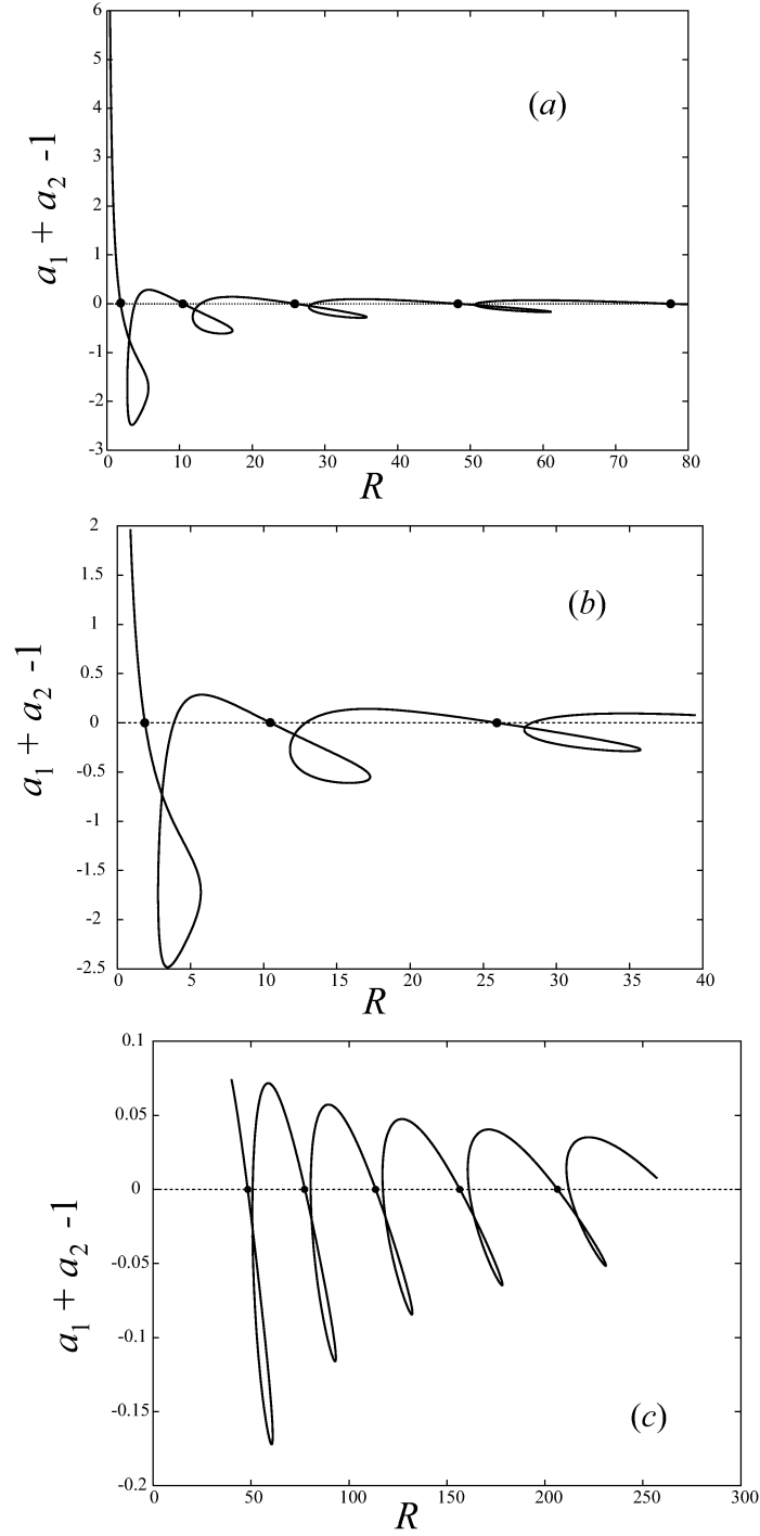
Figure 15. Bifurcation diagrams. \ell = 1 . (a) 0 < R < 80 . (b) 0 < R < 40 . (c) 40 < R < 250 . Intersections with the horizontal axis marked by a small disk are bifurcation points. Those intersections without a mark are not a bifurcation point: They simply occur because of the projection onto the (a_1 + a_2 - 1, R) plane.
