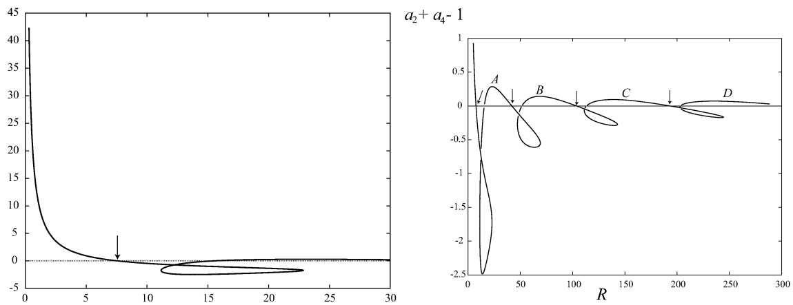
Figure 22. Diagrams. Points indicated by the arrows are bifurcation points. Other intersections are artificial, caused by the projection onto (R, a_2 + a_4 - 1) -plane.
