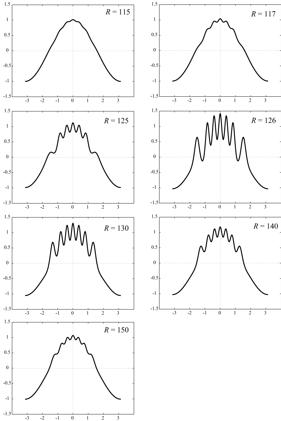
Figure 20. Profiles of bifurcating solutions. \ell = 1 . 115 < R < 160 .
