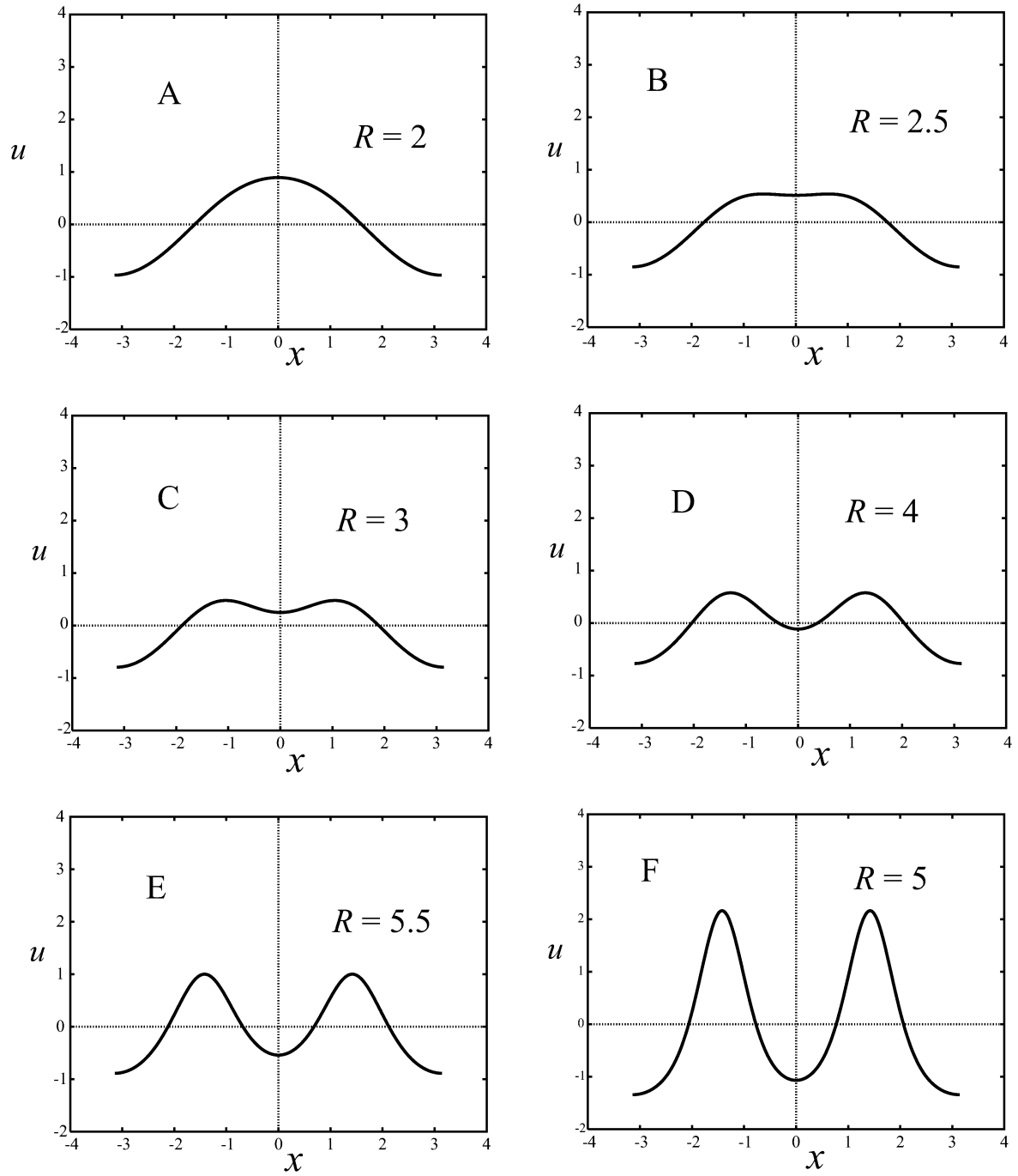
Figure 17. Profiles of bifurcating solutions. \ell = 1 . (a) 2 < R < 10 .
