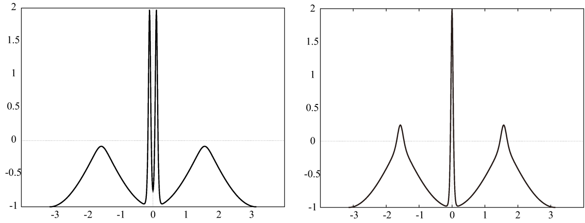
Figure 7. Two solutions at R = 1000 , bifurcating from the second bifurcation point. \ell = 1 .
