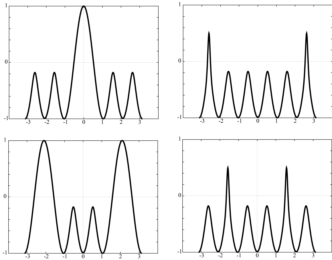
Figure 14. Graphs of u of (3.1) at R = 1000 . \ell = 3 .
