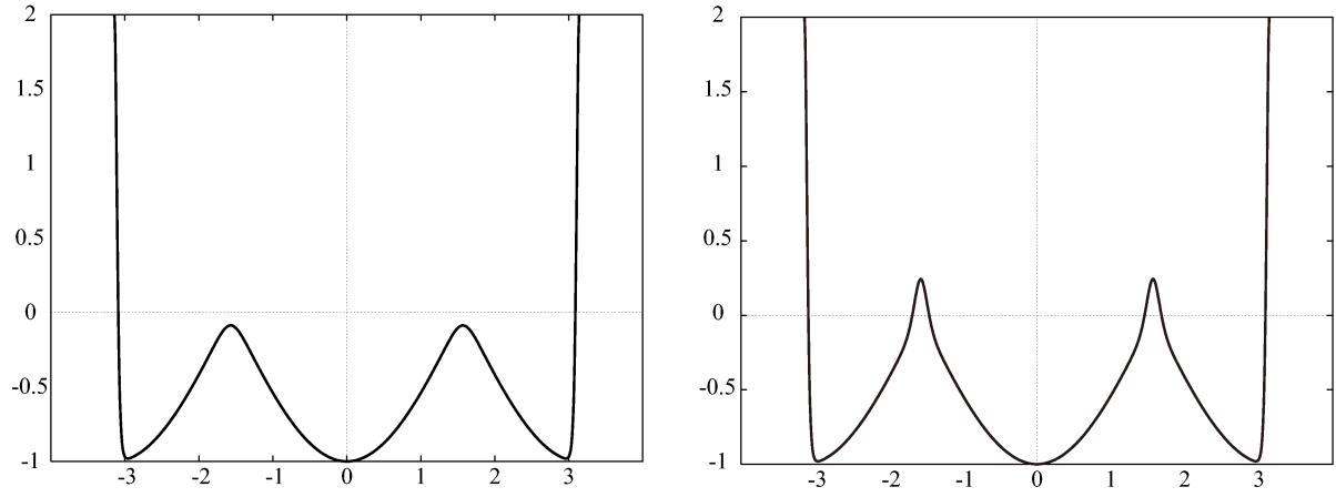
Figure 9. Two solutions at R = 1000 , on the branch separated from the trivial solutions. \ell = 1 .
