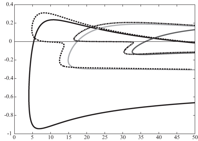
Figure 6. Bifurcation diagram. \ell = 1 . Solid lines represent branches which bifurcate from the trivial solutions. Broken lines represent those branches which are separated from the trivial solutions.
