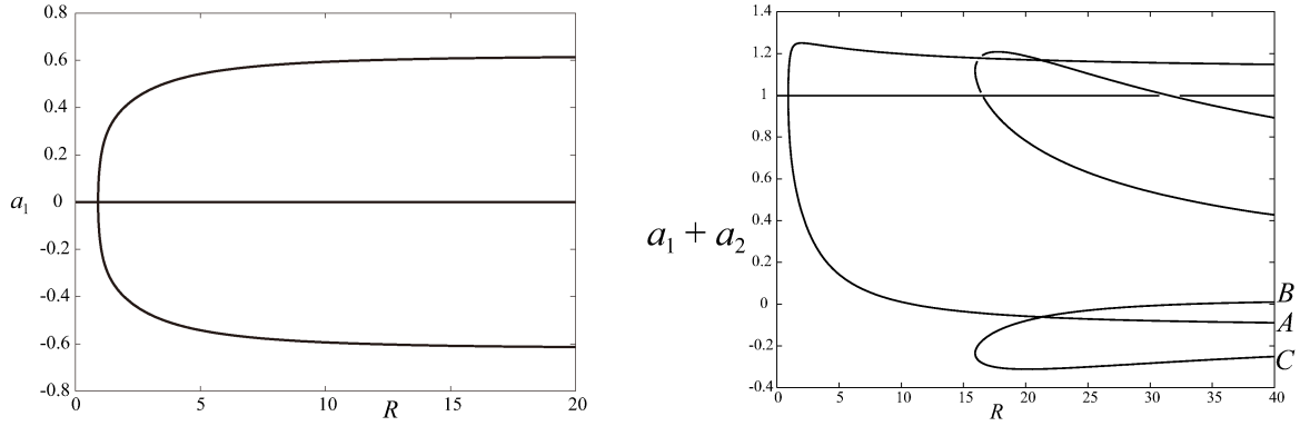
Figure 11. (left) Bifurcation diagram of (3.1) in (R, a_1) . \ell = 2 . This diagram is taken from [6]. (right) the diagram in (R, a_1 + a_2) . Secondary branches are added.
