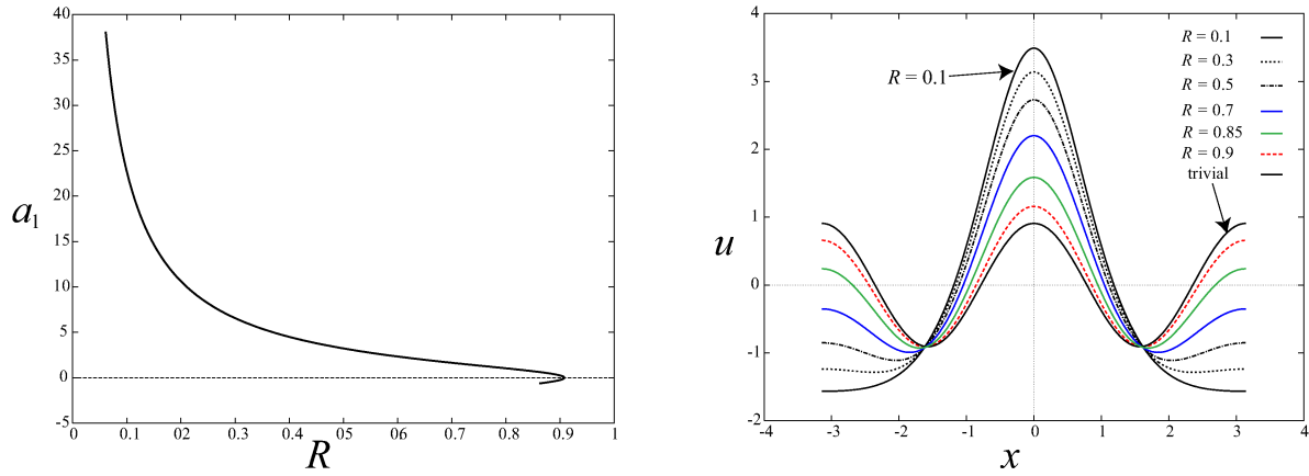
Figure 21. (left): Bifurcation diagrams. (right): Graphs of u for 0.1 \leq R \leq 0.908 .
