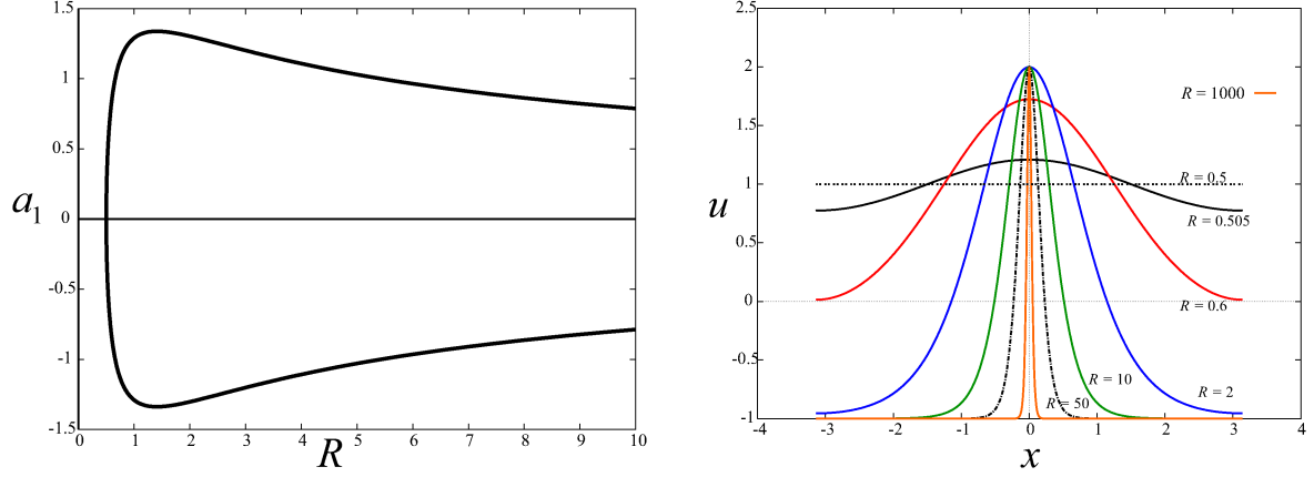
Figure 1. \ell = 0 . (left) Bifurcation diagram, where the Fourier coefficient a_1 is plotted against R . A pitchfork bifurcates at R = 1/2 . (right) Profiles of the bifurcating solutions: \ell = 0, R = 0.505, 0.6, 2, 10, 50 , and R = 1000 .
