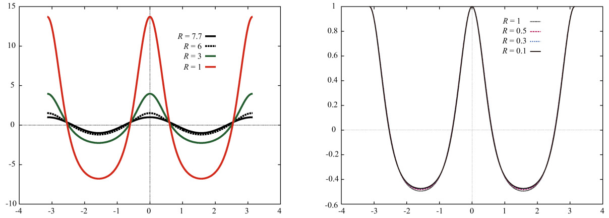
Figure 23. Solutions of mode two with smaller R .
