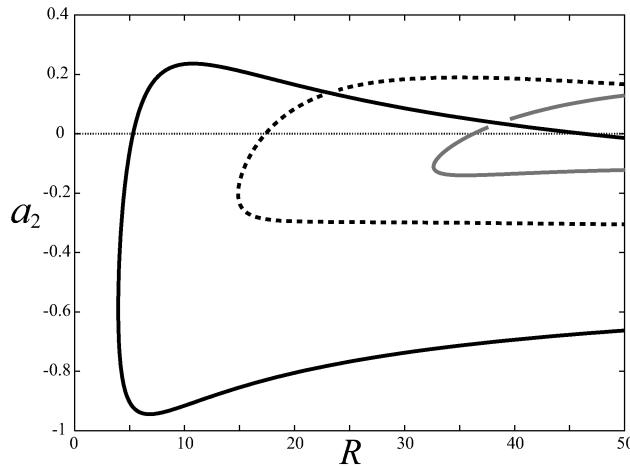
Figure 2. Bifurcation diagram. \ell = 1 .
