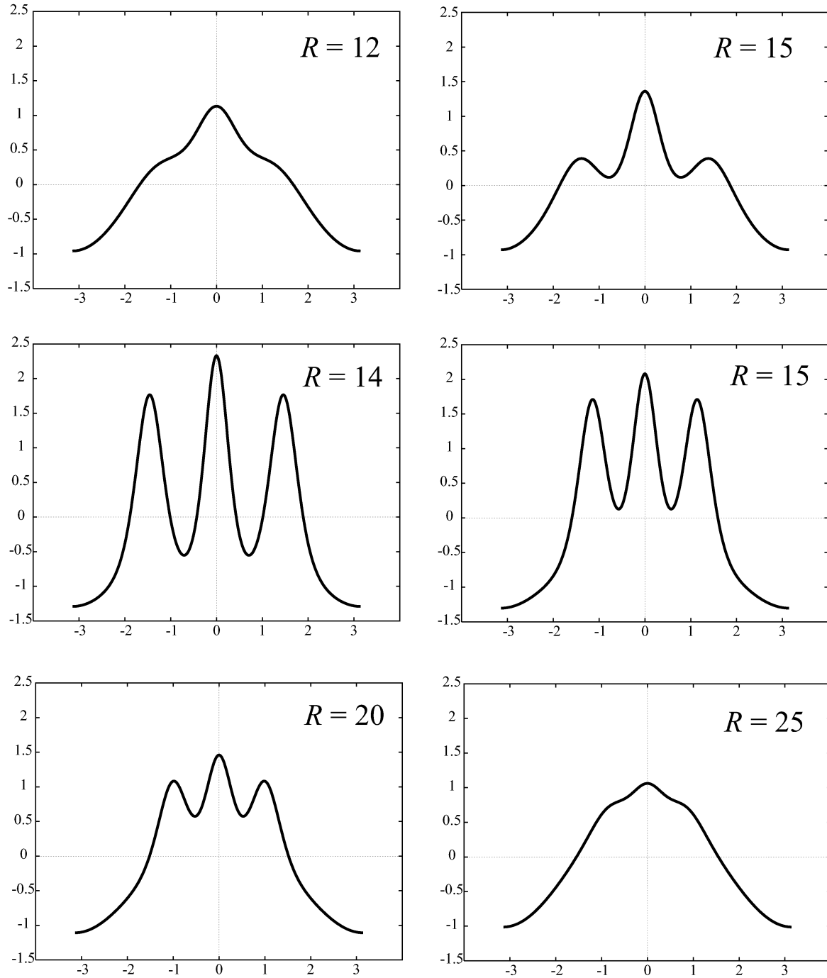
Figure 19. Profiles of bifurcating solutions. \ell = 1 . 12 < R < 25 .
