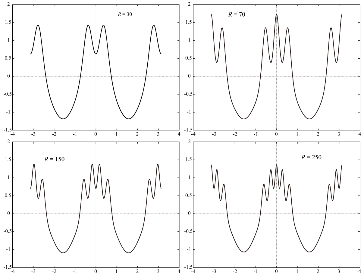
Figure 24. Solutions A, B, C , and D in Figure 22 (right).
