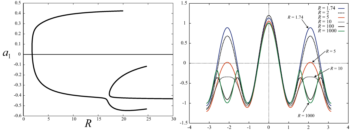
Figure 13. (left) Bifurcation diagram of (3.1) in (R, a_1) . \ell = 3 . (right) Graphs of u in the upper part of the branch.
