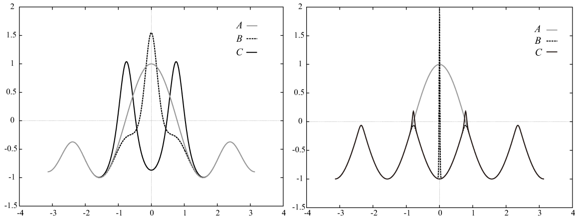
Figure 12. (left) Graphs of the bifurcating solutions u of (3.1) at R = 40 . (right) Graphs at R = 10000 . A, B , and C correspond to those marked in Figure 11.
