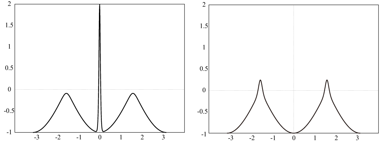
Figure 5. Two solutions at R = 1000 , bifurcating from the primary bifurcation point. \ell = 1 .
