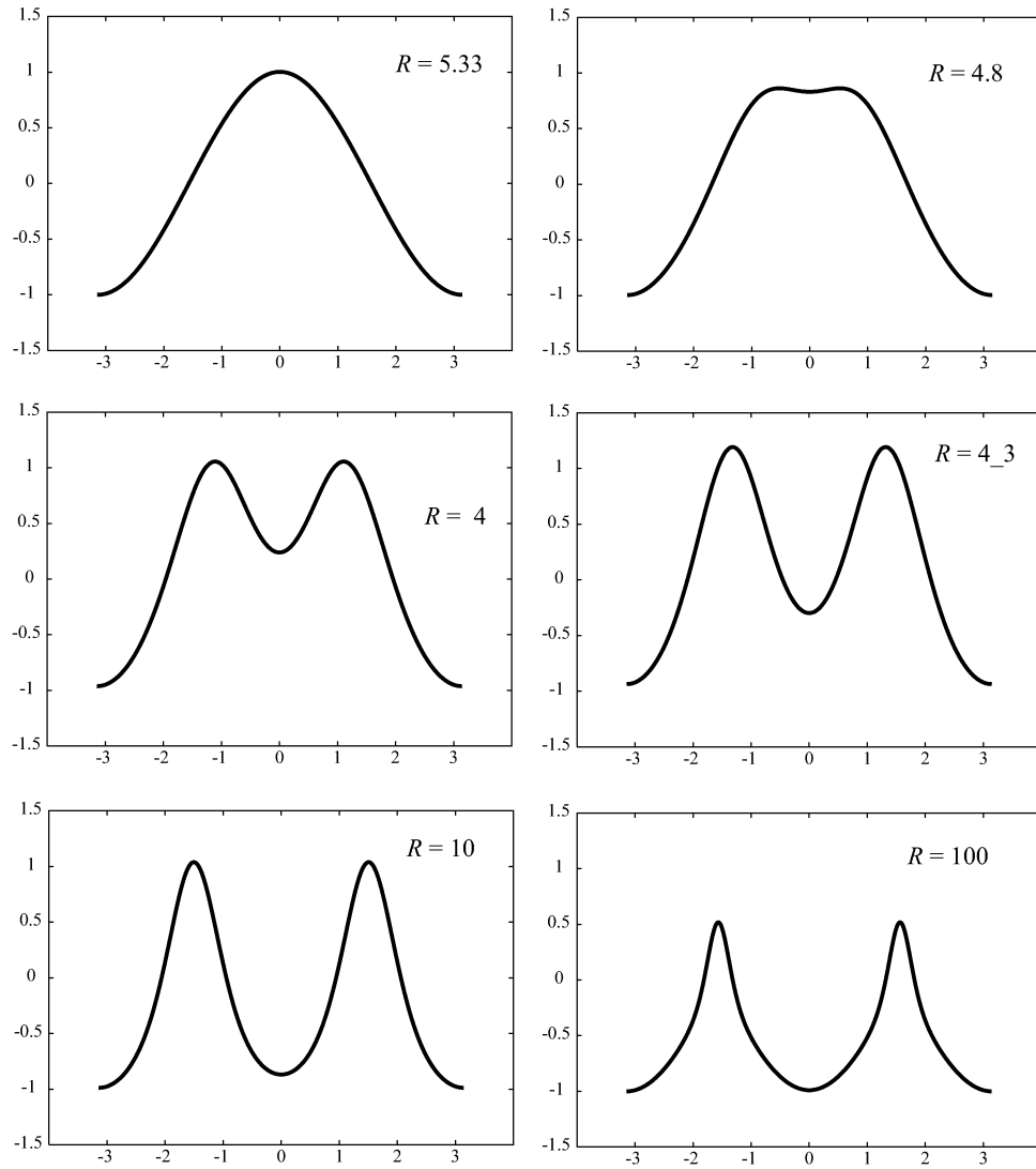
Figure 4. Graphs of solutions on the lower part of the leftmost bifurcating branch in Figure 2. \ell = 1 .
