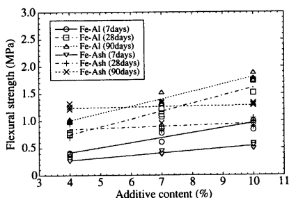
Fig. 5 Flexural strength versus additive content
