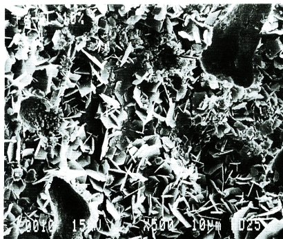
Photo 4 SEM of soil stabilized with 10% of Fe-Al Lime after 28 days
