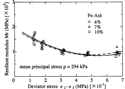
Fig. 17 Resilient modulus versus deviator stress
