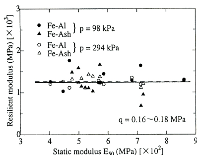
Fig. 23 Resilient modulus versus static modulus E_{s0}
