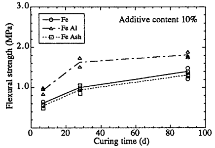
Fig. 8 Flexural strength versus curing time
