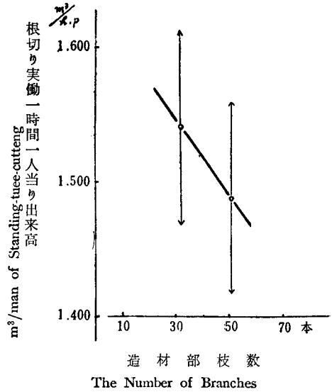
Fig. 2 The Effect of the Number of Branches of m^3/\text{man hour} of Standing-tree-cutting
