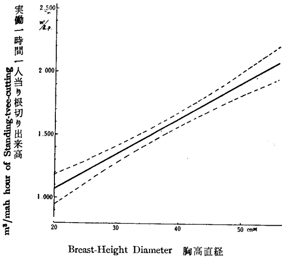
Fig. 1 The Effect of B. H. D on m^3/\text{man hour} of Standing-tree-cutting
