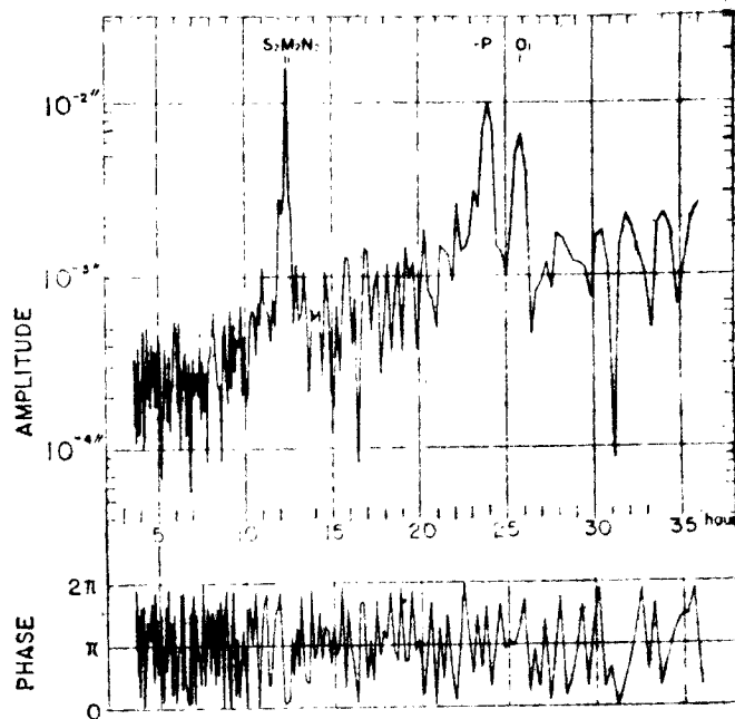
Fig. 11. Amplitude and phase spectra of the E-W component tilt ( Aa ) at Akibasan.
