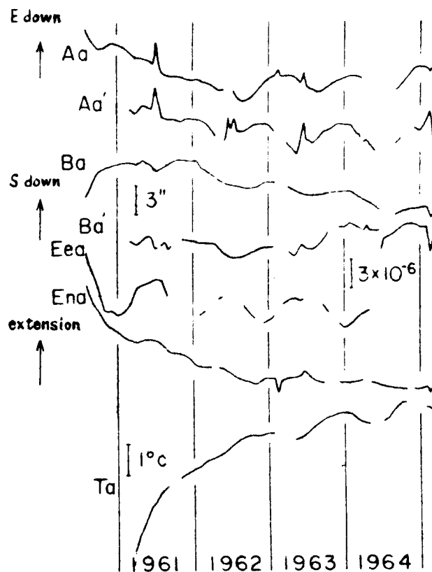
Fig. 5. Secular changes of the ground tilts and strains at Akibasan.
