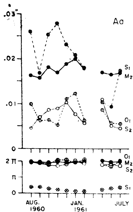
Fig. 9e. Amplitudes and phases of the E-W component tilt at Aki-basan.
