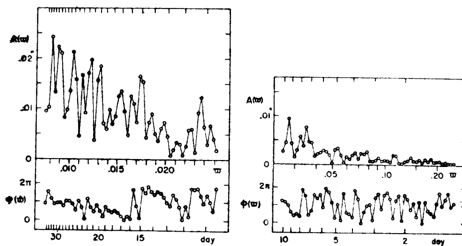
Fig. 21. Corrected amplitude and phase spectra of the N-S component tilt at Akibasan.
