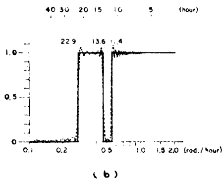
Fig. 27. Comparison of responses of designed ( solid line ) and digital filters ( dashed line ).
