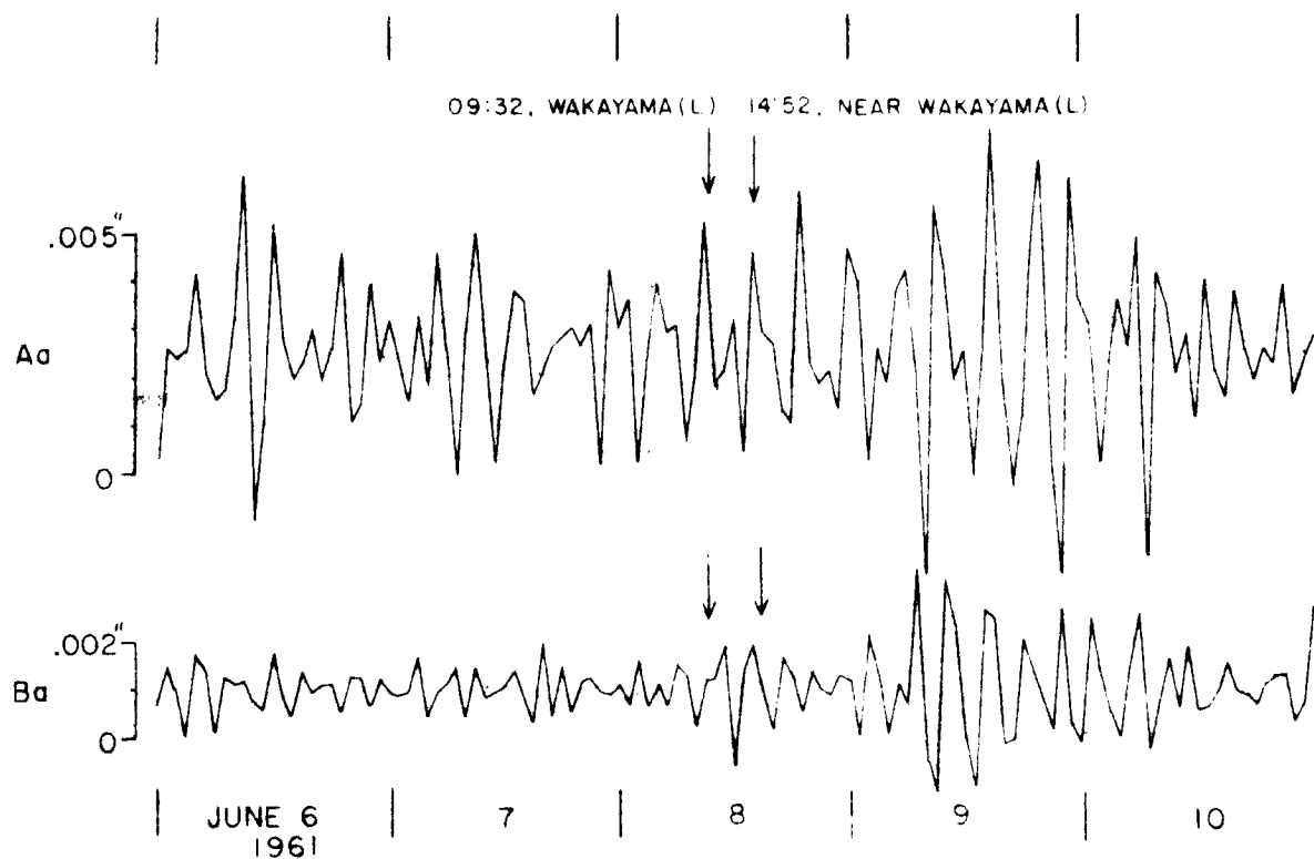
Fig. 36. Examples of filtered tiltgrams before and after the local earthquakes at 09h32m and 14h52m on June 8, 1961.
