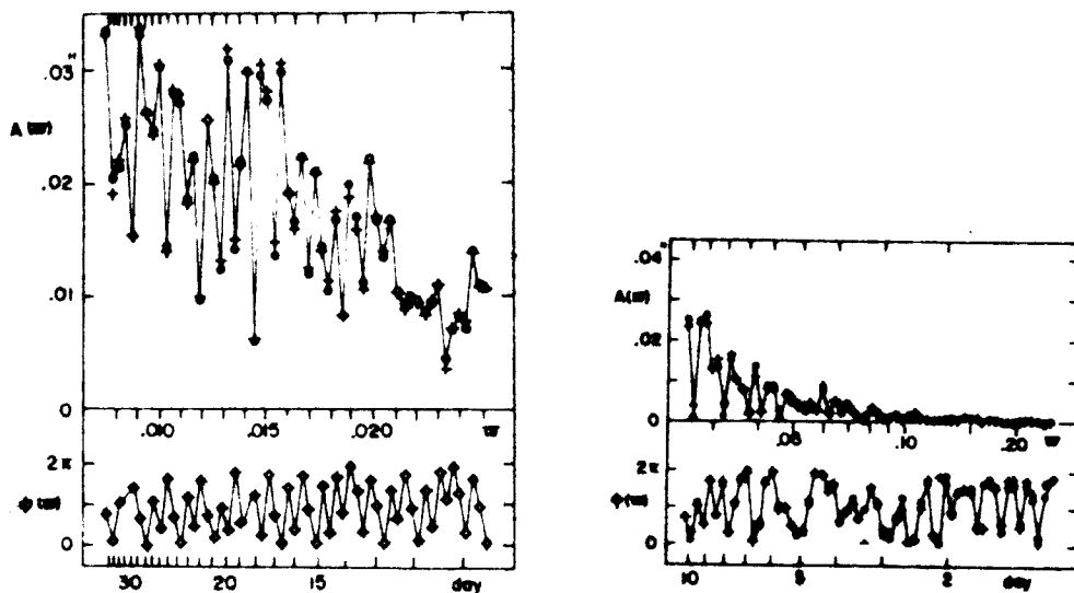
Fig. 13. Spectral amplitude A(\omega) and phase \phi(\omega) of the E-W component tilt at Akibasan. The cross represents the corrected values for the oceanic tides, air temperature, atmospheric pressure and its time derivative.
