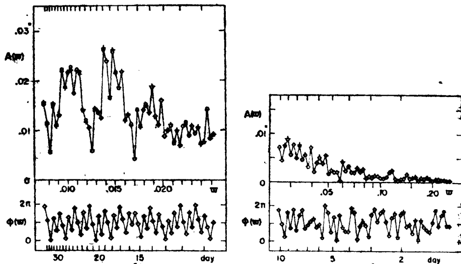
Fig. 14. Spectral amplitude and phase of the N-S component tilt at Akibasan. The cross represents the corrected values for the oceanic tides, air temperature, atmospheric pressure and its time derivative.
