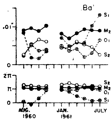
Fig. 9g. Amplitudes and phases of the N-S component tilt at Aki-basan.
