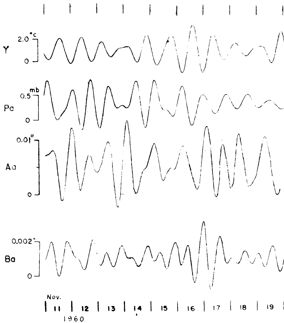
Fig. 31. Filtered records by 0.0770-0.0430 c/h band-pass filter.
