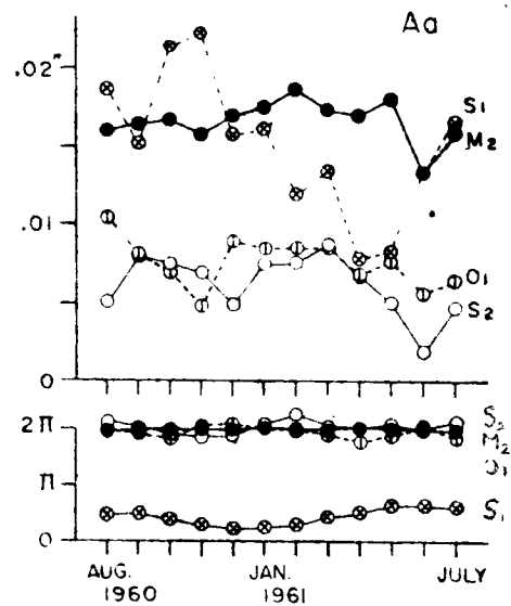
Fig. 9d. Amplitudes and phases of the E-W component tilt at Akibasan.
