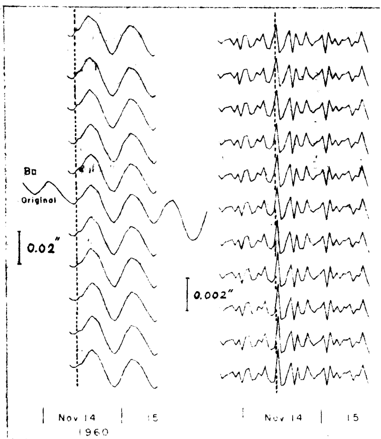
Fig. 33. Stepped tiltgrams at the time of the earthquake occurrence at 11h08m on Nov. 14, 1960, and their filtered results. Curves on the left are the original ( center ) and stepped tiltgrams, and curves on the right are filtered tiltgrams. The dashed line indicates the time of the earthquake occurrence and accordingly the time when the step was given.
