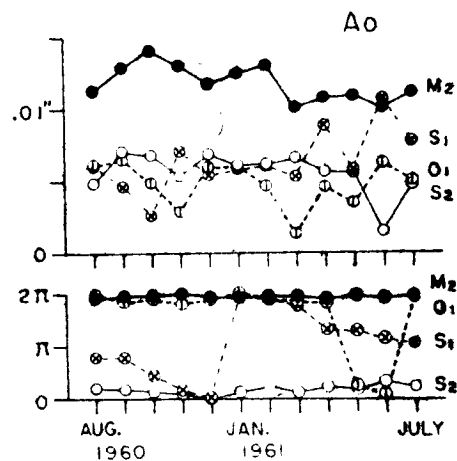
Fig. 9h. Amplitudes and phases of the E-W component tilt at Oura.
