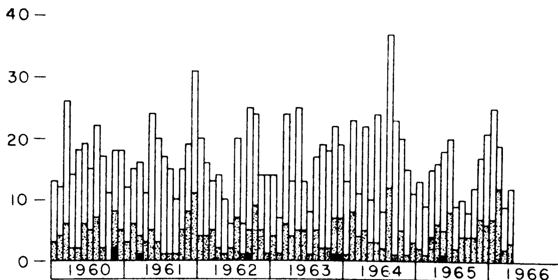
Fig. 7. Monthly numbers of earthquakes occurred near Wakayama City reported on the Seismological Bulletins of the JMA.
