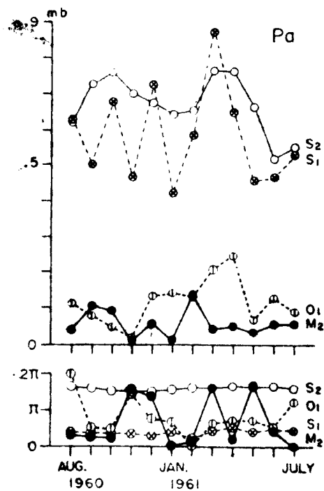
Fig. 9c. Amplitudes and phases of the atmospheric pressure observed at Akibasan.
