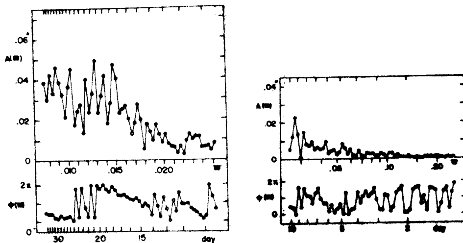
Fig. 20. Corrected amplitude and phase spectra of the E-W component tilt at Akibasan.
