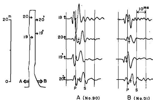
Fig. 16. Records obtained by the hammer blow. Phase of S wave is reversed by reverse of the blow direction.
