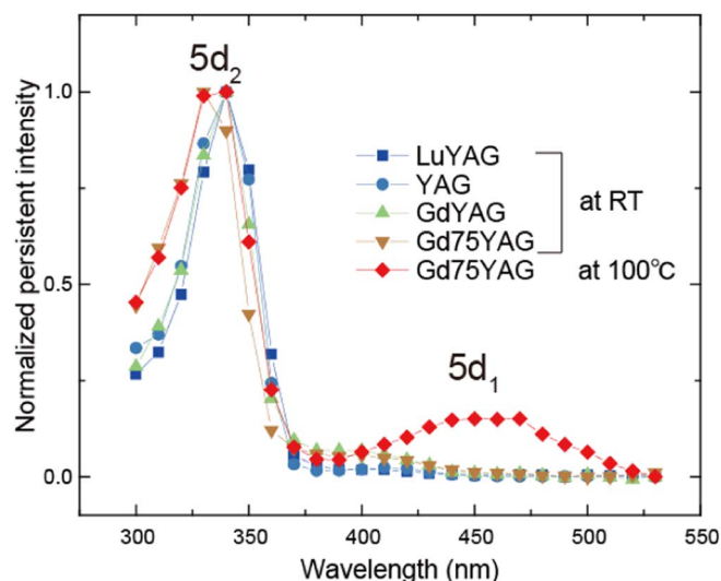
Figure 6. Persistent luminescence excitation (PersLE) spectra at room temperature in LuYAG, YAG, GdYAG and Gd75YAG doped with Ce 3+ and PersLE spectrum at 100°C in Gd75YAG.
