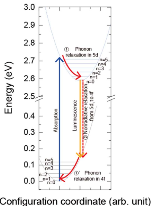
Figure 4. Schematic configuration coordinate diagram of \text{Ce}^{3+} -doped garnet.
