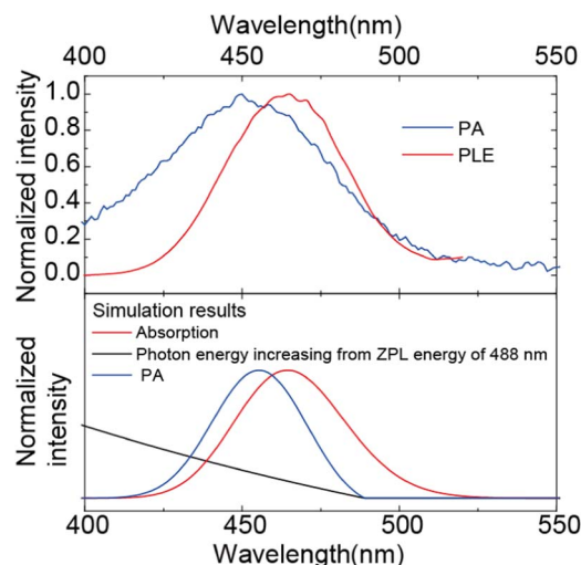
Figure 3. (a) Comparison of PLE and PA spectra in \text{YAG}:\text{Ce}^{3+} , and (b) simulation results of PA spectrum (blue solid line) estimated from the Gaussian type absorption spectra peaked at 460 nm and the change of photon energy from the ZPL energy of 488 nm.
