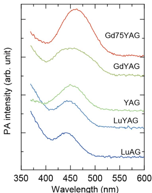
Figure 2. Photoacoustic spectra of \text{Ln}_3\text{Al}_5\text{O}_{12}:\text{Ce}^{3+} .
