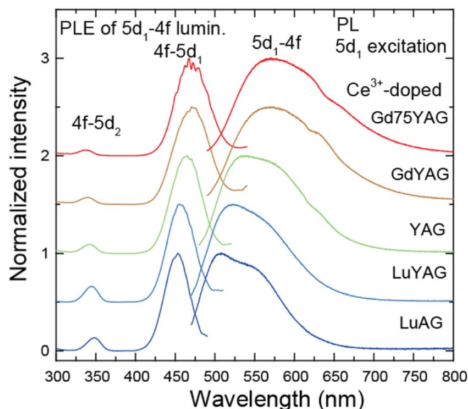
Figure 1. PL and PLE spectra of \text{Ln}_3\text{Al}_5\text{O}_{12}:\text{Ce}^{3+} .
